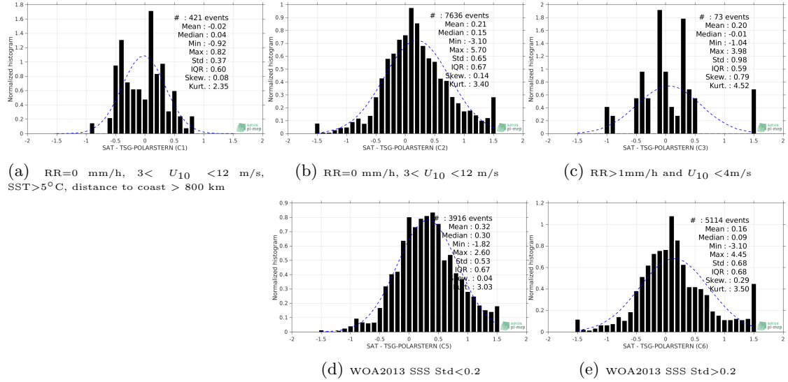
Figure 13: Normalized histogram of \Delta SSS (SMAP-L2-RSS-V4 - TSG-POLARSTERN) for 5 different subdatasets corresponding to: RR=0 mm/h, 3 < U_{10} < 12 m/s, SST > 5°C, distance to coast > 800 km (a), RR=0 mm/h, 3 < U_{10} < 12 m/s (b), RR > 1mm/h and U_{10} < 4 m/s (c), WOA2013 SSS Std < 0.2 (d), WOA2013 SSS Std > 0.2 (e).
