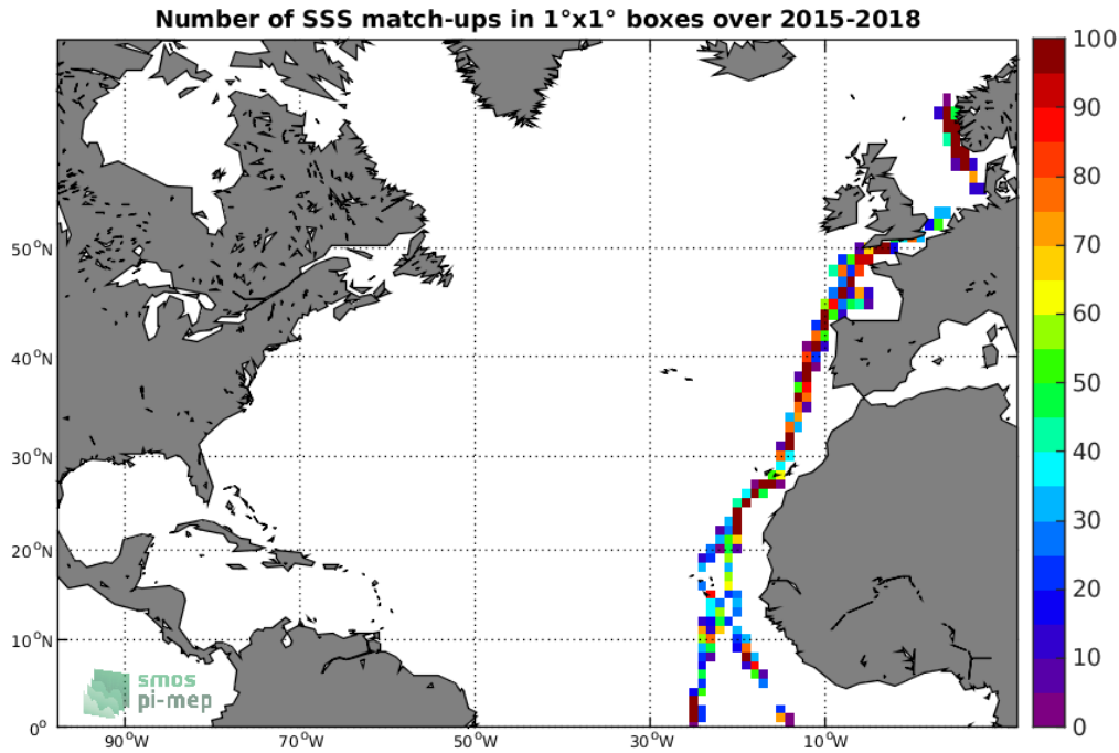
Figure 4: Number of SSS match-ups between TSG-POLARSTERN SSS and the SMAP-L2-RSS-V4 SSS product for the North Atlantic Ocean Pi-MEP region over 1^\circ \times 1^\circ boxes and for the full satellite product period.
