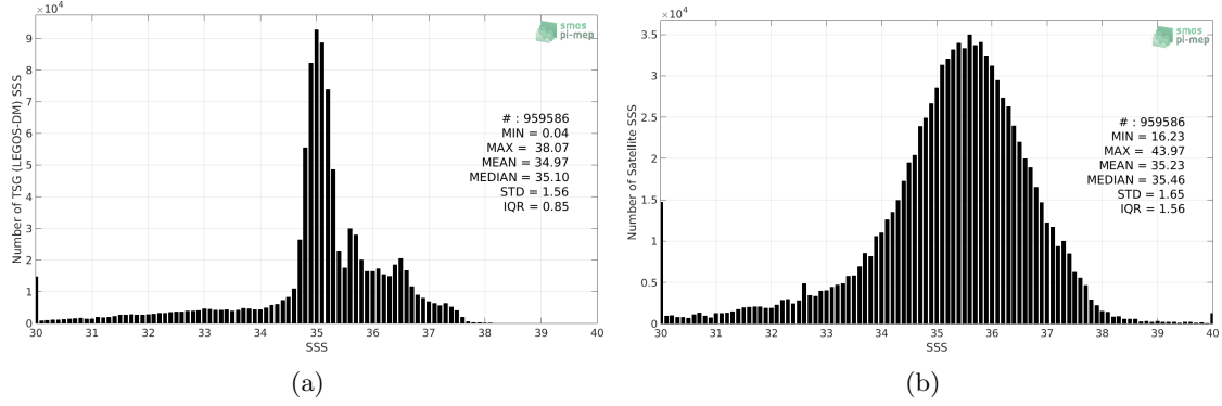
Figure 2: Histograms of SSS from TSG (LEGOS-DM) (a) and SMAP SSS L2 v4 (RSS) (b) considering all match-up pairs per bins of 0.1 over the North Atlantic Ocean Pi-MEP region and for the full satellite product period.
