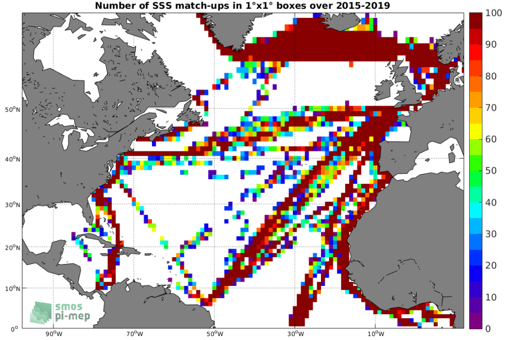
Figure 4: Number of SSS match-ups between TSG (LEGOS-DM) SSS and the SMAP SSS L2 v4 (RSS) SSS product for the North Atlantic Ocean Pi-MEP region over 1^\circ \times 1^\circ boxes and for the full satellite product period.
