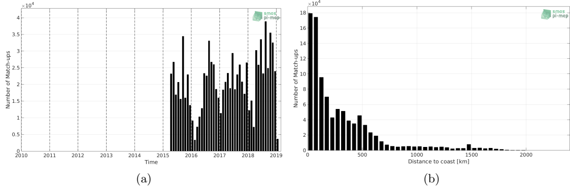
Figure 1: Number of match-ups between TSG (LEGOS-DM) and SMAP SSS L2 v4 (RSS) SSS as a function of time (a) and as function of the distance to coast (b) over the North Atlantic Ocean Pi-MEP region and for the full satellite product period.
