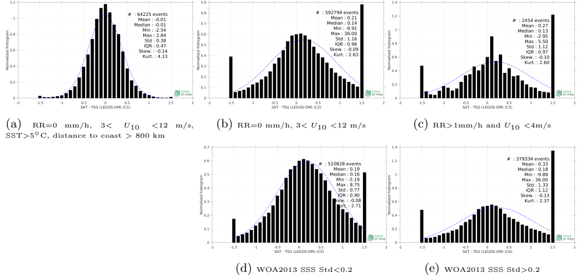
Figure 13: Normalized histogram of \Delta\text{SSS} (SMAP SSS L2 v4 (RSS) - TSG (LEGOS-DM)) for 5 different subdatasets corresponding to: RR=0 mm/h, 3 < U_{10} < 12 m/s, SST>5°C, distance to coast > 800 km (a), RR=0 mm/h, 3 < U_{10} < 12 m/s (b), RR>1mm/h and U_{10} < 4 m/s (c), WOA2013 SSS Std<0.2 (d), WOA2013 SSS Std>0.2 (e).
