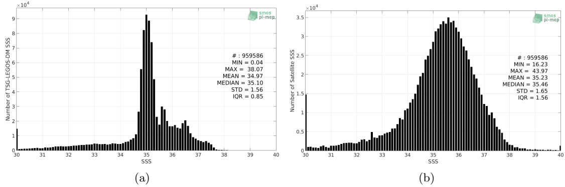
Figure 2: Histograms of SSS from TSG-LEGOS-DM (a) and SMAP-L2-RSS-V4 (b) considering all match-up pairs per bins of 0.1 over the North Atlantic Ocean Pi-MEP region and for the full satellite product period.
