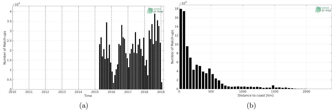
Figure 1: Number of match-ups between TSG-LEGOS-DM and SMAP-L2-RSS-V4 SSS as a function of time (a) and as function of the distance to coast (b) over the North Atlantic Ocean Pi-MEP region and for the full satellite product period.
