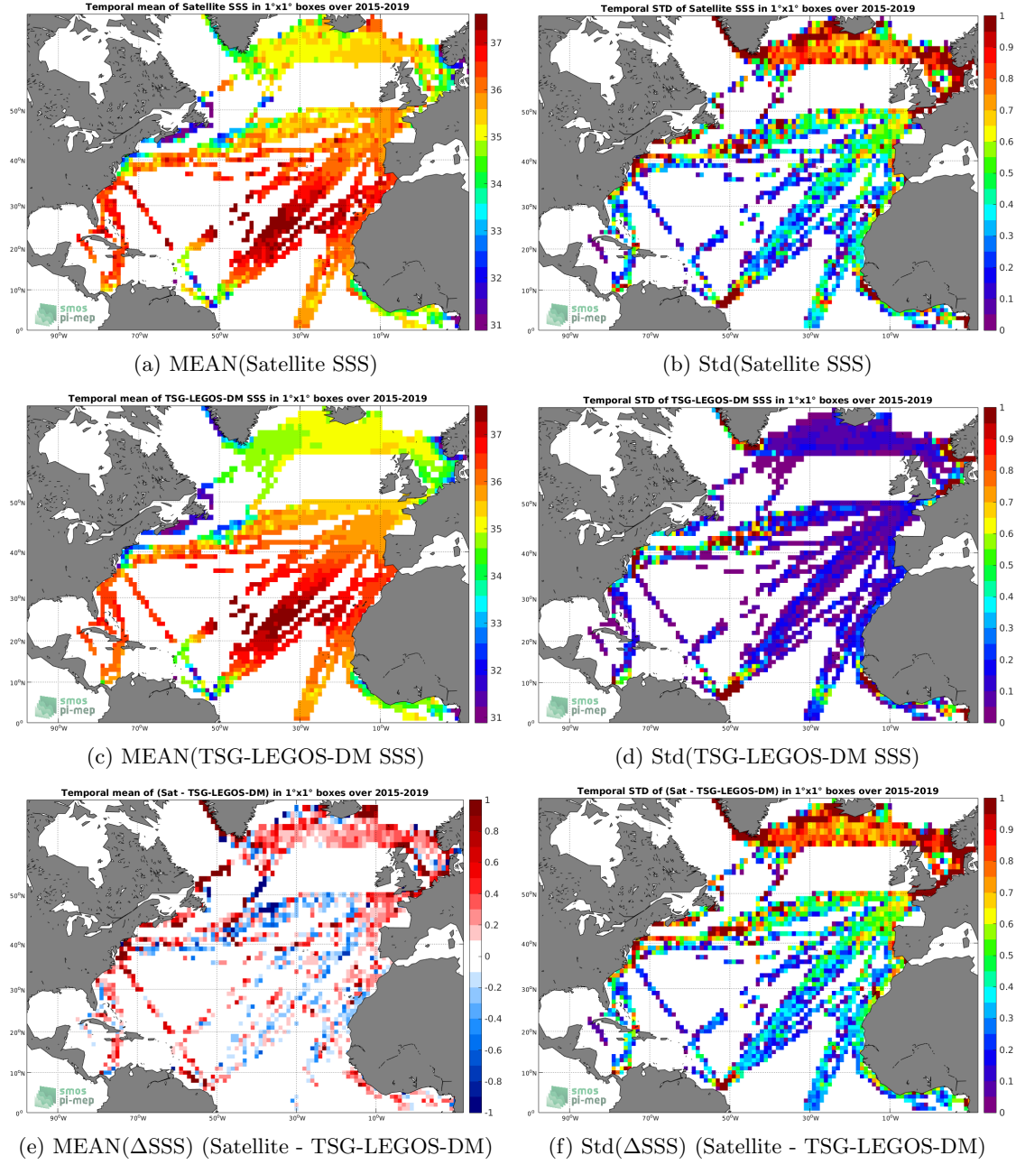
Figure 6: Temporal mean (left) and Std (right) of SSS from SMAP-L2-RSS-V4 (top), TSG-LEGOS-DM (middle), and of \Delta SSS (Satellite - TSG-LEGOS-DM). Only match-up pairs are used to generate these maps.
