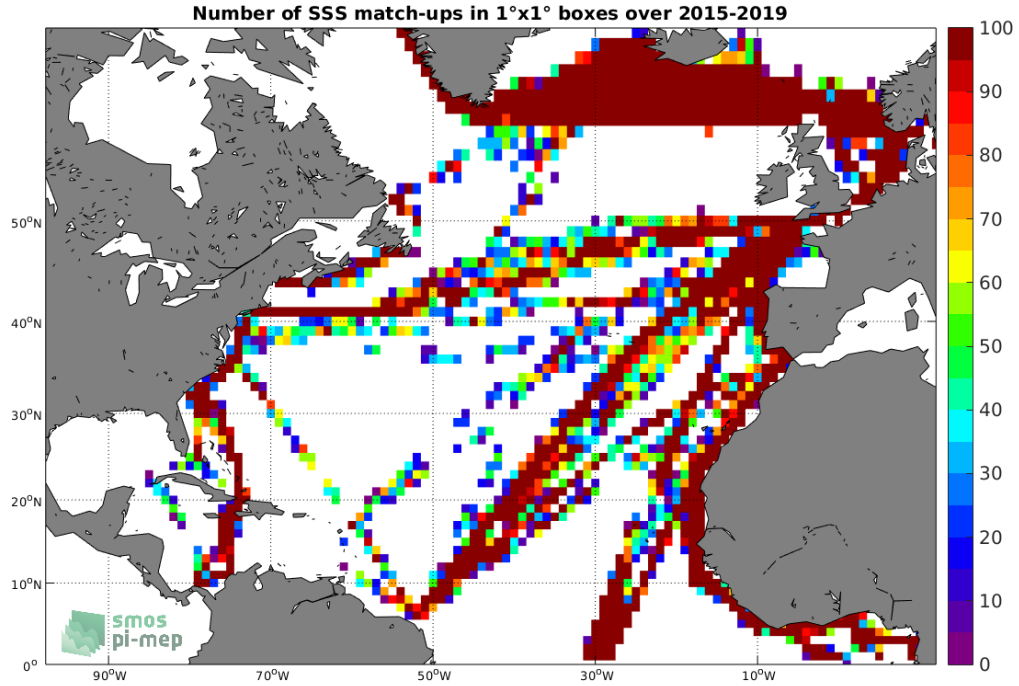
Figure 4: Number of SSS match-ups between TSG-LEGOS-DM SSS and the SMAP-L2-RSS-V4 SSS product for the North Atlantic Ocean Pi-MEP region over 1^\circ \times 1^\circ boxes and for the full satellite product period.
