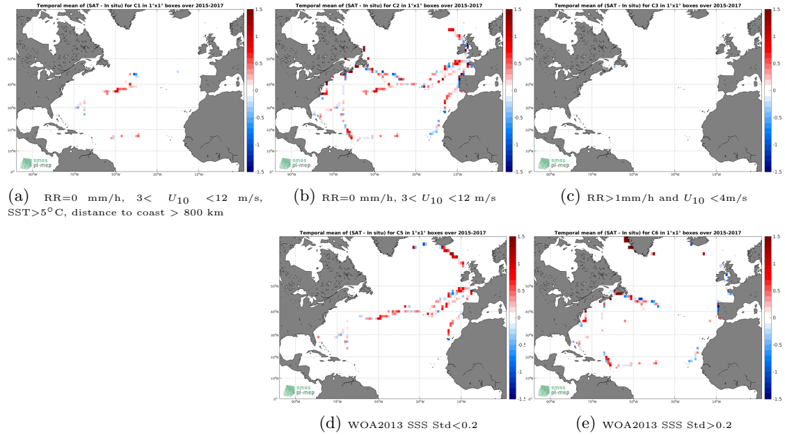
Figure 12: Temporal mean gridded over spatial boxes of size 1^\circ \times 1^\circ of \Delta SSS (SMAP SSS L2 v4 (RSS) - TSG (GOSUD-Sailing-ship)) for 5 different subdatasets corresponding to: RR=0 mm/h, 3 < U_{10} < 12 m/s, SST>5°C, distance to coast > 800 km (a), RR=0 mm/h, 3 < U_{10} < 12 m/s (b), RR>1mm/h and U_{10} < 4 m/s (c), WOA2013 SSS Std<0.2 (d), WOA2013 SSS Std>0.2 (e).
