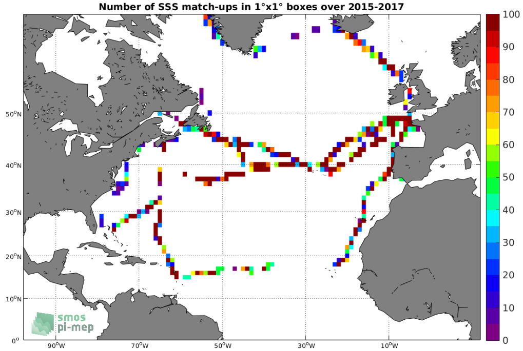
Figure 4: Number of SSS match-ups between TSG (GOSUD-Sailing-ship) SSS and the SMAP SSS L2 v4 (RSS) SSS product for the North Atlantic Ocean Pi-MEP region over 1^\circ \times 1^\circ boxes and for the full satellite product period.
