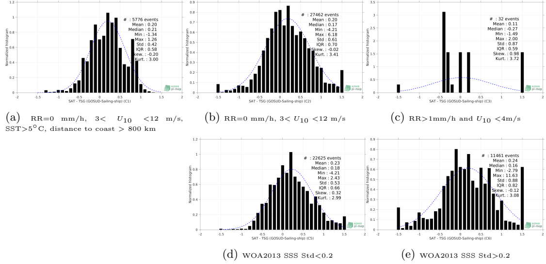
Figure 13: Normalized histogram of \Delta\text{SSS} (SMAP SSS L2 v4 (RSS) - TSG (GOSUD-Sailing-ship)) for 5 different subdatasets corresponding to: RR=0 mm/h, 3 < U_{10} < 12 m/s, SST>5°C, distance to coast > 800 km (a), RR=0 mm/h, 3 < U_{10} < 12 m/s (b), RR>1mm/h and U_{10} < 4 m/s (c), WOA2013 SSS Std<0.2 (d), WOA2013 SSS Std>0.2 (e).
