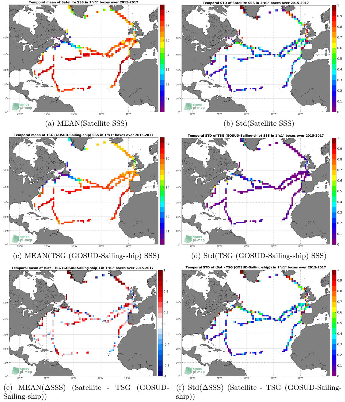
Figure 6: Temporal mean (left) and Std (right) of SSS from SMAP SSS L2 v4 (RSS) (top), TSG (GOSUD-Sailing-ship) (middle), and of \Delta SSS (Satellite - TSG (GOSUD-Sailing-ship)). Only match-up pairs are used to generate these maps.
