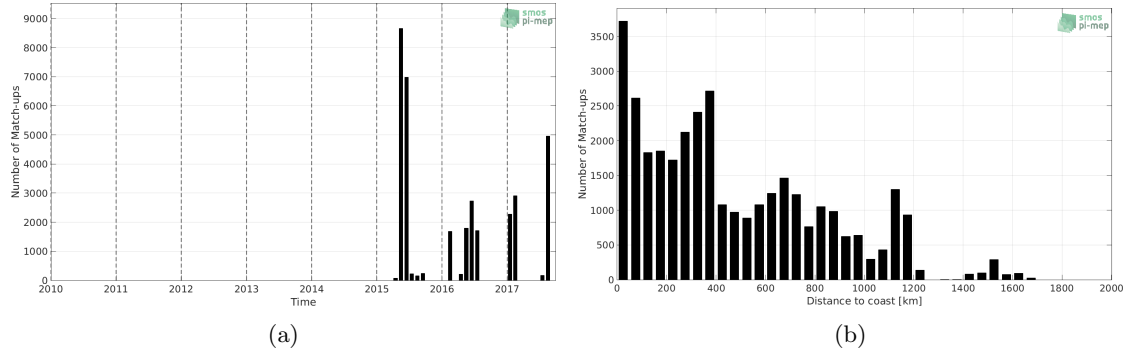
Figure 1: Number of match-ups between TSG (GOSUD-Sailing-ship) and SMAP SSS L2 v4 (RSS) SSS as a function of time (a) and as function of the distance to coast (b) over the North Atlantic Ocean Pi-MEP region and for the full satellite product period.
