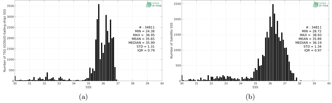
Figure 2: Histograms of SSS from TSG (GOSUD-Sailing-ship) (a) and SMAP SSS L2 v4 (RSS) (b) considering all match-up pairs per bins of 0.1 over the North Atlantic Ocean Pi-MEP region and for the full satellite product period.
