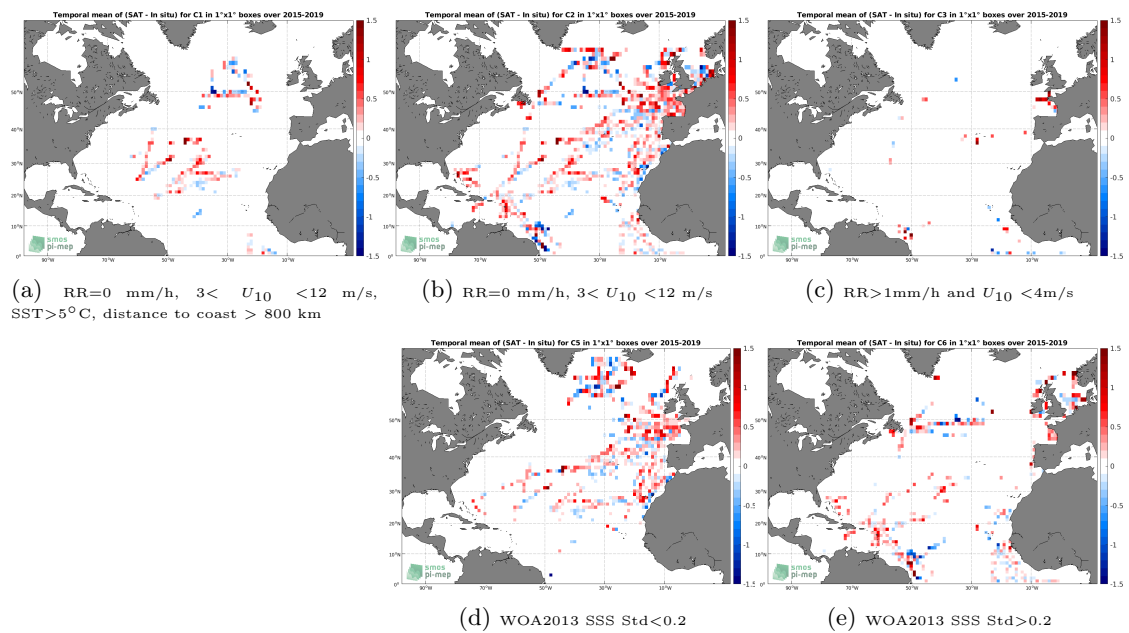
Figure 12: Temporal mean gridded over spatial boxes of size 1°x1° of \Delta SSS (SMAP SSS L2 v4 (RSS) - TSG (GOSUD-Research-vessel)) for 5 different subdatasets corresponding to:RR=0 mm/h, 3 < U_{10} < 12 m/s, SST>5°C, distance to coast > 800 km (a), RR=0 mm/h, 3 < U_{10} < 12 m/s (b), RR>1mm/h and U_{10} < 4 m/s (c), WOA2013 SSS Std<0.2 (d), WOA2013 SSS Std>0.2 (e).
