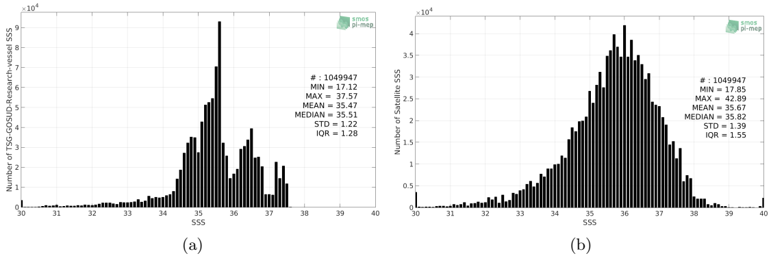
Figure 2: Histograms of SSS from TSG-GOSUD-Research-vessel (a) and SMAP-L2-RSS-V4 (b) considering all match-up pairs per bins of 0.1 over the North Atlantic Ocean Pi-MEP region and for the full satellite product period.
