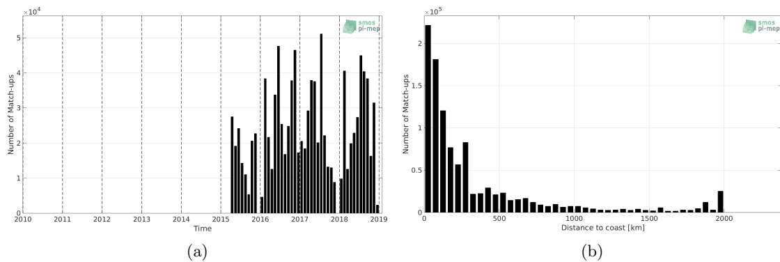
Figure 1: Number of match-ups between TSG-GOSUD-Research-vessel and SMAP-L2-RSS-V4 SSS as a function of time (a) and as function of the distance to coast (b) over the North Atlantic Ocean Pi-MEP region and for the full satellite product period.
