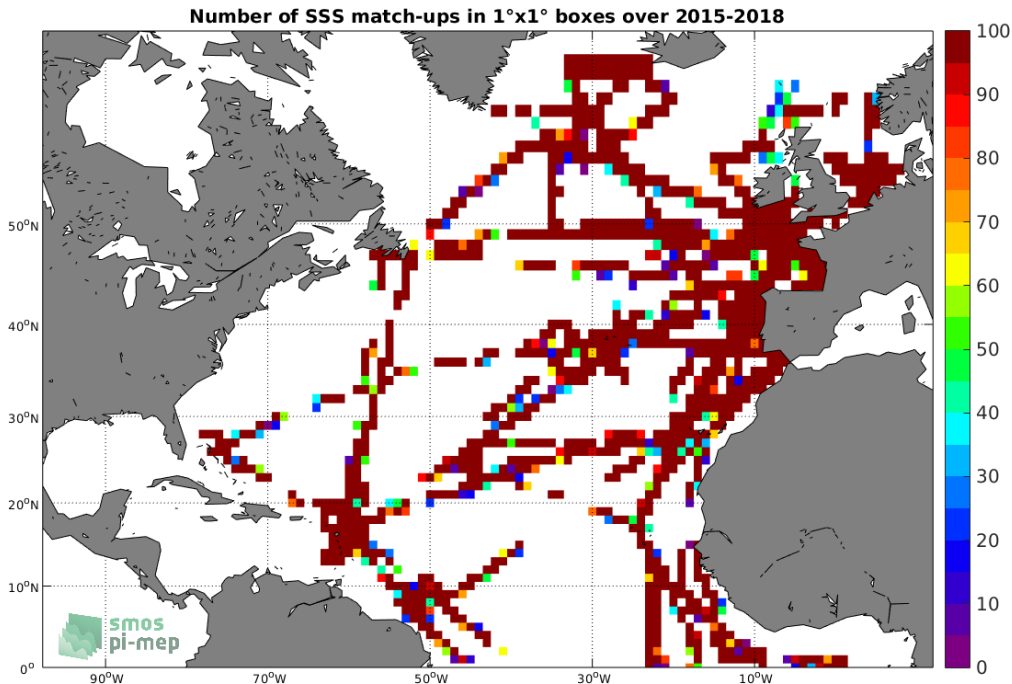
Figure 4: Number of SSS match-ups between TSG-GOSUD-Research-vessel SSS and the SMAP-L2-RSS-V4 SSS product for the North Atlantic Ocean Pi-MEP region over 1°x1° boxes and for the full satellite product period.
