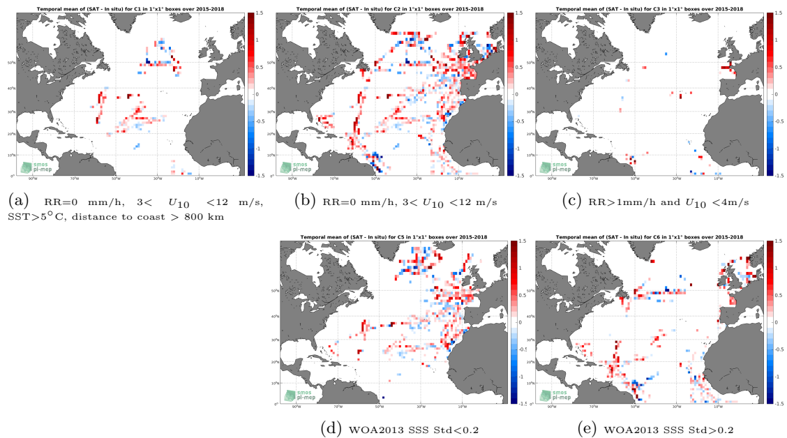
Figure 12: Temporal mean gridded over spatial boxes of size 1^\circ \times 1^\circ of \Delta SSS (SMAP-L2-RSS-V4 - TSG-GOSUD-Research-vessel) for 5 different subdatasets corresponding to:RR=0 mm/h, 3 < U_{10} < 12 m/s, SST > 5^\circ\text{C} , distance to coast > 800 km (a), RR=0 mm/h, 3 < U_{10} < 12 m/s (b), RR > 1 mm/h and U_{10} < 4 m/s (c), WOA2013 SSS Std < 0.2 (d), WOA2013 SSS Std > 0.2 (e).
