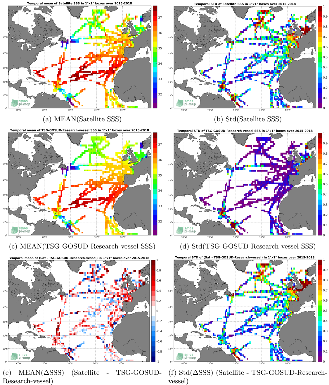
Figure 6: Temporal mean (left) and Std (right) of SSS from SMAP-L2-RSS-V4 (top), TSG-GOSUD-Research-vessel (middle), and of \Delta SSS (Satellite - TSG-GOSUD-Research-vessel). Only match-up pairs are used to generate these maps.
