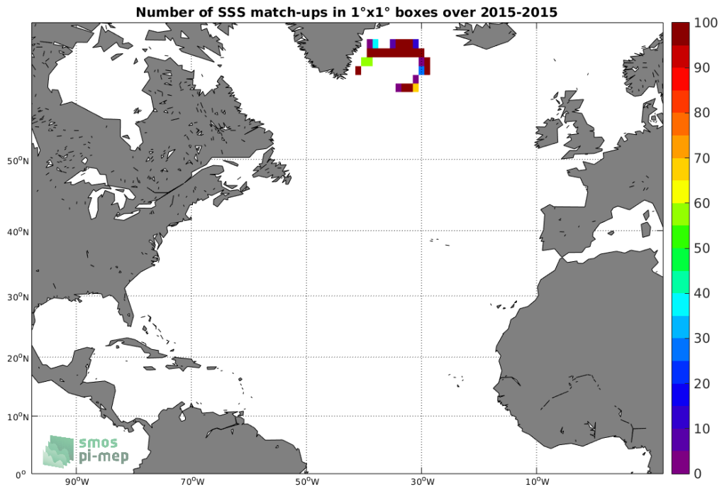
Figure 3: Number of SSS match-ups between Surface drifters SSS and the SMAP-L2-RSS-V4 SSS product for the North Atlantic Ocean Pi-MEP region over 1°x1° boxes and for the full satellite product period.
