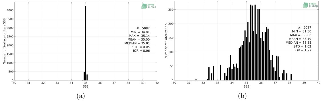
Figure 2: Histograms of SSS from Surface drifters (a) and SMAP-L2-RSS-V4 (b) considering all match-up pairs per bins of 0.1 over the North Atlantic Ocean Pi-MEP region and for the full satellite product period.
