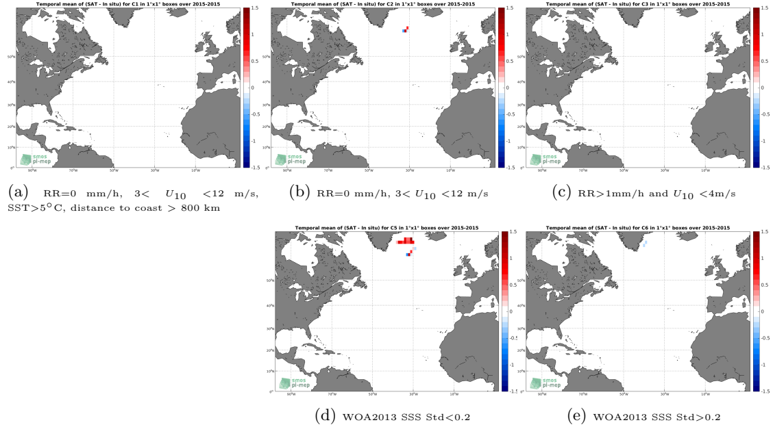
Figure 11: Temporal mean gridded over spatial boxes of size 1^{\circ}\times 1^{\circ} of \Delta\text{SSS} (SMAP-L2-RSS-V4 - Surface drifters) for 5 different subdatasets corresponding to: RR=0 mm/h, 3 < U_{10} < 12 m/s, SST >5^{\circ}\text{C} , distance to coast > 800 km (a), RR=0 mm/h, 3 < U_{10} < 12 m/s (b), RR >1 mm/h and U_{10} < 4 m/s (c), WOA2013 SSS Std <0.2 (d), WOA2013 SSS Std >0.2 (e).
