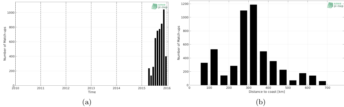
Figure 1: Number of match-ups between Surface drifters and SMAP-L2-RSS-V4 SSS as a function of time (a) and as function of the distance to coast (b) over the North Atlantic Ocean Pi-MEP region and for the full satellite product period.
