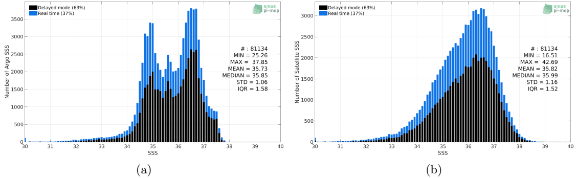
Figure 2: Histograms of SSS from Argo (a) and SMAP SSS L2 v4 (RSS) (b) considering all match-up pairs per bins of 0.1 over the North Atlantic Ocean Pi-MEP region and for the full satellite product period.
