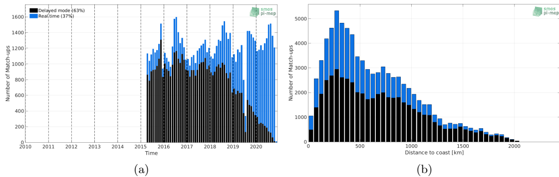
Figure 1: Number of match-ups between Argo and SMAP SSS L2 v4 (RSS) SSS as a function of time (a) and as function of the distance to coast (b) over the North Atlantic Ocean Pi-MEP region and for the full satellite product period.
