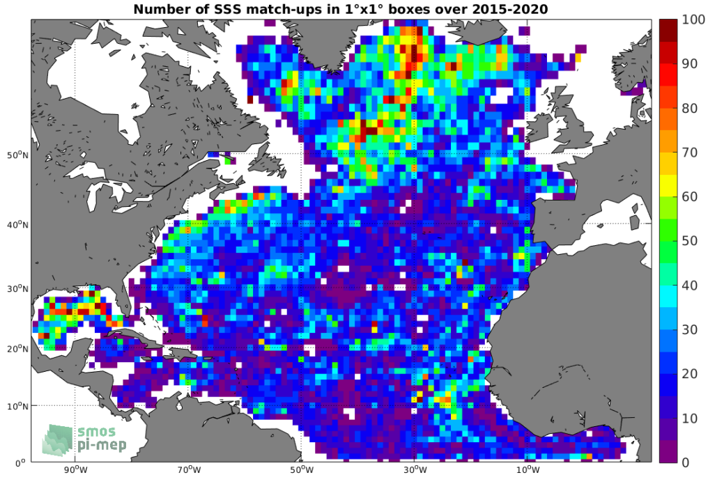
Figure 4: Number of SSS match-ups between Argo SSS and the SMAP SSS L2 v4 (RSS) SSS product for the North Atlantic Ocean Pi-MEP region over 1^\circ \times 1^\circ boxes and for the full satellite product period.
