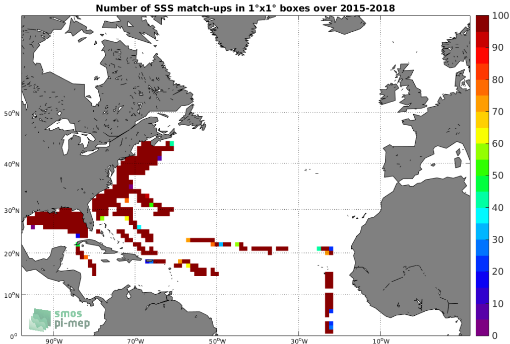
Figure 4: Number of SSS match-ups between TSG-SAMOS SSS and the SMAP-L2-RSS-V3-70KM SSS product for the North Atlantic Ocean Pi-MEP region over 1°x1° boxes and for the full satellite product period.
