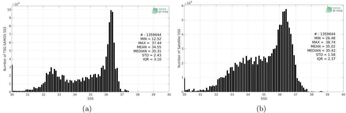
Figure 2: Histograms of SSS from TSG-SAMOS (a) and SMAP-L2-RSS-V3-70KM (b) considering all match-up pairs per bins of 0.1 over the North Atlantic Ocean Pi-MEP region and for the full satellite product period.
