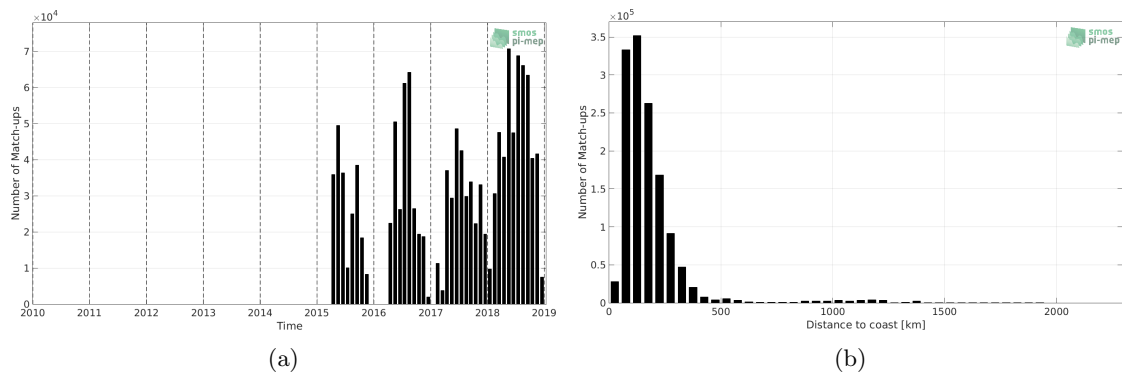
Figure 1: Number of match-ups between TSG-SAMOS and SMAP-L2-RSS-V3-70KM SSS as a function of time (a) and as function of the distance to coast (b) over the North Atlantic Ocean Pi-MEP region and for the full satellite product period.
