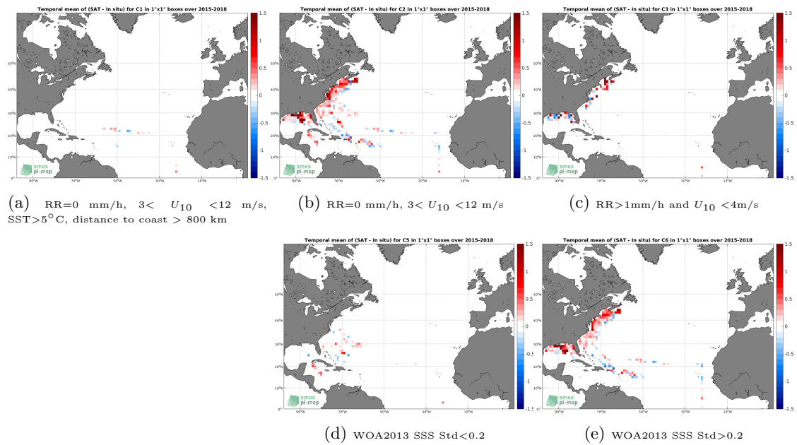
Figure 12: Temporal mean gridded over spatial boxes of size 1^\circ \times 1^\circ of \Delta SSS (SMAP-L2-RSS-V3-70KM - TSG-SAMOS) for 5 different subdatasets corresponding to:RR=0 mm/h, 3 < U_{10} < 12 m/s, SST >5^\circ C, distance to coast > 800 km (a), RR=0 mm/h, 3 < U_{10} < 12 m/s (b), RR >1 mm/h and U_{10} < 4 m/s (c), WOA2013 SSS Std <0.2 (d), WOA2013 SSS Std >0.2 (e).
