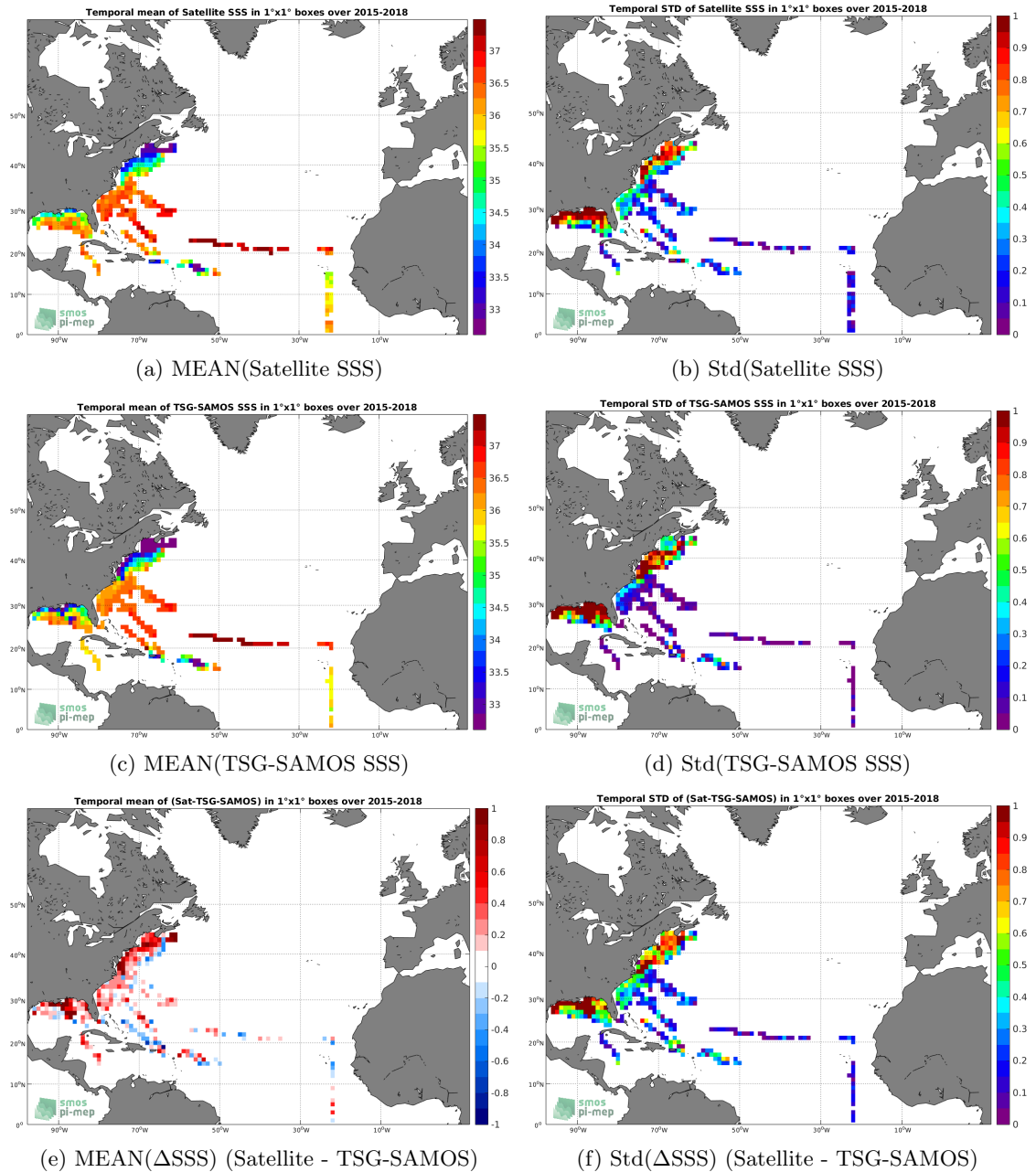
Figure 6: Temporal mean (left) and Std (right) of SSS from SMAP-L2-RSS-V3-70KM (top), TSG-SAMOS (middle), and of \Delta SSS (Satellite - TSG-SAMOS). Only match-up pairs are used to generate these maps.
