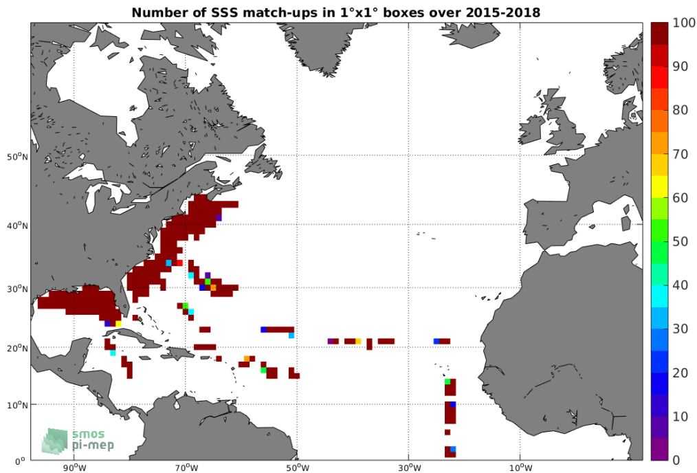
Figure 4: Number of SSS match-ups between TSG-SAMOS SSS and the SMAP-L2-RSS-V3-70KM SSS product for the North Atlantic Ocean Pi-MEP region over 1^\circ \times 1^\circ boxes and for the full satellite product period.
