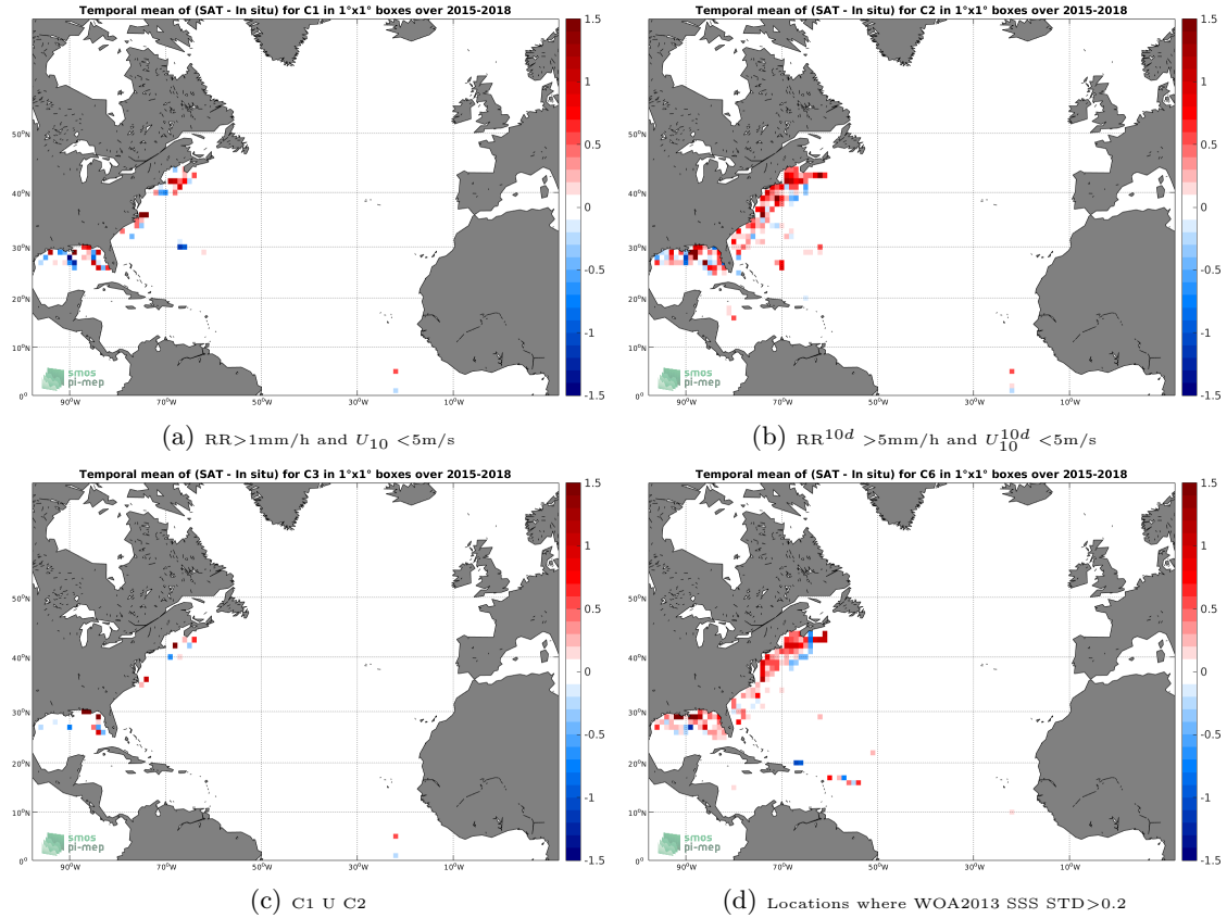
Figure 12: Temporal mean gridded over spatial boxes of size 1^\circ \times 1^\circ of \Delta SSS (SMAP-L2-RSS-V3-70KM - TSG-SAMOS) for 4 different subdatasets corresponding to: RR > 1 mm/h and U_{10} < 5 m/s (a), RR 10d > 5 mm/h and U_{10}^{10d} < 5 m/s (b), C1 U C2 (c), Locations where WOA2013 SSS STD > 0.2 (d).
