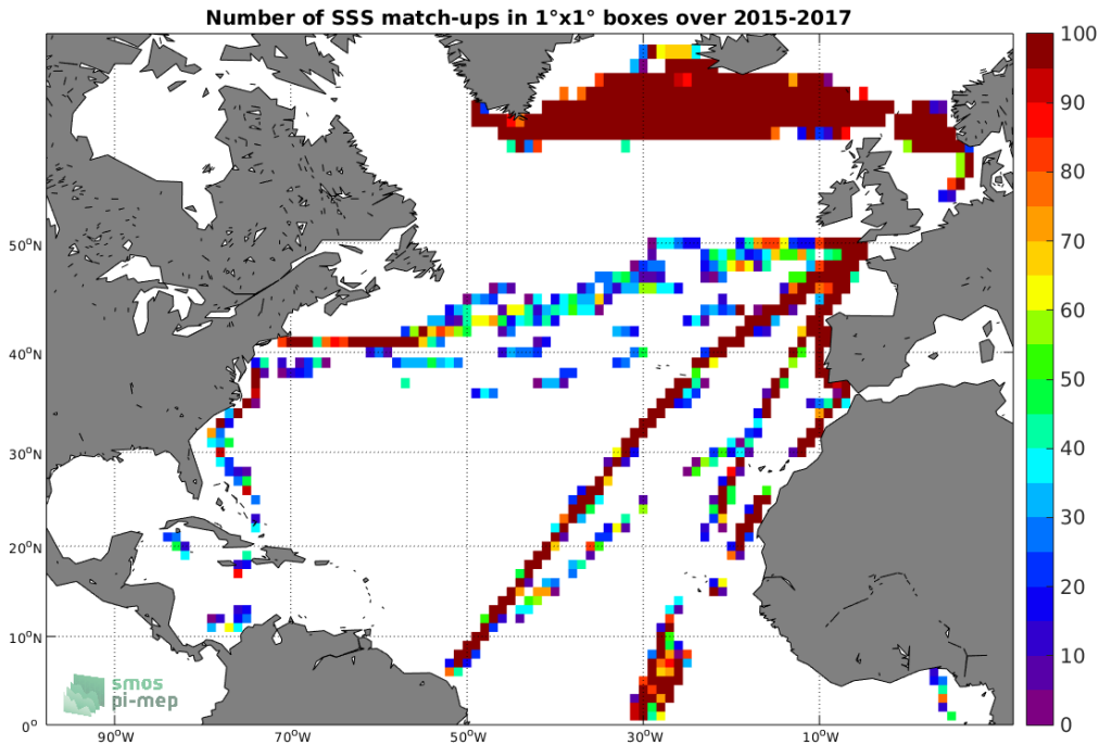
Figure 4: Number of SSS match-ups between TSG-LEGOS-DM SSS and the SMAP-L2-RSS-V3-70KM SSS product for the North Atlantic Ocean Pi-MEP region over 1^\circ \times 1^\circ boxes and for the full satellite product period.
