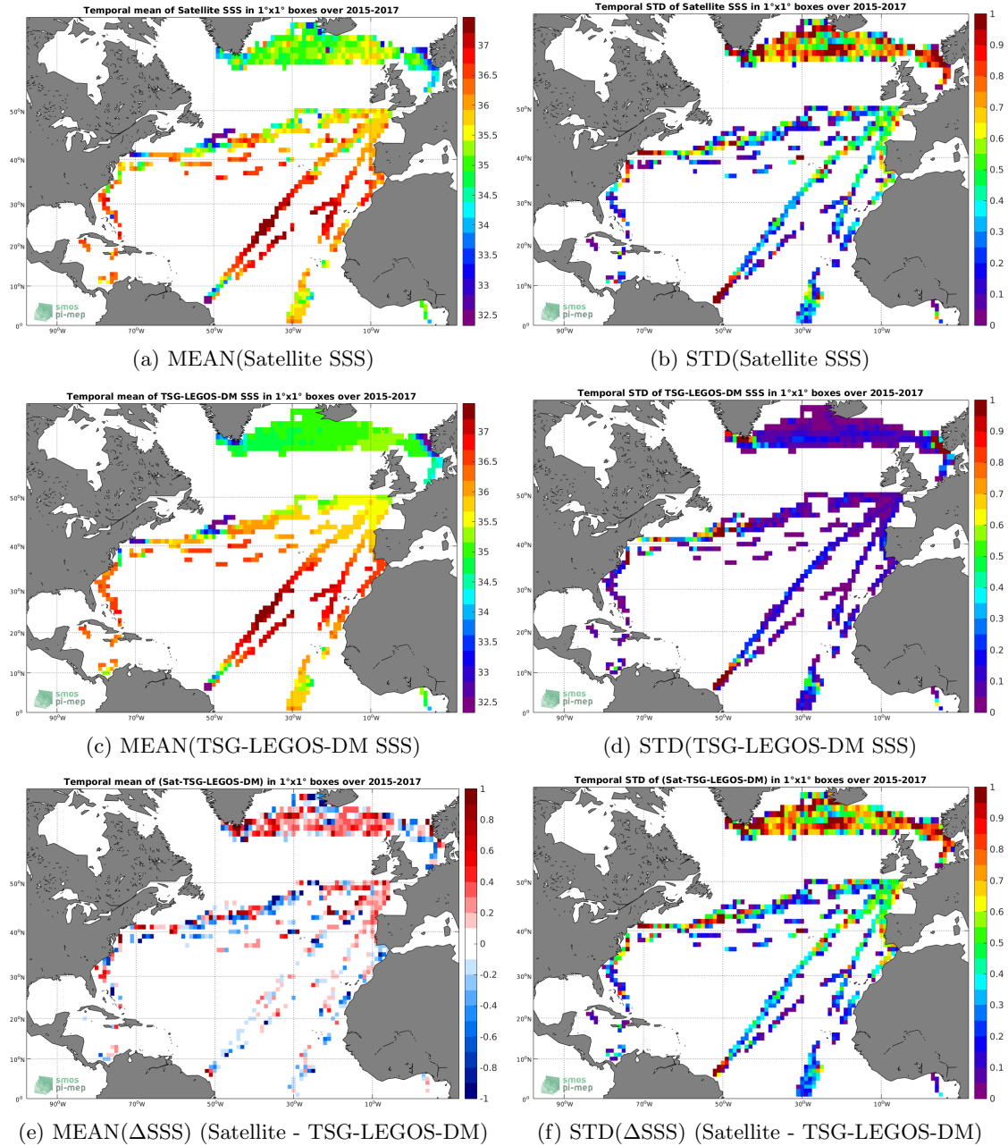
Figure 6: Temporal mean (left) and STD (right) of SSS from SMAP-L2-RSS-V3-70KM (top), TSG-LEGOS-DM (middle), and of \Delta SSS (Satellite - TSG-LEGOS-DM). Only match-up pairs are used to generate these maps.
