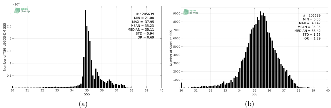
Figure 2: Histograms of SSS from TSG-LEGOS-DM (a) and SMAP-L2-RSS-V3-70KM (b) considering all match-up pairs per bins of 0.1 over the North Atlantic Ocean Pi-MEP region and for the full satellite product period.
