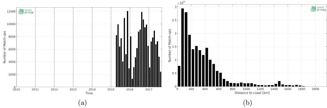
Figure 1: Number of match-ups between TSG-LEGOS-DM and SMAP-L2-RSS-V3-70KM SSS as a function of time (a) and as function of the distance to coast (b) over the North Atlantic Ocean Pi-MEP region and for the full satellite product period.
