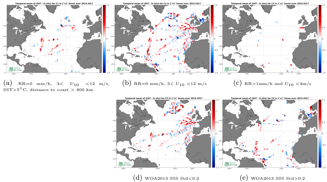
Figure 12: Temporal mean gridded over spatial boxes of size 1^\circ \times 1^\circ of \Delta SSS (SMAP-L2-RSS-V3-70KM - TSG-GOSUD-Research-vessel) for 5 different subdatasets corresponding to:RR=0 mm/h, 3 < U_{10} < 12 m/s, SST >5^\circ C, distance to coast > 800 km (a), RR=0 mm/h, 3 < U_{10} < 12 m/s (b), RR >1 mm/h and U_{10} < 4 m/s (c), WOA2013 SSS Std <0.2 (d), WOA2013 SSS Std >0.2 (e).
