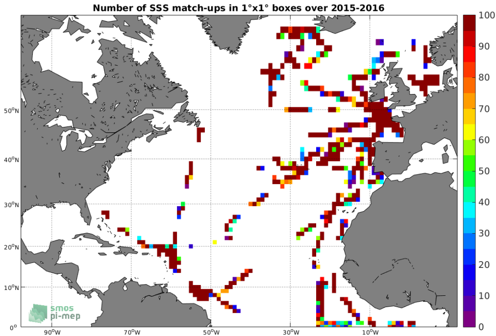
Figure 4: Number of SSS match-ups between TSG-GOSUD-Research-vessel SSS and the SMAP-L2-RSS-V3-70KM SSS product for the North Atlantic Ocean Pi-MEP region over 1^\circ \times 1^\circ boxes and for the full satellite product period.
