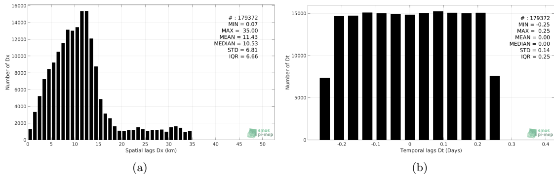
Figure 5: Histograms of the spatial (a) and temporal (b) lags between the time of the TSG-GOSUD-Research-vessel measurements and the date of the corresponding SMAP-L2-RSS-V3-70KM SSS product.
