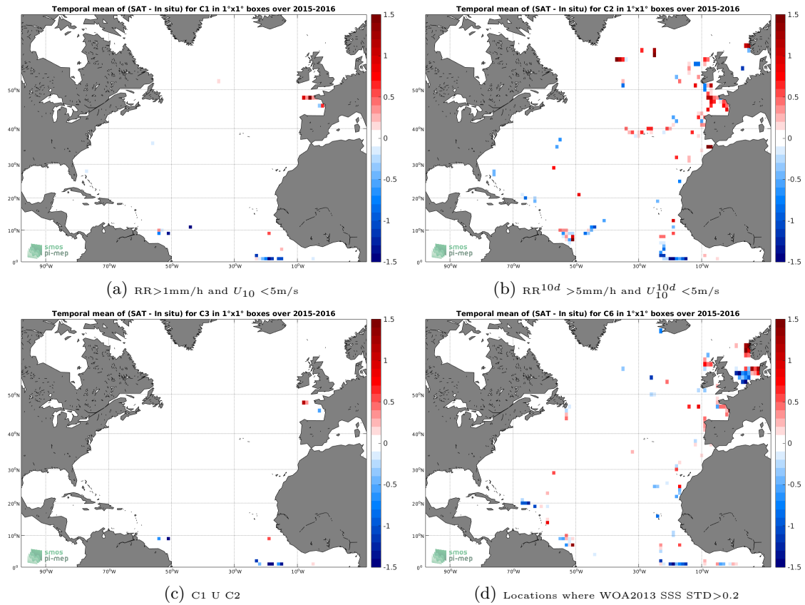
Figure 12: Temporal mean gridded over spatial boxes of size 1^\circ \times 1^\circ of \Delta SSS (SMAP-L2-RSS-V3-70KM - TSG-GOSUD-Research-vessel) for 4 different subdatasets corresponding to: RR > 1mm/h and U_{10} < 5\text{m/s} (a), RR^{10d} > 5\text{mm/h} and U_{10}^{10d} < 5\text{m/s} (b), C1 U C2 (c), Locations where WOA2013 SSS STD > 0.2 (d).
