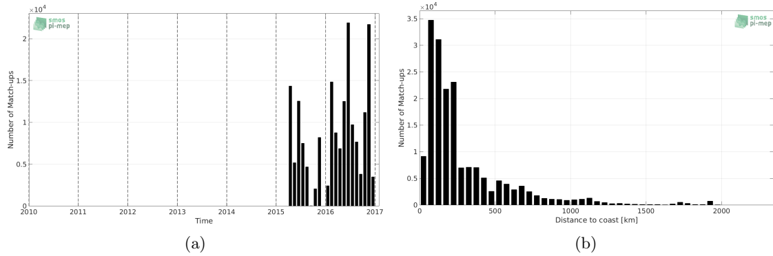
Figure 1: Number of match-ups between TSG-GOSUD-Research-vessel and SMAP-L2-RSS-V3-70KM SSS as a function of time (a) and as function of the distance to coast (b) over the North Atlantic Ocean Pi-MEP region and for the full satellite product period.
