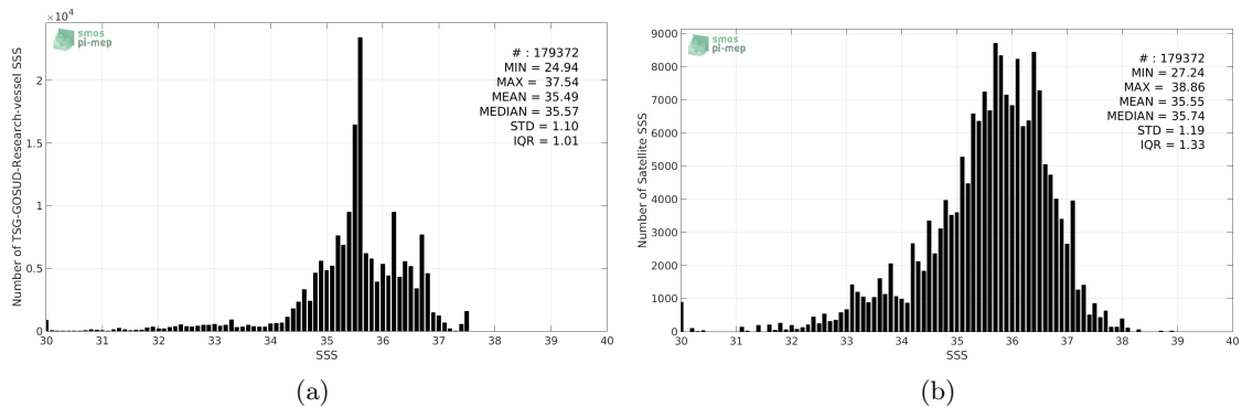
Figure 2: Histograms of SSS from TSG-GOSUD-Research-vessel (a) and SMAP-L2-RSS-V3-70KM (b) considering all match-up pairs per bins of 0.1 over the North Atlantic Ocean Pi-MEP region and for the full satellite product period.
