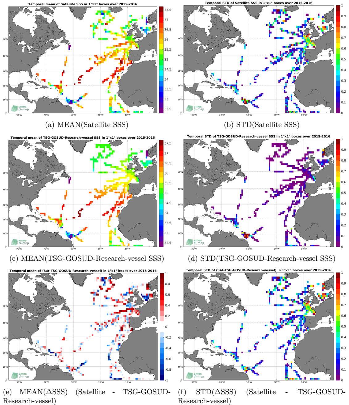
Figure 6: Temporal mean (left) and STD (right) of SSS from SMAP-L2-RSS-V3-70KM (top), TSG-GOSUD-Research-vessel (middle), and of \Delta SSS (Satellite - TSG-GOSUD-Research-vessel). Only match-up pairs are used to generate these maps.
