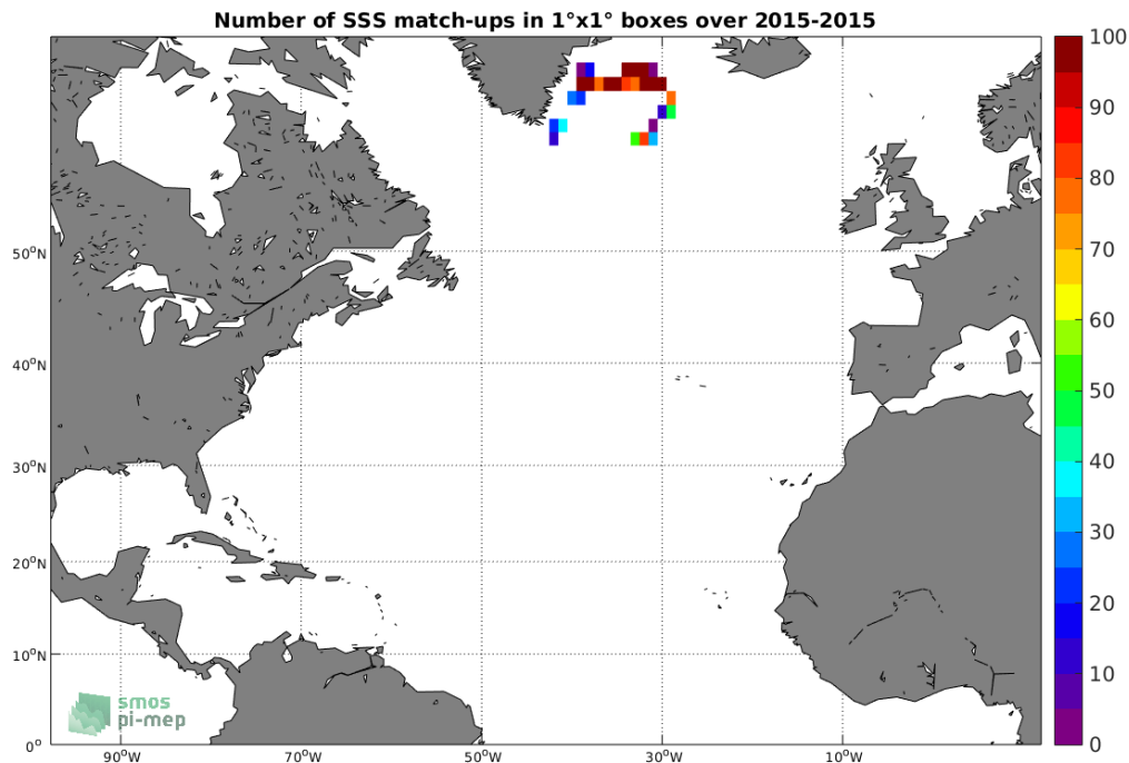
Figure 3: Number of SSS match-ups between Surface drifters SSS and the SMAP-L2-RSS-V3-70KM SSS product for the North Atlantic Ocean Pi-MEP region over 1°x1° boxes and for the full satellite product period.
