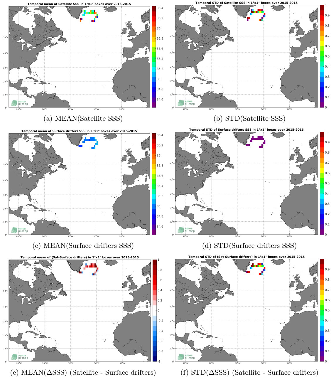
Figure 5: Temporal mean (left) and STD (right) of SSS from SMAP-L2-RSS-V3-70KM (top), Surface drifters (middle), and of \Delta SSS (Satellite - Surface drifters). Only match-up pairs are used to generate these maps.
