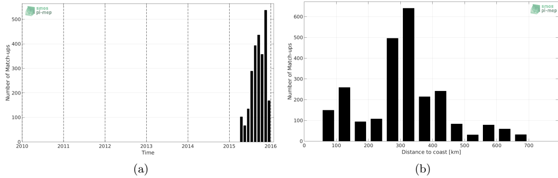
Figure 1: Number of match-ups between Surface drifters and SMAP-L2-RSS-V3-70KM SSS as a function of time (a) and as function of the distance to coast (b) over the North Atlantic Ocean Pi-MEP region and for the full satellite product period.
