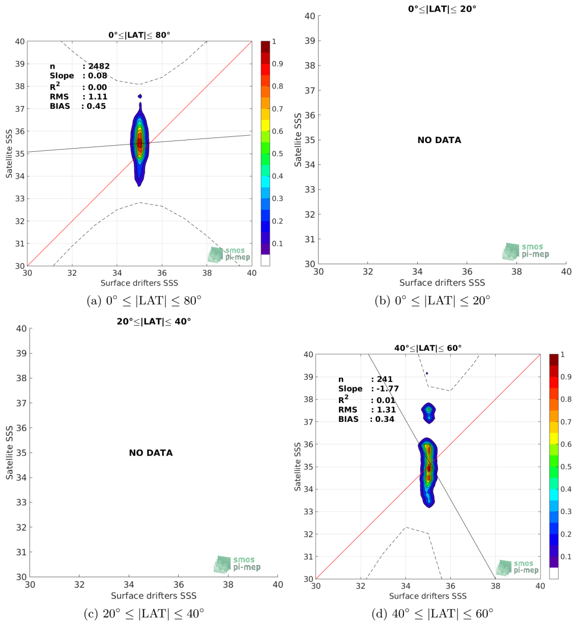
Figure 8: Contour maps of the concentration of SMAP-L2-RSS-V3-70KM SSS (y-axis) versus Surface drifters SSS (x-axis) at match-up pairs for different latitude bands. For each plot, the red line shows x=y . The black thin and dashed lines indicate a linear fit through the data cloud and the \pm 95\% confidence levels, respectively. The number match-up pairs n , the slope and R^2 coefficient of the linear fit, the root mean square (RMS) and the mean bias between satellite and in situ data are indicated for each latitude band in each plots.
