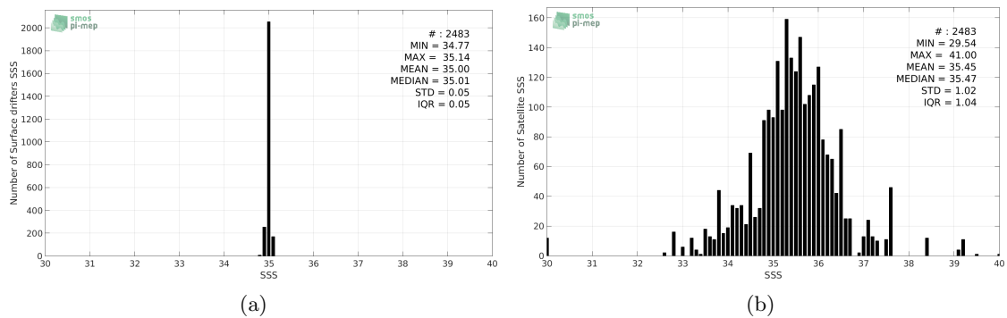
Figure 2: Histograms of SSS from Surface drifters (a) and SMAP-L2-RSS-V3-70KM (b) considering all match-up pairs per bins of 0.1 over the North Atlantic Ocean Pi-MEP region and for the full satellite product period.
