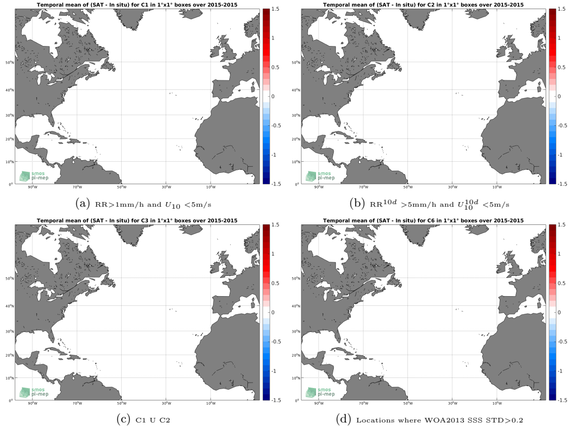
Figure 11: Temporal mean gridded over spatial boxes of size 1^\circ \times 1^\circ of \Delta SSS (SMAP-L2-RSS-V3-70KM - Surface drifters) for 4 different subdatasets corresponding to: RR > 1\text{mm/h} and U_{10} < 5\text{m/s} (a), RR^{10d} > 5\text{mm/h} and U_{10}^{10d} < 5\text{m/s} (b), C1 U C2 (c), Locations where WOA2013 SSS STD > 0.2 (d).
