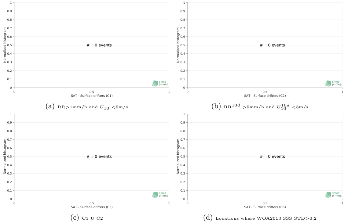
Figure 12: Normalized histogram of \Delta\text{SSS} (SMAP-L2-RSS-V3-70KM - Surface drifters) for 6 different subdatasets corresponding to: RR > 1\text{mm/h} and U_{10} < 5\text{m/s} (a), RR^{10d} > 5\text{mm/h} and U_{10}^{10d} < 5\text{m/s} (b), C1 \cup C2 (c), Locations where WOA2013 SSS STD > 0.2 (d).
