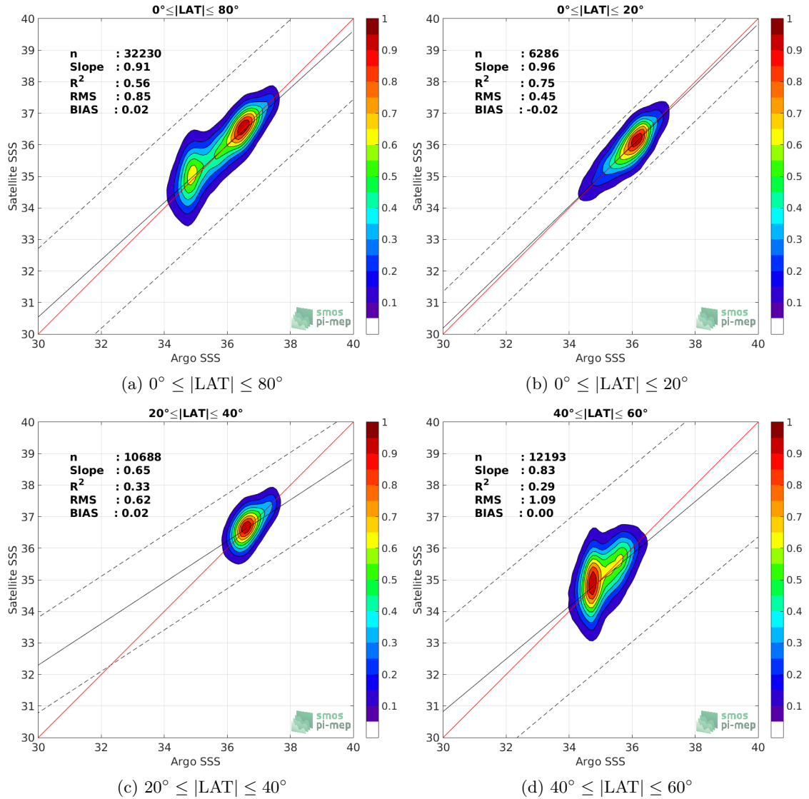
Figure 9: Contour maps of the concentration of SMAP-L2-RSS-V3-70KM SSS (y-axis) versus Argo SSS (x-axis) at match-up pairs for different latitude bands. For each plot, the red line shows x=y . The black thin and dashed lines indicate a linear fit through the data cloud and the \pm 95\% confidence levels, respectively. The number match-up pairs n , the slope and R^2 coefficient of the linear fit, the root mean square (RMS) and the mean bias between satellite and in situ data are indicated for each latitude band in each plots.
