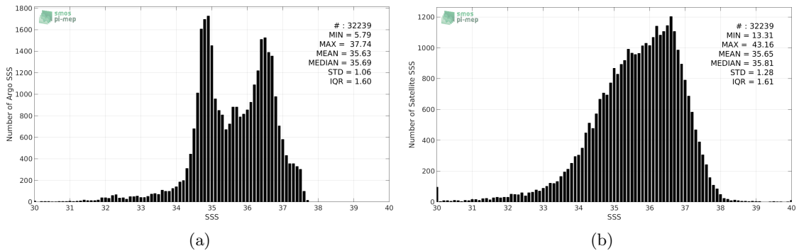
Figure 2: Histograms of SSS from Argo (a) and SMAP-L2-RSS-V3-70KM (b) considering all match-up pairs per bins of 0.1 over the North Atlantic Ocean Pi-MEP region and for the full satellite product period.
