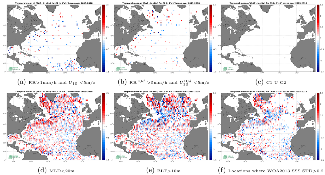
Figure 12: Temporal mean gridded over spatial boxes of size 1^\circ \times 1^\circ of \Delta\text{SSS} (SMAP-L2-RSS-V3-70KM - Argo) for 6 different subdatasets corresponding to: RR > 1\text{mm/h} and U_{10} < 5\text{m/s} (a), RR^{10d} > 5\text{mm/h} and U_{10}^{10d} < 5\text{m/s} (b), C1 U C2 (c), MLD < 20\text{m} (d), BLT > 10\text{m} (e), Locations where WOA2013 SSS STD > 0.2 (f).
