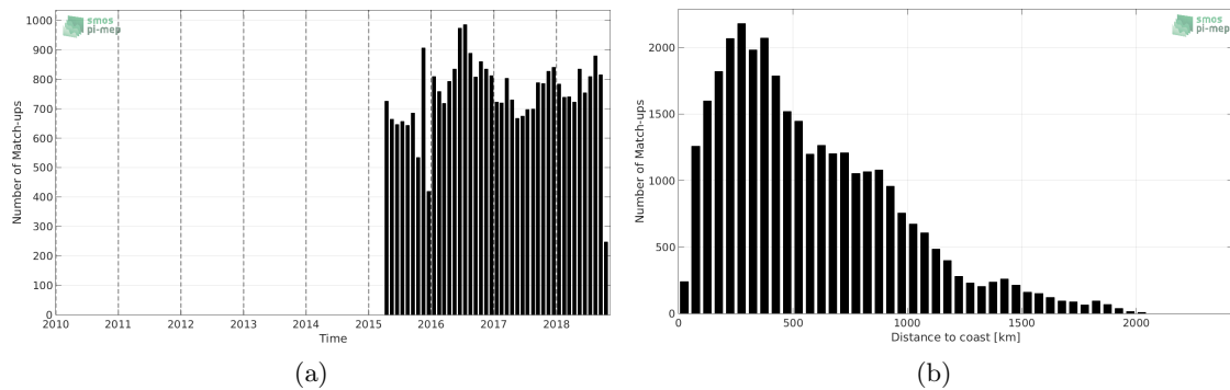
Figure 1: Number of match-ups between Argo and SMAP-L2-RSS-V3-70KM SSS as a function of time (a) and as function of the distance to coast (b) over the North Atlantic Ocean Pi-MEP region and for the full satellite product period.
