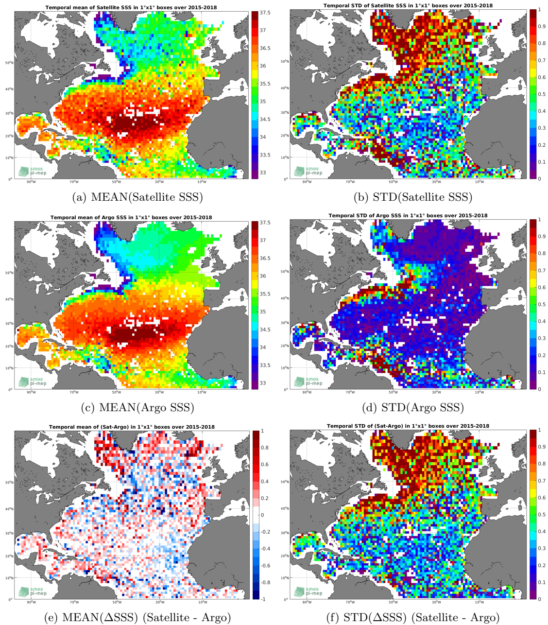
Figure 6: Temporal mean (left) and STD (right) of SSS from SMAP-L2-RSS-V3-70KM (top), Argo (middle), and of \Delta SSS (Satellite - Argo). Only match-up pairs are used to generate these maps.
