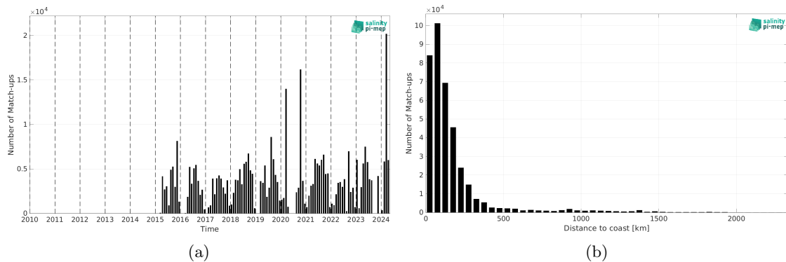
Figure 2: Number of match-ups between TSG (SAMOS) and SMAP SSS L2 v5.0 (JPL) SSS as a function of time (a) and as function of the distance to coast (b) over the North Atlantic Ocean Pi-MEP region and for the full satellite product period.
