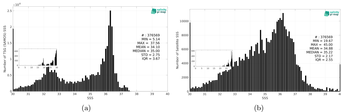
Figure 3: Histograms of SSS from TSG (SAMOS) (a) and SMAP SSS L2 v5.0 (JPL) (b) considering all match-up pairs per bins of 0.1 over the North Atlantic Ocean Pi-MEP region and for the full satellite product period.
