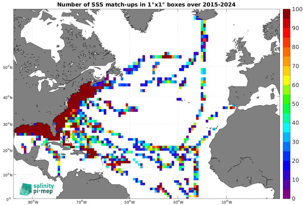
Figure 5: Number of SSS match-ups between TSG (SAMOS) SSS and the SMAP SSS L2 v5.0 (JPL) SSS product for the North Atlantic Ocean Pi-MEP region over 1^\circ \times 1^\circ boxes and for the full satellite product period.
