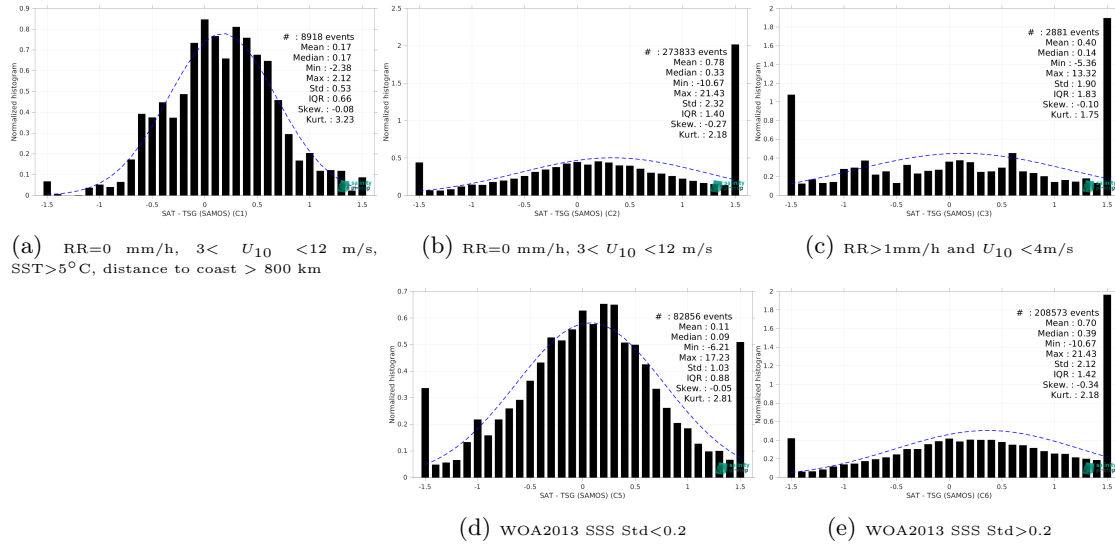
Figure 15: Normalized histogram of \Delta\text{SSS} (SMAP SSS L2 v5.0 (JPL) - TSG (SAMOS)) for 5 different subdatasets corresponding to: RR=0 mm/h, 3 < U_{10} < 12 m/s, SST>5°C, distance to coast > 800 km (a), RR=0 mm/h, 3 < U_{10} < 12 m/s (b), RR>1mm/h and U_{10} < 4 m/s (c), WOA2013 SSS Std<0.2 (d), WOA2013 SSS Std>0.2 (e).
