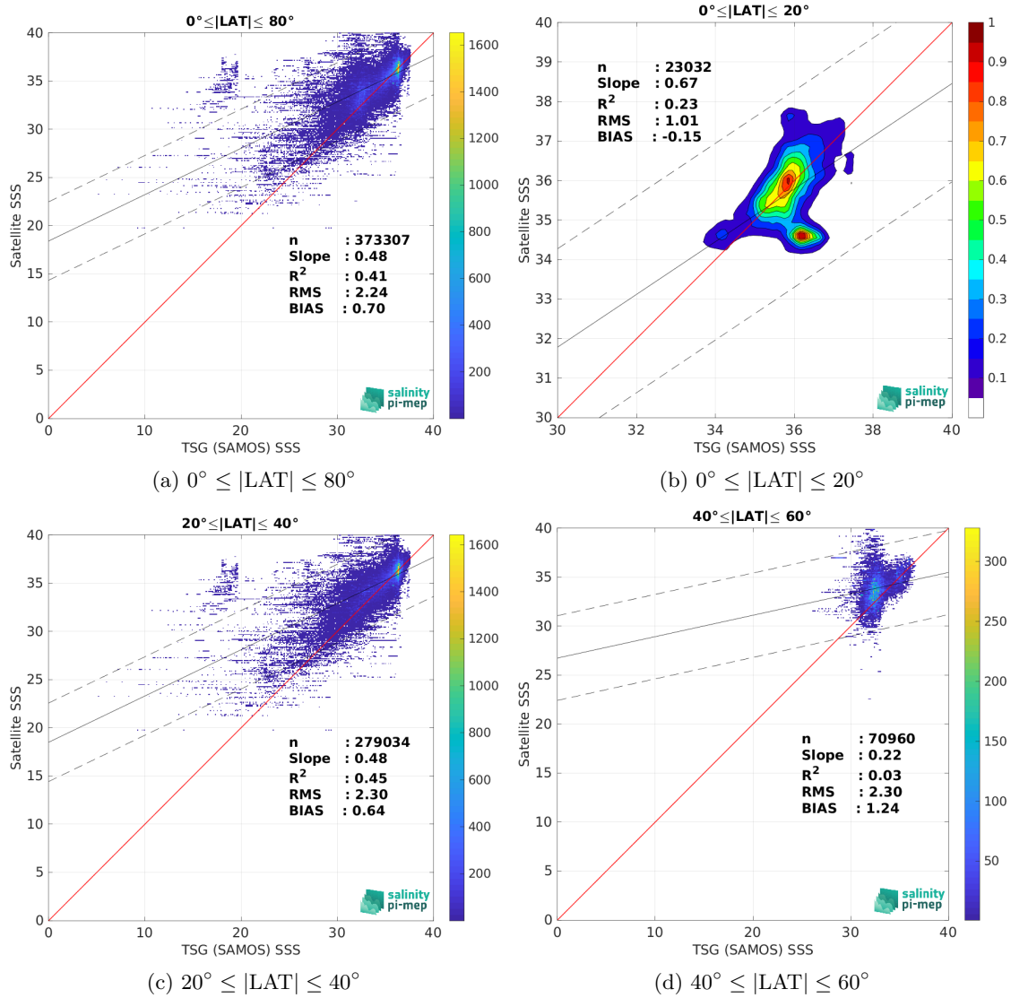
Figure 10: Contour maps of the concentration of SMAP SSS L2 v5.0 (JPL) SSS (y-axis) versus TSG (SAMOS) SSS (x-axis) at match-up pairs for different latitude bands. For each plot, the red line shows x=y . The black thin and dashed lines indicate a linear fit through the data cloud and the \pm 95\% confidence levels, respectively. The number match-up pairs n , the slope and R^2 coefficient of the linear fit, the root mean square (RMS) and the mean bias between satellite and in situ data are indicated for each latitude band in each plots.
