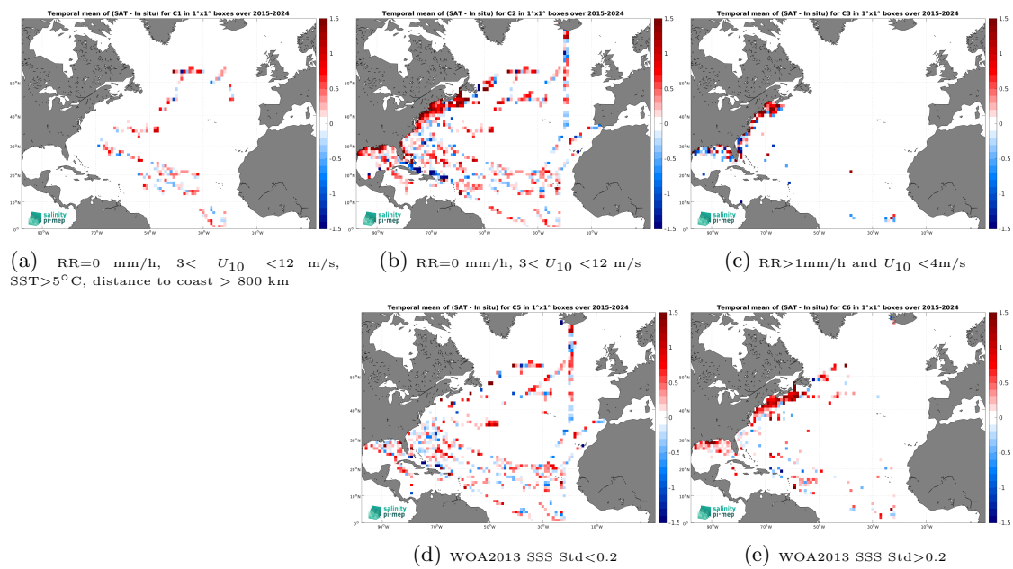
Figure 14: Temporal mean gridded over spatial boxes of size 1^\circ \times 1^\circ of \Delta\text{SSS} (SMAP SSS L2 v5.0 (JPL) - TSG (SAMOS)) for 5 different subdatasets corresponding to:RR=0 mm/h, 3 < U_{10} < 12 m/s, SST>5°C, distance to coast > 800 km (a), RR=0 mm/h, 3 < U_{10} < 12 m/s (b), RR>1mm/h and U_{10} < 4 m/s (c), WOA2013 SSS Std<0.2 (d), WOA2013 SSS Std>0.2 (e).
