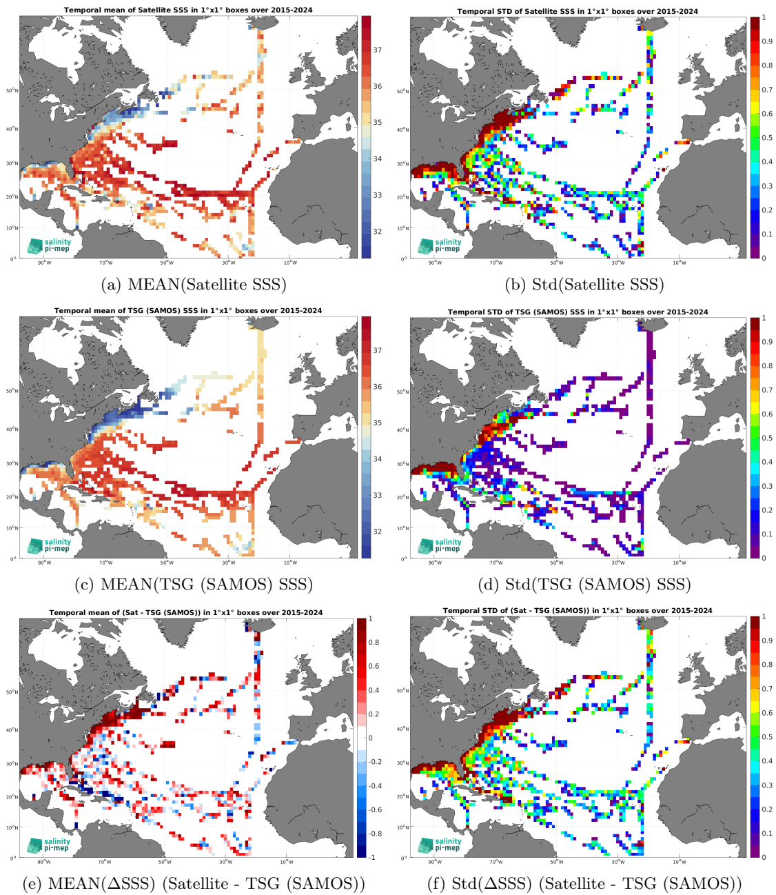
Figure 7: Temporal mean (left) and Std (right) of SSS from SMAP SSS L2 v5.0 (JPL) (top), TSG (SAMOS) (middle), and of \Delta SSS (Satellite - TSG (SAMOS)). Only match-up pairs are used to generate these maps.
