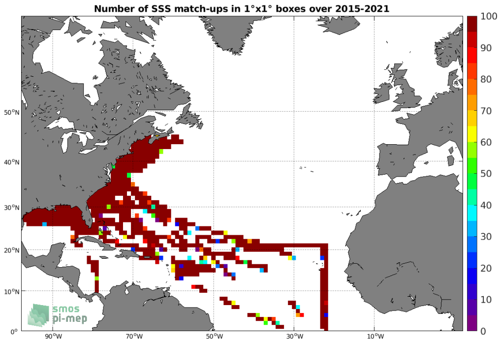
Figure 4: Number of SSS match-ups between TSG (SAMOS) SSS and the SMAP SSS L2 v5.0 (JPL) SSS product for the North Atlantic Ocean Pi-MEP region over 1°x1° boxes and for the full satellite product period.
