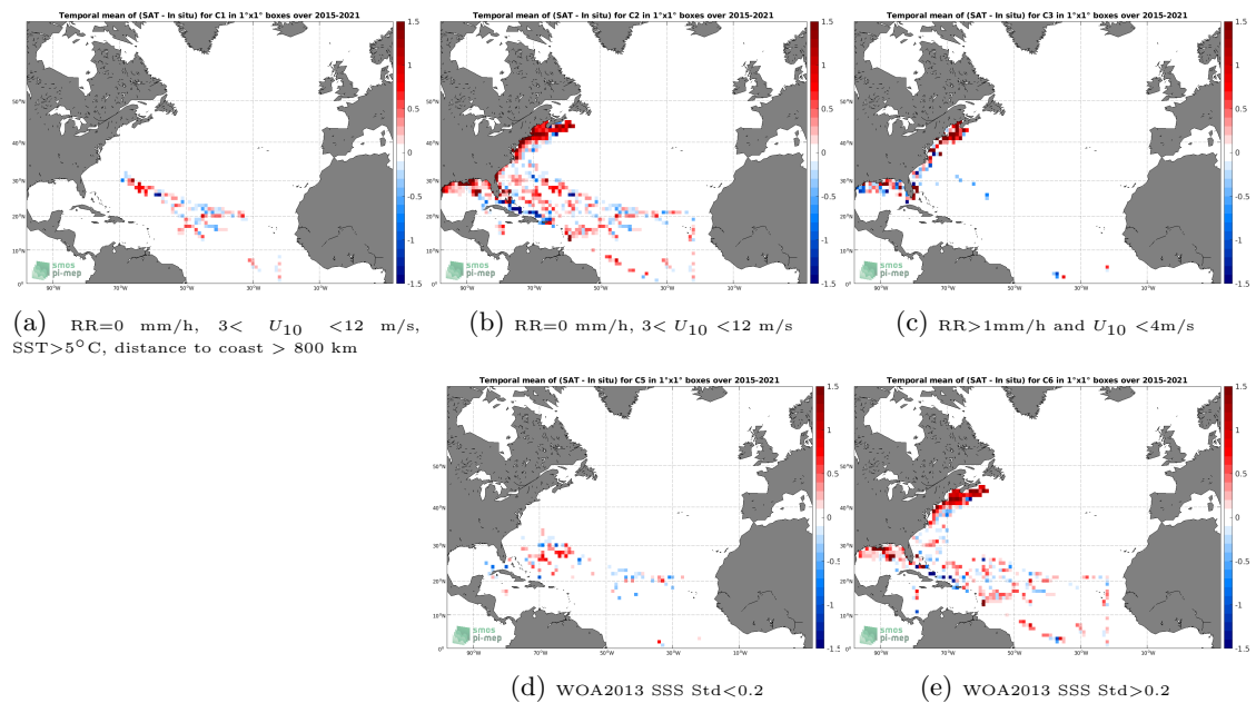
Figure 12: Temporal mean gridded over spatial boxes of size 1°x1° of \Delta SSS (SMAP SSS L2 v5.0 (JPL) - TSG (SAMOS)) for 5 different subdatasets corresponding to:RR=0 mm/h, 3 < U_{10} < 12 m/s, SST>5°C, distance to coast > 800 km (a), RR=0 mm/h, 3 < U_{10} < 12 m/s (b), RR>1mm/h and U_{10} < 4 m/s (c), WOA2013 SSS Std<0.2 (d), WOA2013 SSS Std>0.2 (e).
