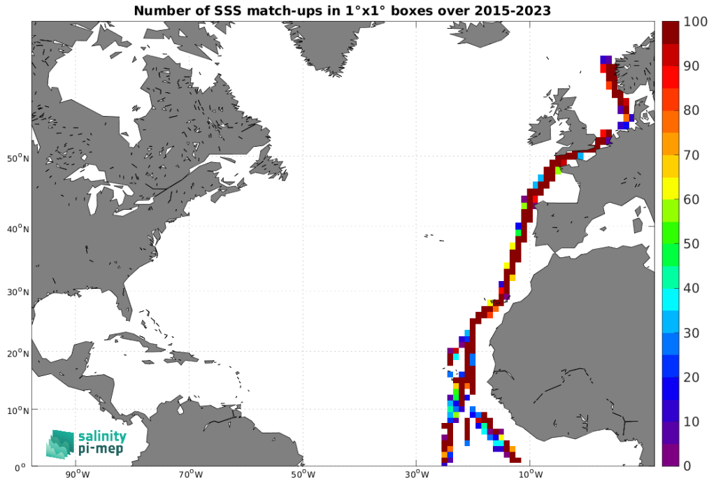
Figure 5: Number of SSS match-ups between TSG (Polarstern) SSS and the SMAP SSS L2 v5.0 (JPL) SSS product for the North Atlantic Ocean Pi-MEP region over 1^\circ \times 1^\circ boxes and for the full satellite product period.
