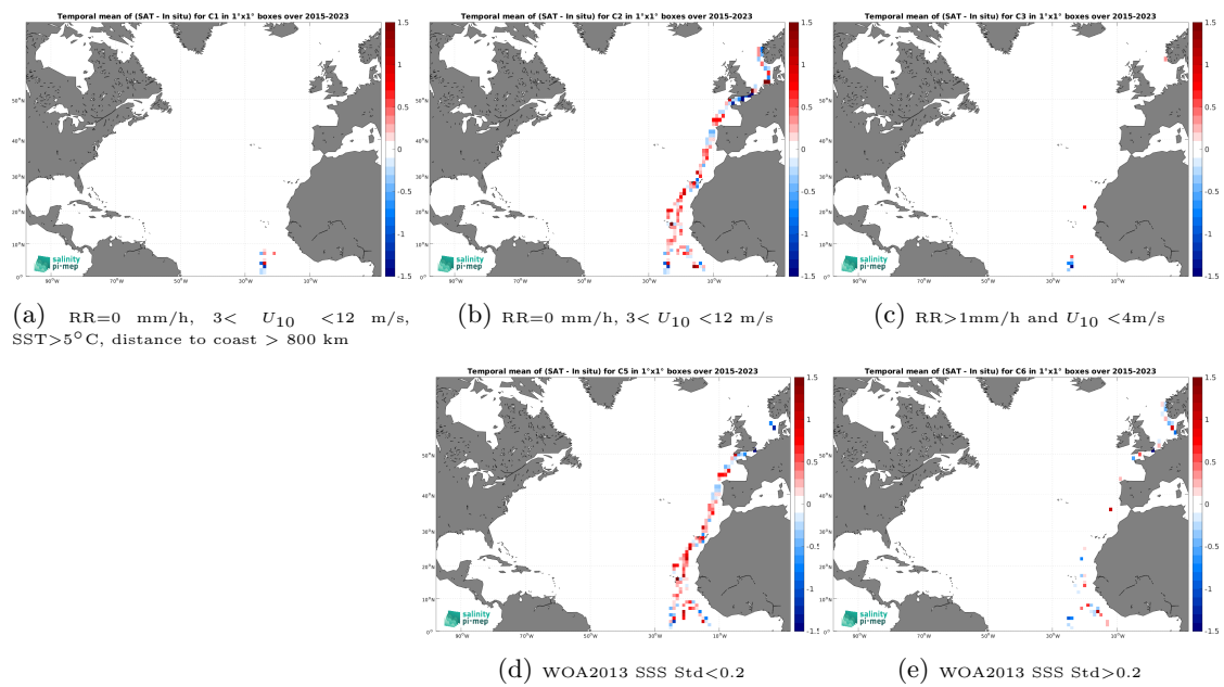
Figure 14: Temporal mean gridded over spatial boxes of size 1^\circ \times 1^\circ of \Delta\text{SSS} (SMAP SSS L2 v5.0 (JPL) - TSG (Polarstern)) for 5 different subdatasets corresponding to:RR=0 mm/h, 3 < U_{10} < 12 m/s, SST >5^\circ\text{C} , distance to coast > 800 km (a), RR=0 mm/h, 3 < U_{10} < 12 m/s (b), RR >1 mm/h and U_{10} < 4 m/s (c), WOA2013 SSS Std <0.2 (d), WOA2013 SSS Std >0.2 (e).
