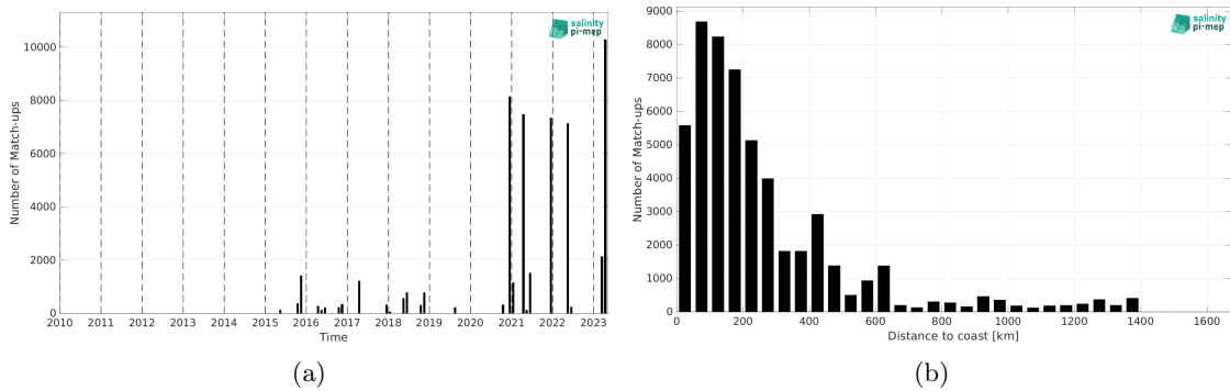
Figure 2: Number of match-ups between TSG (Polarstern) and SMAP SSS L2 v5.0 (JPL) SSS as a function of time (a) and as function of the distance to coast (b) over the North Atlantic Ocean Pi-MEP region and for the full satellite product period.
