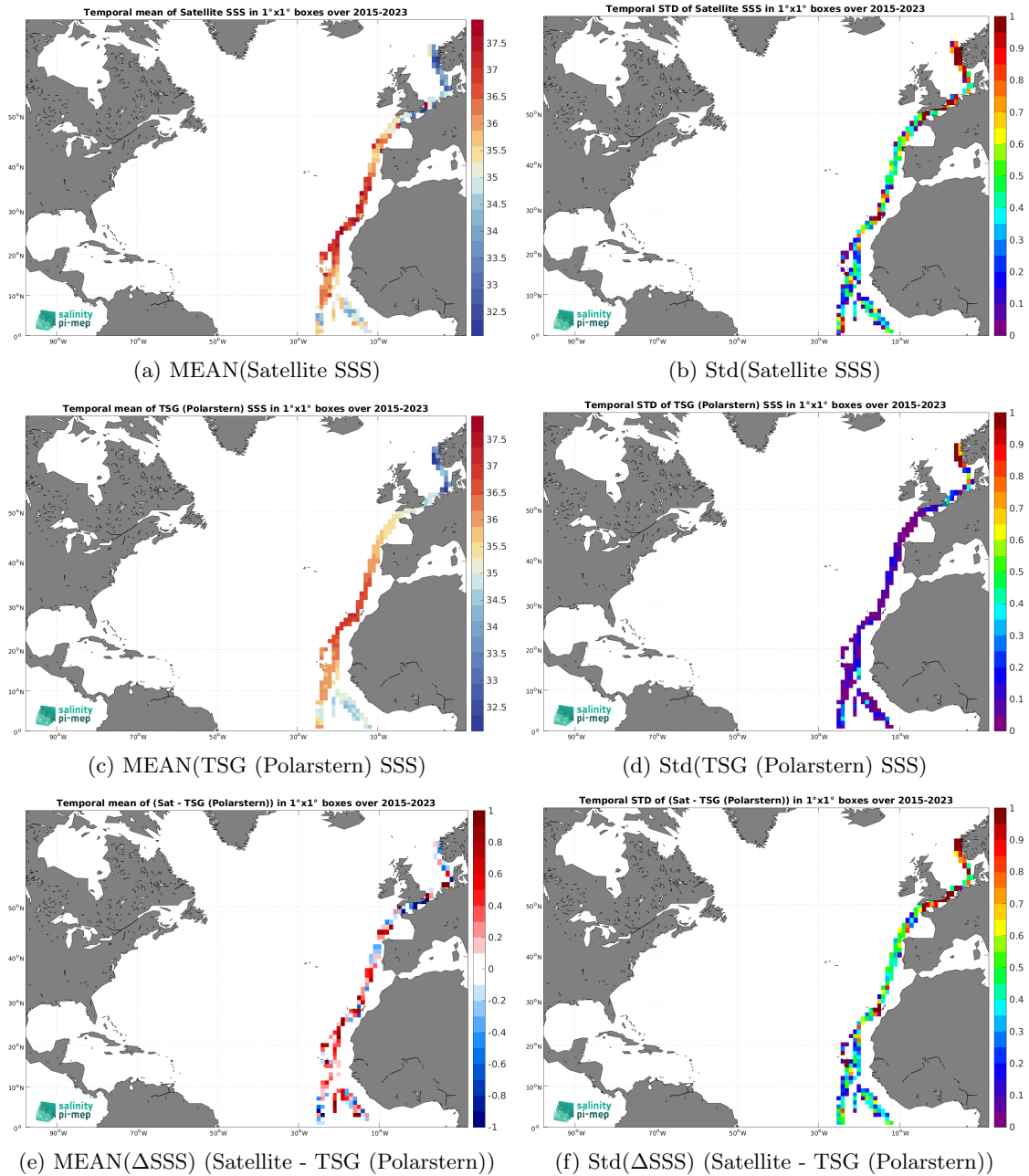
Figure 7: Temporal mean (left) and Std (right) of SSS from SMAP SSS L2 v5.0 (JPL) (top), TSG (Polarstern) (middle), and of \Delta SSS (Satellite - TSG (Polarstern)). Only match-up pairs are used to generate these maps.
