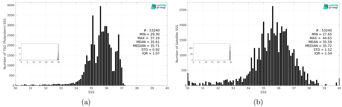
Figure 3: Histograms of SSS from TSG (Polarstern) (a) and SMAP SSS L2 v5.0 (JPL) (b) considering all match-up pairs per bins of 0.1 over the North Atlantic Ocean Pi-MEP region and for the full satellite product period.
