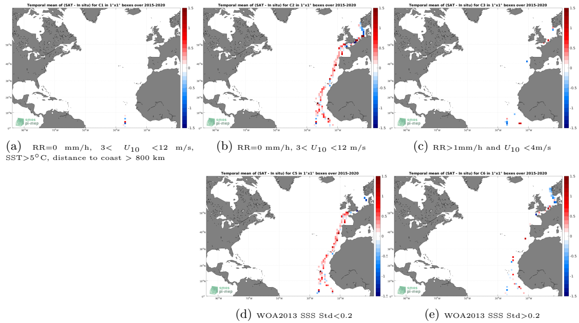
Figure 12: Temporal mean gridded over spatial boxes of size 1^\circ \times 1^\circ of \Delta\text{SSS} (SMAP SSS L2 v5.0 (JPL) - TSG (Polarstern)) for 5 different subdatasets corresponding to:RR=0 mm/h, 3 < U_{10} < 12 m/s, SST >5^\circ\text{C} , distance to coast > 800 km (a), RR=0 mm/h, 3 < U_{10} < 12 m/s (b), RR >1 mm/h and U_{10} < 4 m/s (c), WOA2013 SSS Std <0.2 (d), WOA2013 SSS Std >0.2 (e).
