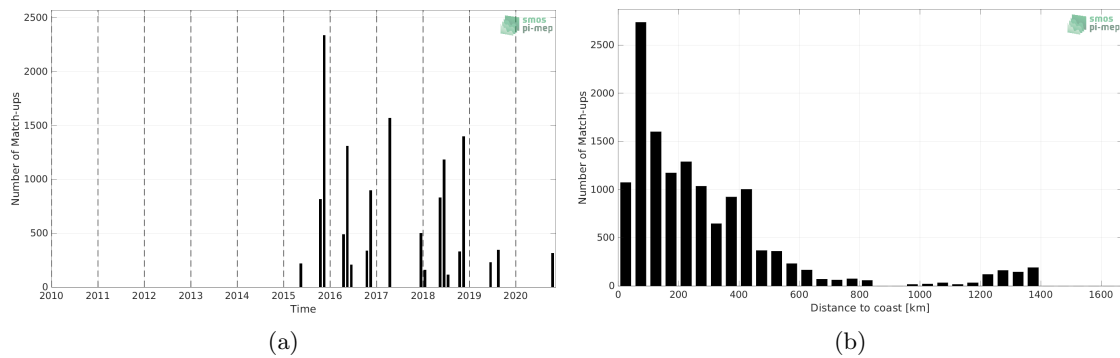
Figure 1: Number of match-ups between TSG (Polarstern) and SMAP SSS L2 v5.0 (JPL) SSS as a function of time (a) and as function of the distance to coast (b) over the North Atlantic Ocean Pi-MEP region and for the full satellite product period.
