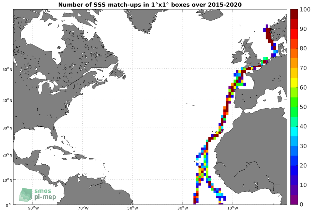
Figure 4: Number of SSS match-ups between TSG (Polarstern) SSS and the SMAP SSS L2 v5.0 (JPL) SSS product for the North Atlantic Ocean Pi-MEP region over 1^\circ \times 1^\circ boxes and for the full satellite product period.
