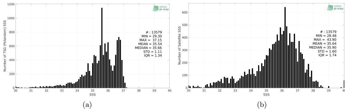
Figure 2: Histograms of SSS from TSG (Polarstern) (a) and SMAP SSS L2 v5.0 (JPL) (b) considering all match-up pairs per bins of 0.1 over the North Atlantic Ocean Pi-MEP region and for the full satellite product period.
