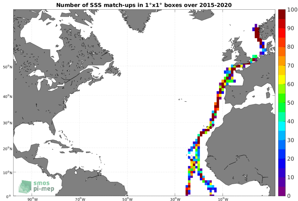
Figure 4: Number of SSS match-ups between TSG (Polarstern) SSS and the SMAP SSS L2 v5.0 (JPL) SSS product for the North Atlantic Ocean Pi-MEP region over 1°x1° boxes and for the full satellite product period.
