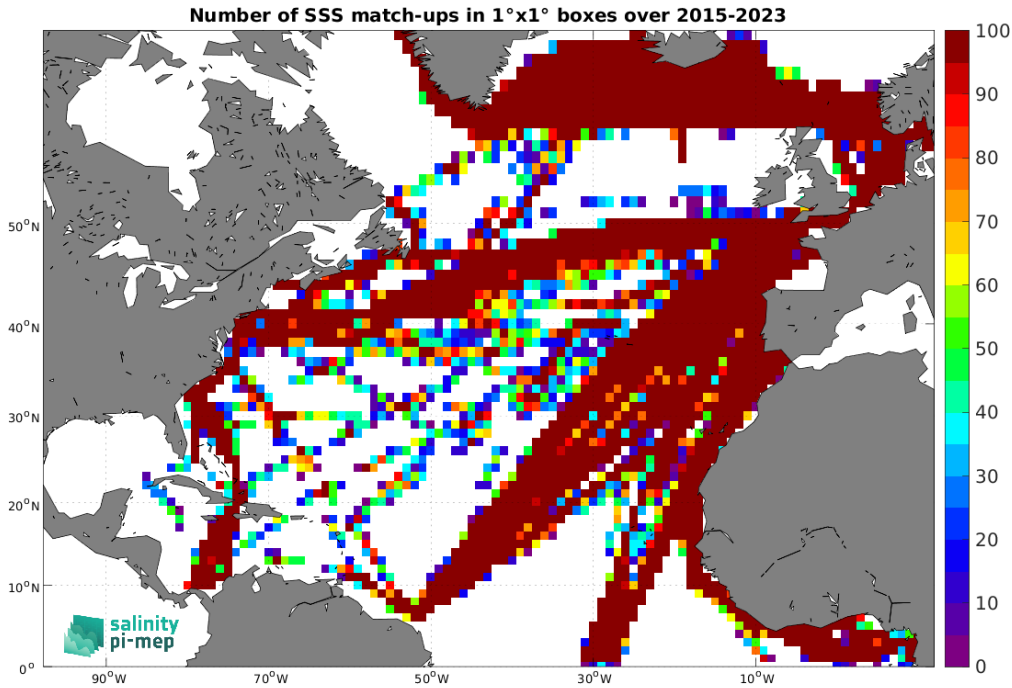
Figure 5: Number of SSS match-ups between TSG (LEGOS-DM) SSS and the SMAP SSS L2 v5.0 (JPL) SSS product for the North Atlantic Ocean Pi-MEP region over 1^\circ \times 1^\circ boxes and for the full satellite product period.
