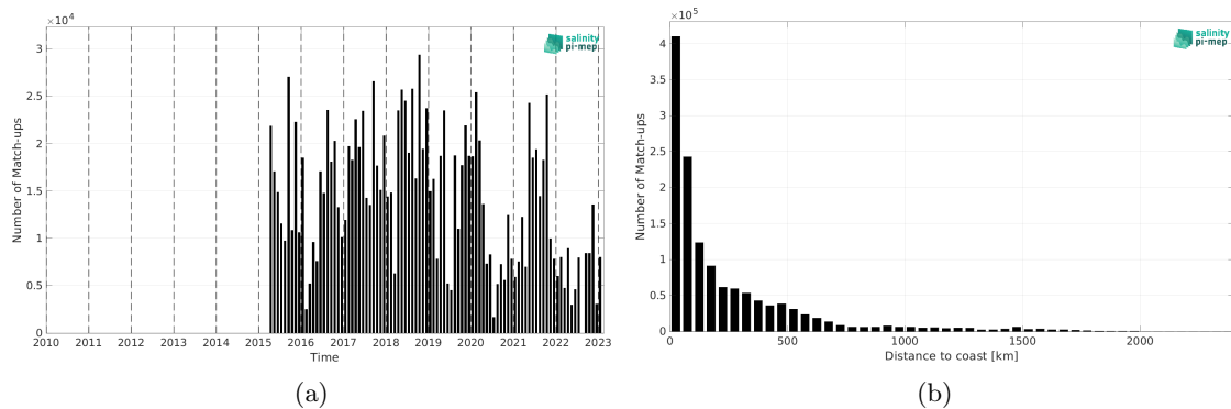
Figure 2: Number of match-ups between TSG (LEGOS-DM) and SMAP SSS L2 v5.0 (JPL) SSS as a function of time (a) and as function of the distance to coast (b) over the North Atlantic Ocean Pi-MEP region and for the full satellite product period.
