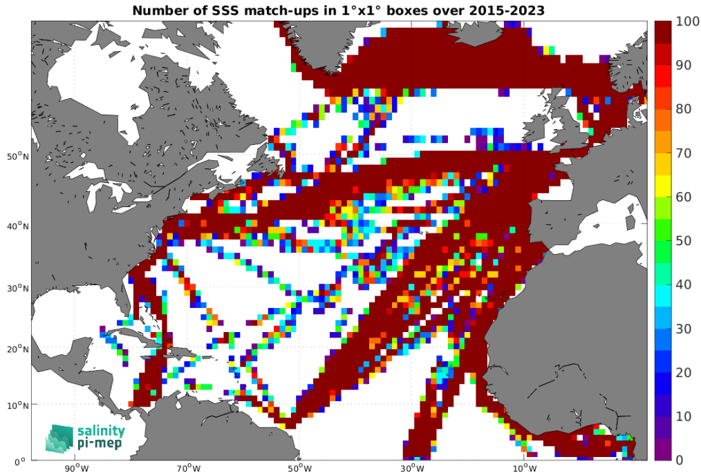
Figure 4: Number of SSS match-ups between TSG (LEGOS-DM) SSS and the SMAP SSS L2 v5.0 (JPL) SSS product for the North Atlantic Ocean Pi-MEP region over 1^\circ \times 1^\circ boxes and for the full satellite product period.
