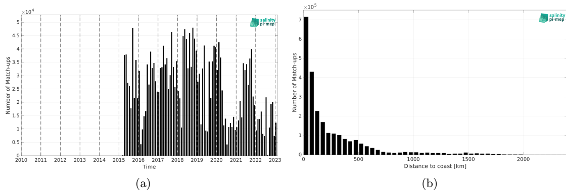
Figure 1: Number of match-ups between TSG (LEGOS-DM) and SMAP SSS L2 v5.0 (JPL) SSS as a function of time (a) and as function of the distance to coast (b) over the North Atlantic Ocean Pi-MEP region and for the full satellite product period.
