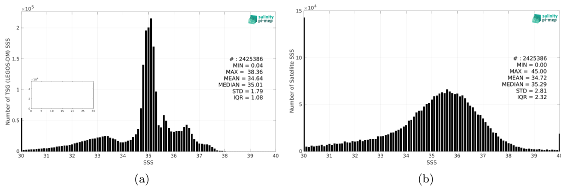
Figure 2: Histograms of SSS from TSG (LEGOS-DM) (a) and SMAP SSS L2 v5.0 (JPL) (b) considering all match-up pairs per bins of 0.1 over the North Atlantic Ocean Pi-MEP region and for the full satellite product period.
