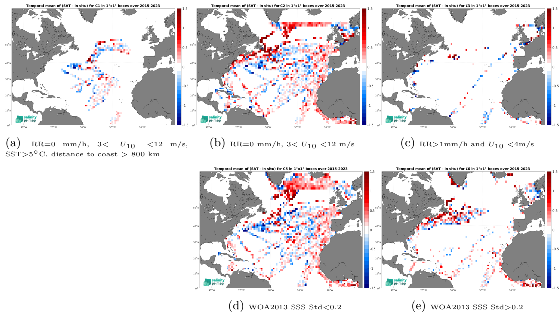
Figure 12: Temporal mean gridded over spatial boxes of size 1^\circ \times 1^\circ of \Delta SSS (SMAP SSS L2 v5.0 (JPL) - TSG (LEGOS-DM)) for 5 different subdatasets corresponding to:RR=0 mm/h, 3 < U_{10} < 12 m/s, SST >5^\circ\text{C} , distance to coast > 800 km (a), RR=0 mm/h, 3 < U_{10} < 12 m/s (b), RR >1 mm/h and U_{10} < 4 m/s (c), WOA2013 SSS Std <0.2 (d), WOA2013 SSS Std >0.2 (e).
