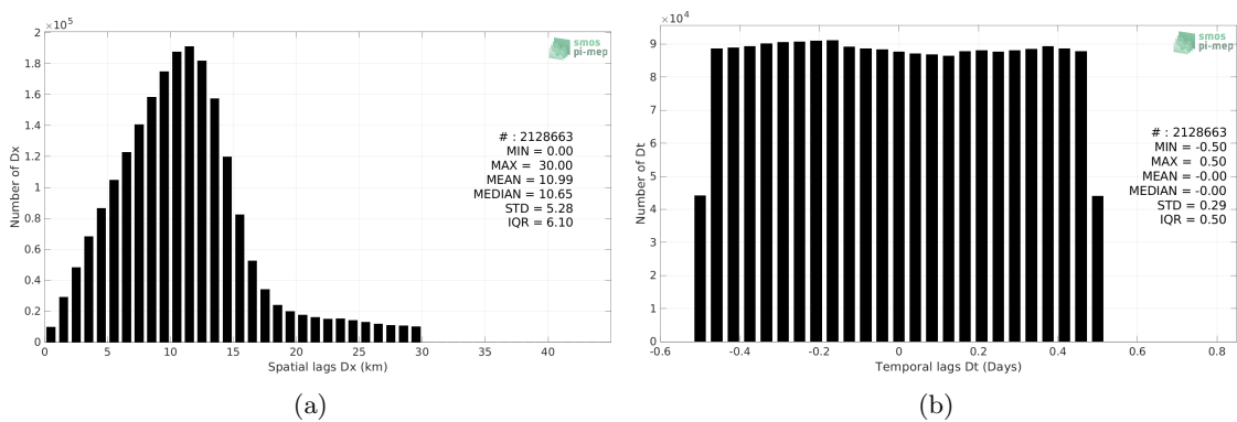
Figure 5: Histograms of the spatial (a) and temporal (b) lags between the location/time of the TSG (LEGOS-DM) measurement and the date of the corresponding SMAP SSS L2 v5.0 (JPL) SSS pixel.
