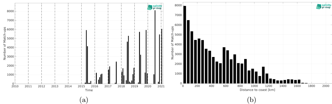
Figure 2: Number of match-ups between TSG (GOSUD-Sailing-ship) and SMAP SSS L2 v5.0 (JPL) SSS as a function of time (a) and as function of the distance to coast (b) over the North Atlantic Ocean Pi-MEP region and for the full satellite product period.
