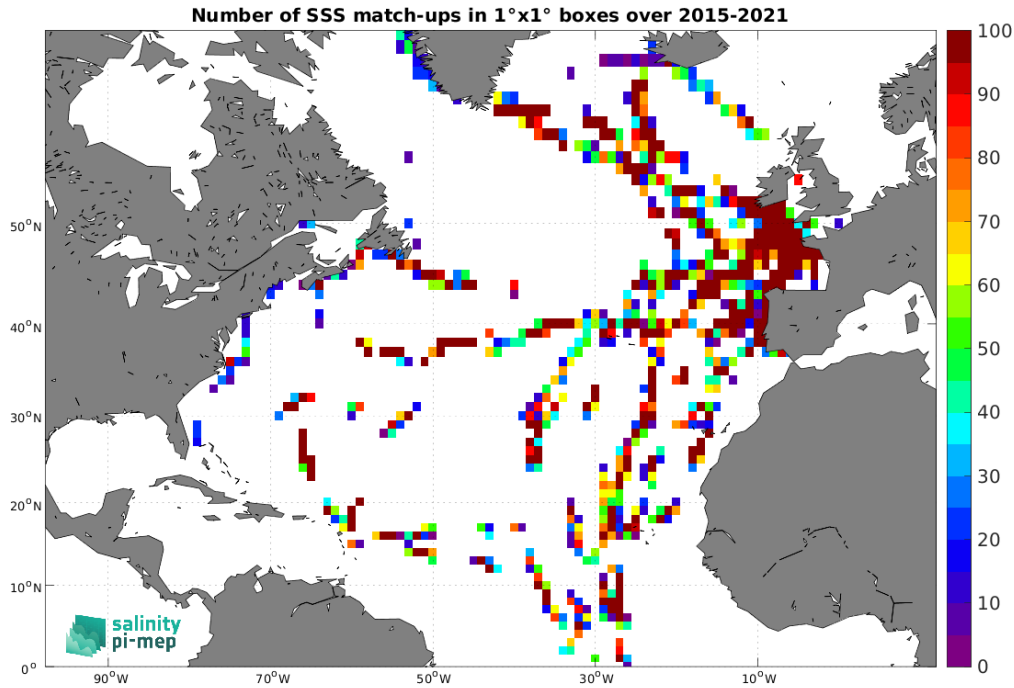
Figure 5: Number of SSS match-ups between TSG (GOSUD-Sailing-ship) SSS and the SMAP SSS L2 v5.0 (JPL) SSS product for the North Atlantic Ocean Pi-MEP region over 1^\circ \times 1^\circ boxes and for the full satellite product period.
