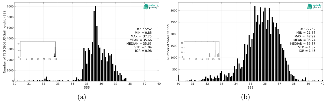
Figure 3: Histograms of SSS from TSG (GOSUD-Sailing-ship) (a) and SMAP SSS L2 v5.0 (JPL) (b) considering all match-up pairs per bins of 0.1 over the North Atlantic Ocean Pi-MEP region and for the full satellite product period.
