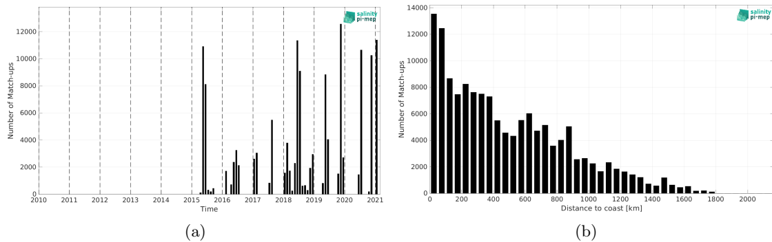
Figure 1: Number of match-ups between TSG (GOSUD-Sailing-ship) and SMAP SSS L2 v5.0 (JPL) SSS as a function of time (a) and as function of the distance to coast (b) over the North Atlantic Ocean Pi-MEP region and for the full satellite product period.
