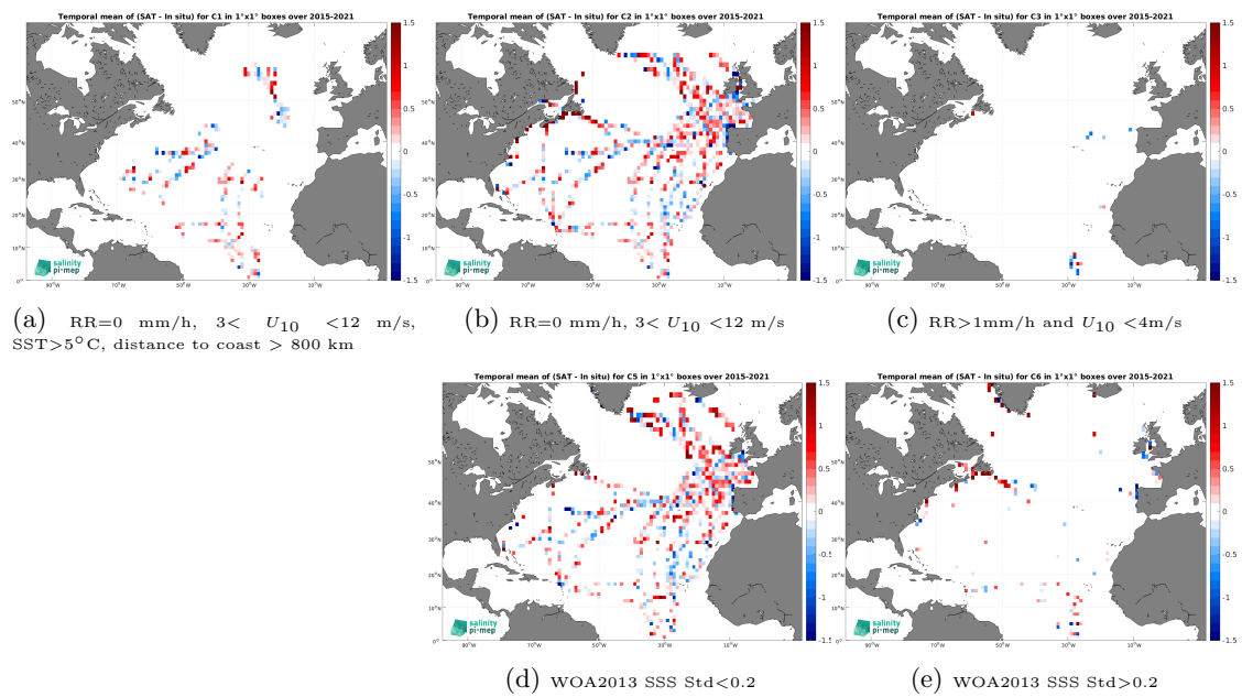
Figure 12: Temporal mean gridded over spatial boxes of size 1^\circ \times 1^\circ of \Delta\text{SSS} (SMAP SSS L2 v5.0 (JPL) - TSG (GOSUD-Sailing-ship)) for 5 different subdatasets corresponding to:RR=0 mm/h, 3 < U_{10} < 12 m/s, SST >5^\circ\text{C} , distance to coast > 800 km (a), RR=0 mm/h, 3 < U_{10} < 12 m/s (b), RR >1 mm/h and U_{10} < 4 m/s (c), WOA2013 SSS Std <0.2 (d), WOA2013 SSS Std >0.2 (e).
