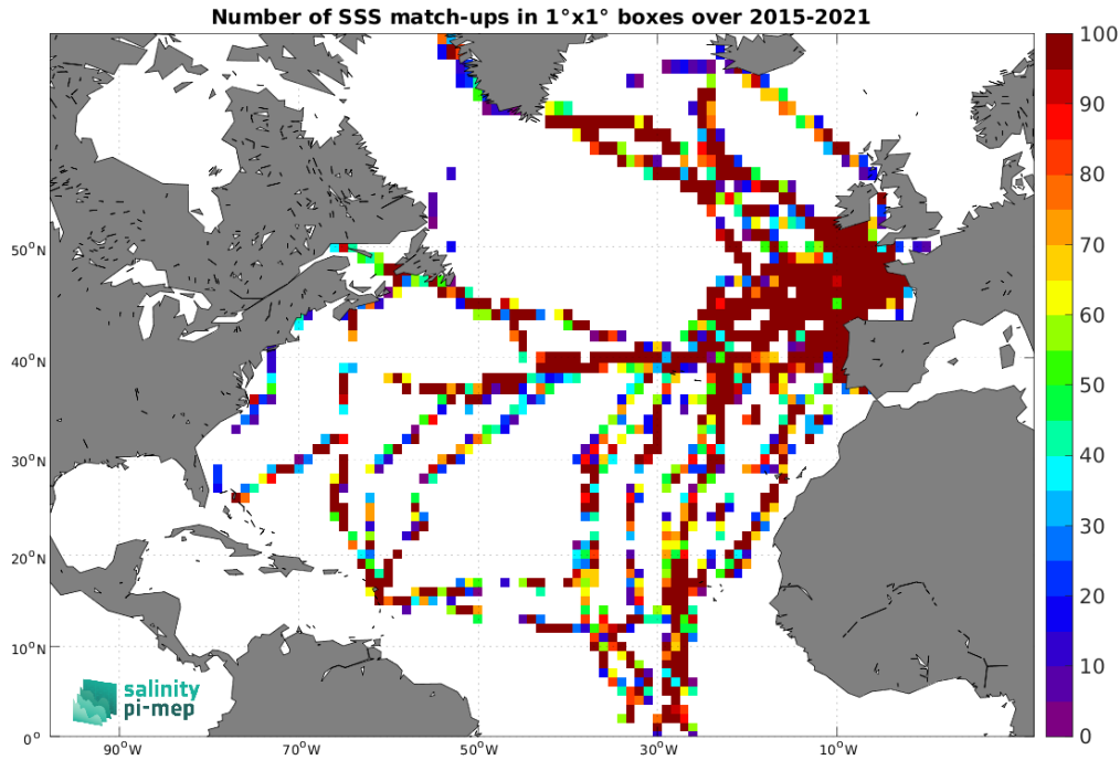
Figure 4: Number of SSS match-ups between TSG (GOSUD-Sailing-ship) SSS and the SMAP SSS L2 v5.0 (JPL) SSS product for the North Atlantic Ocean Pi-MEP region over 1^\circ \times 1^\circ boxes and for the full satellite product period.
