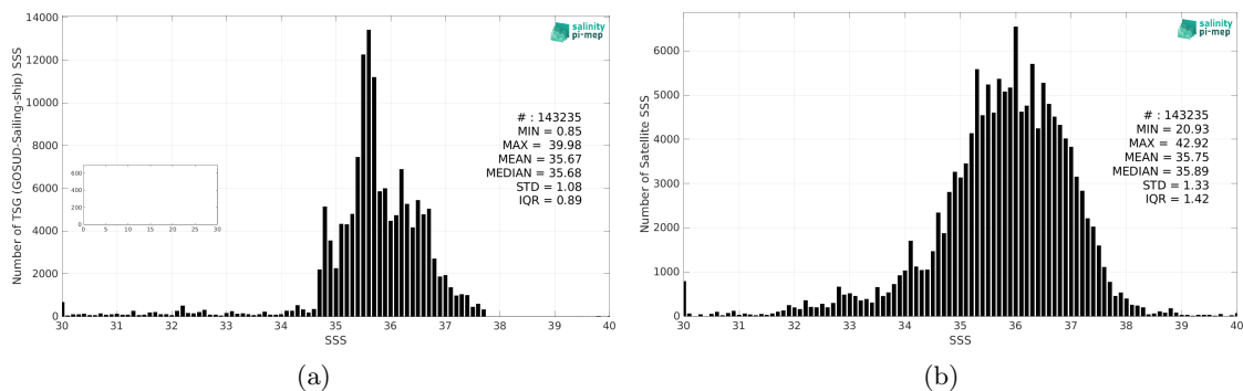
Figure 2: Histograms of SSS from TSG (GOSUD-Sailing-ship) (a) and SMAP SSS L2 v5.0 (JPL) (b) considering all match-up pairs per bins of 0.1 over the North Atlantic Ocean Pi-MEP region and for the full satellite product period.
