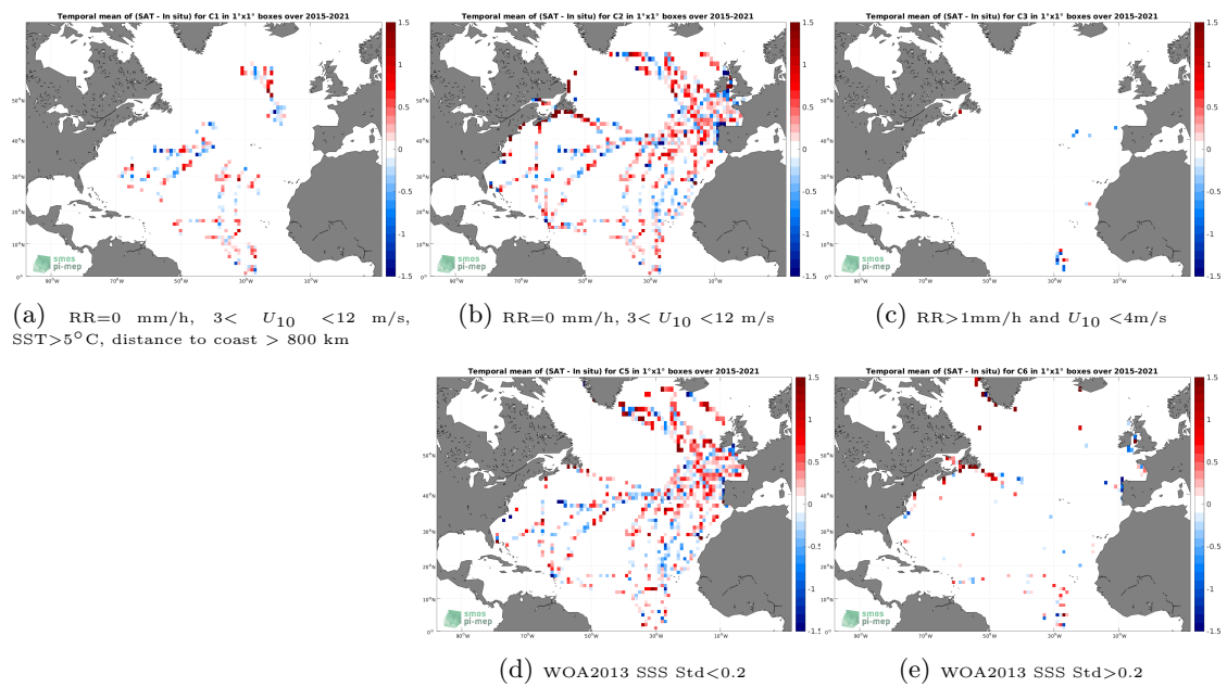
Figure 12: Temporal mean gridded over spatial boxes of size 1^\circ \times 1^\circ of \Delta SSS (SMAP SSS L2 v5.0 (JPL) - TSG (GOSUD-Sailing-ship)) for 5 different subdatasets corresponding to:RR=0 mm/h, 3 < U_{10} < 12 m/s, SST > 5°C, distance to coast > 800 km (a), RR=0 mm/h, 3 < U_{10} < 12 m/s (b), RR > 1mm/h and U_{10} < 4 m/s (c), WOA2013 SSS Std < 0.2 (d), WOA2013 SSS Std > 0.2 (e).
