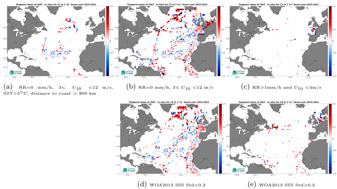
Figure 14: Temporal mean gridded over spatial boxes of size 1^\circ \times 1^\circ of \Delta\text{SSS} (SMAP SSS L2 v5.0 (JPL) - TSG (GOSUD-Research-vessel)) for 5 different subdatasets corresponding to:RR=0 mm/h, 3 < U_{10} < 12 m/s, SST >5^\circ\text{C} , distance to coast > 800 km (a), RR=0 mm/h, 3 < U_{10} < 12 m/s (b), RR >1 mm/h and U_{10} < 4 m/s (c), WOA2013 SSS Std <0.2 (d), WOA2013 SSS Std >0.2 (e).
