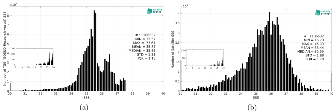
Figure 3: Histograms of SSS from TSG (GOSUD-Research-vessel) (a) and SMAP SSS L2 v5.0 (JPL) (b) considering all match-up pairs per bins of 0.1 over the North Atlantic Ocean Pi-MEP region and for the full satellite product period.
