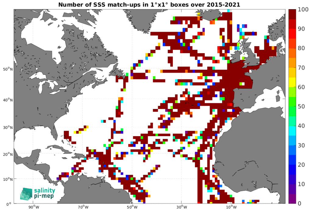
Figure 5: Number of SSS match-ups between TSG (GOSUD-Research-vessel) SSS and the SMAP SSS L2 v5.0 (JPL) SSS product for the North Atlantic Ocean Pi-MEP region over 1^\circ \times 1^\circ boxes and for the full satellite product period.
