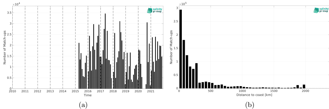
Figure 2: Number of match-ups between TSG (GOSUD-Research-vessel) and SMAP SSS L2 v5.0 (JPL) SSS as a function of time (a) and as function of the distance to coast (b) over the North Atlantic Ocean Pi-MEP region and for the full satellite product period.
