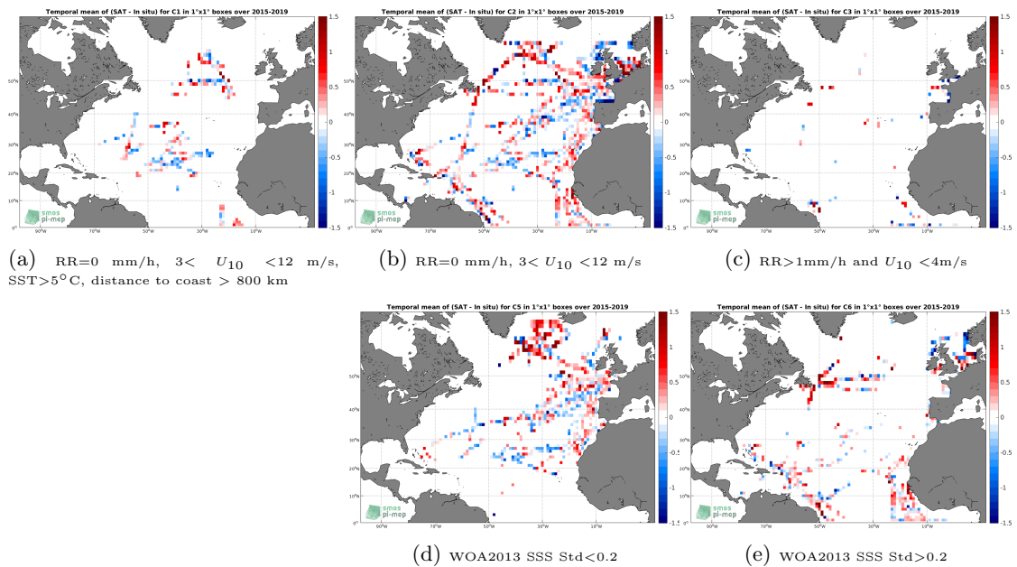
Figure 12: Temporal mean gridded over spatial boxes of size 1^\circ \times 1^\circ of \Delta\text{SSS} (SMAP SSS L2 v5.0 (JPL) - TSG (GOSUD-Research-vessel)) for 5 different subdatasets corresponding to:RR=0 mm/h, 3 < U_{10} < 12 m/s, SST > 5°C, distance to coast > 800 km (a), RR=0 mm/h, 3 < U_{10} < 12 m/s (b), RR > 1mm/h and U_{10} < 4 m/s (c), WOA2013 SSS Std < 0.2 (d), WOA2013 SSS Std > 0.2 (e).
