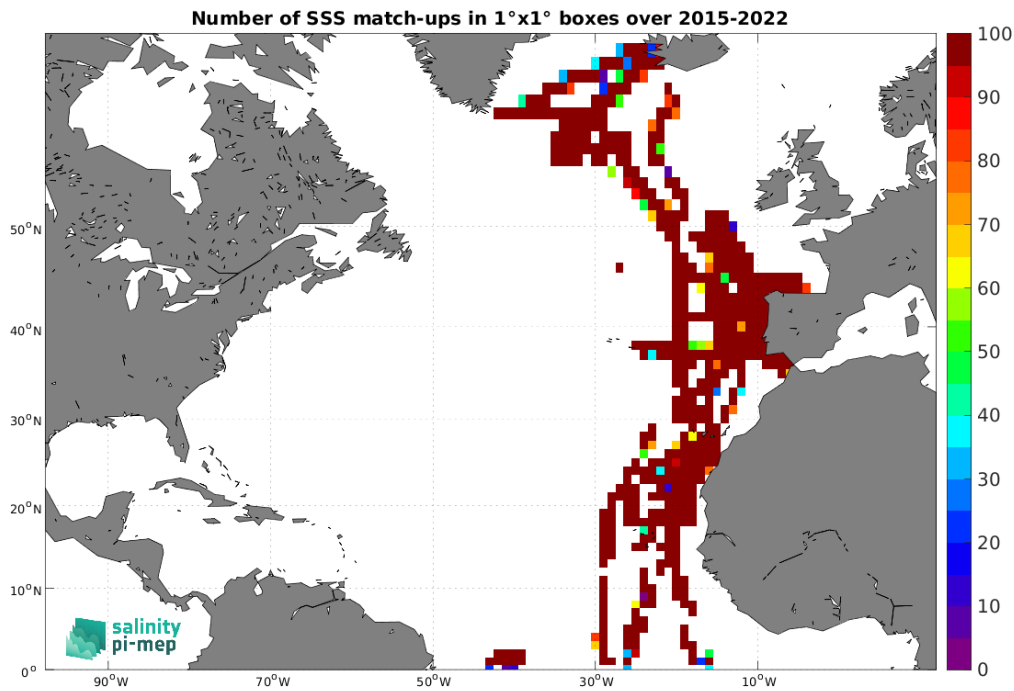
Figure 5: Number of SSS match-ups between TSG (CSIC-UTM) SSS and the SMAP SSS L2 v5.0 (JPL) SSS product for the North Atlantic Ocean Pi-MEP region over 1°x1° boxes and for the full satellite product period.
