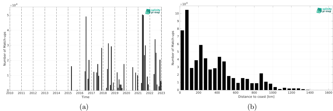
Figure 2: Number of match-ups between TSG (CSIC-UTM) and SMAP SSS L2 v5.0 (JPL) SSS as a function of time (a) and as function of the distance to coast (b) over the North Atlantic Ocean Pi-MEP region and for the full satellite product period.
