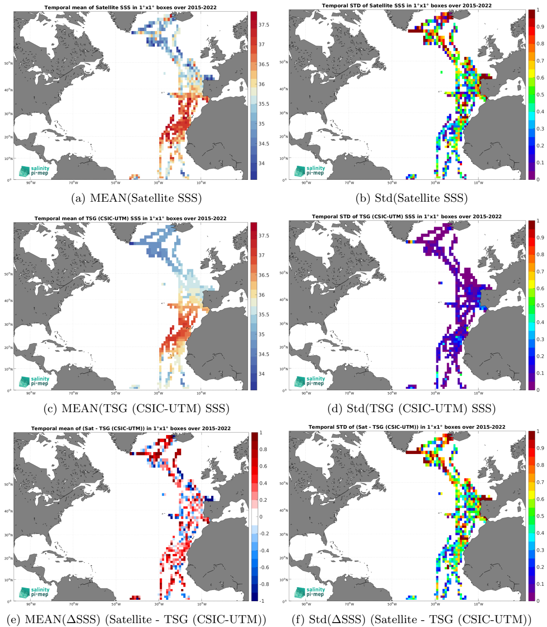
Figure 7: Temporal mean (left) and Std (right) of SSS from SMAP SSS L2 v5.0 (JPL) (top), TSG (CSIC-UTM) (middle), and of \Delta SSS (Satellite - TSG (CSIC-UTM)). Only match-up pairs are used to generate these maps.
