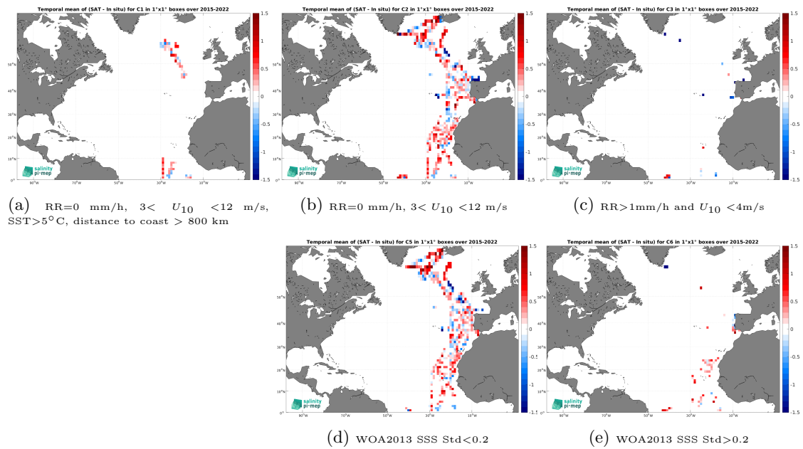
Figure 14: Temporal mean gridded over spatial boxes of size 1^\circ \times 1^\circ of \Delta\text{SSS} (SMAP SSS L2 v5.0 (JPL) - TSG (CSIC-UTM)) for 5 different subdatasets corresponding to:RR=0 mm/h, 3 < U_{10} < 12 m/s, SST > 5°C, distance to coast > 800 km (a), RR=0 mm/h, 3 < U_{10} < 12 m/s (b), RR > 1mm/h and U_{10} < 4 m/s (c), WOA2013 SSS Std < 0.2 (d), WOA2013 SSS Std > 0.2 (e).
