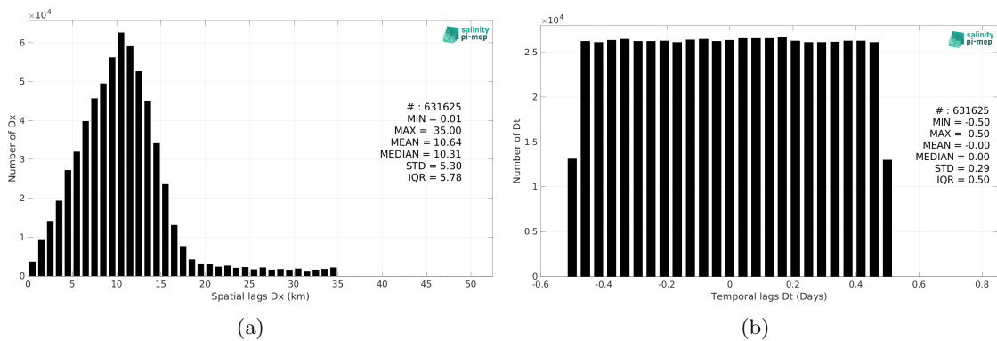
Figure 6: Histograms of the spatial (a) and temporal (b) lags between the location/time of the TSG (CSIC-UTM) measurement and the date of the corresponding SMAP SSS L2 v5.0 (JPL) SSS pixel.
