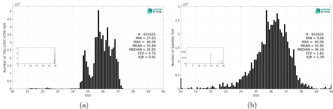
Figure 3: Histograms of SSS from TSG (CSIC-UTM) (a) and SMAP SSS L2 v5.0 (JPL) (b) considering all match-up pairs per bins of 0.1 over the North Atlantic Ocean Pi-MEP region and for the full satellite product period.
