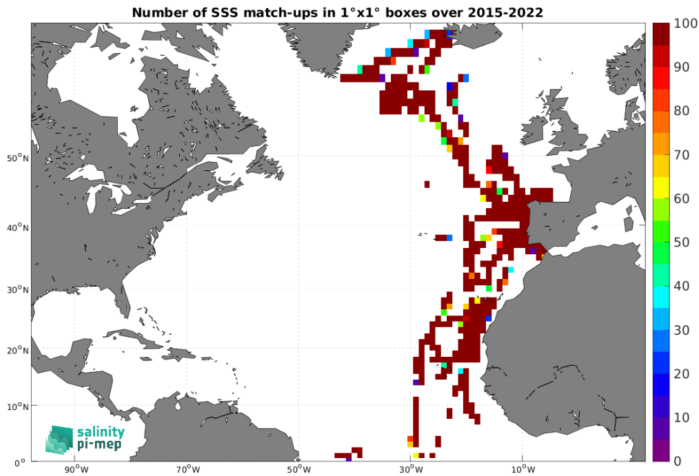
Figure 5: Number of SSS match-ups between TSG (CSIC-UTM) SSS and the SMAP SSS L2 v5.0 (JPL) SSS product for the North Atlantic Ocean Pi-MEP region over 1^\circ \times 1^\circ boxes and for the full satellite product period.
