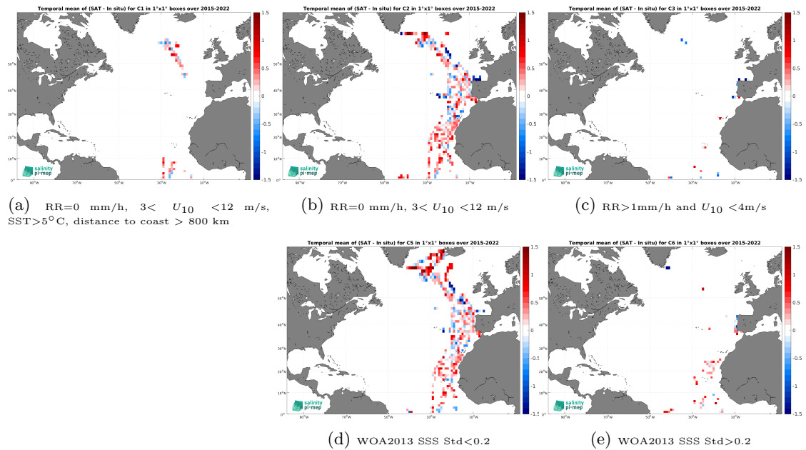
Figure 12: Temporal mean gridded over spatial boxes of size 1^\circ \times 1^\circ of \Delta SSS (SMAP SSS L2 v5.0 (JPL) - TSG (CSIC-UTM)) for 5 different subdatasets corresponding to:RR=0 mm/h, 3 < U_{10} < 12 m/s, SST >5^\circ\text{C} , distance to coast > 800 km (a), RR=0 mm/h, 3 < U_{10} < 12 m/s (b), RR >1 mm/h and U_{10} < 4 m/s (c), WOA2013 SSS Std <0.2 (d), WOA2013 SSS Std >0.2 (e).
