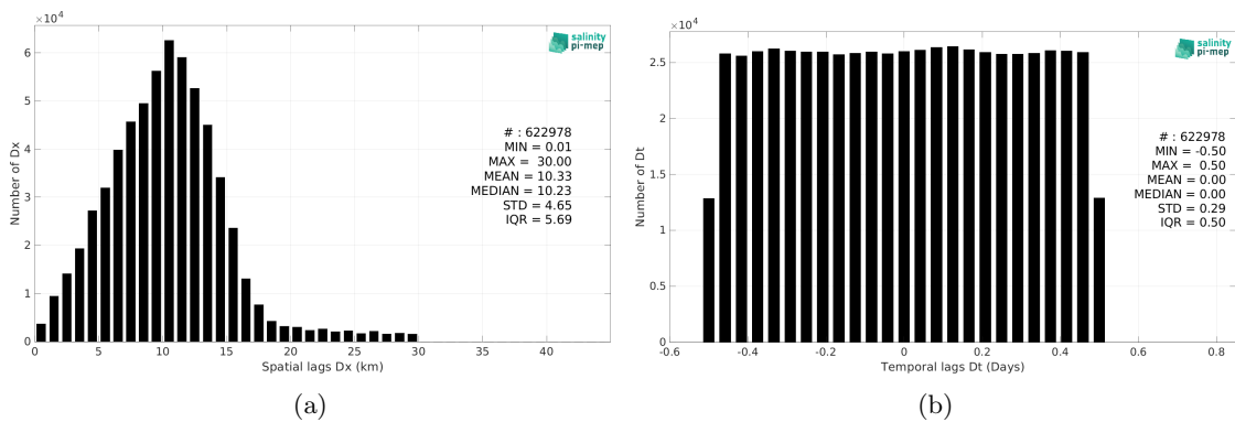
Figure 5: Histograms of the spatial (a) and temporal (b) lags between the location/time of the TSG (CSIC-UTM) measurement and the date of the corresponding SMAP SSS L2 v5.0 (JPL) SSS pixel.
