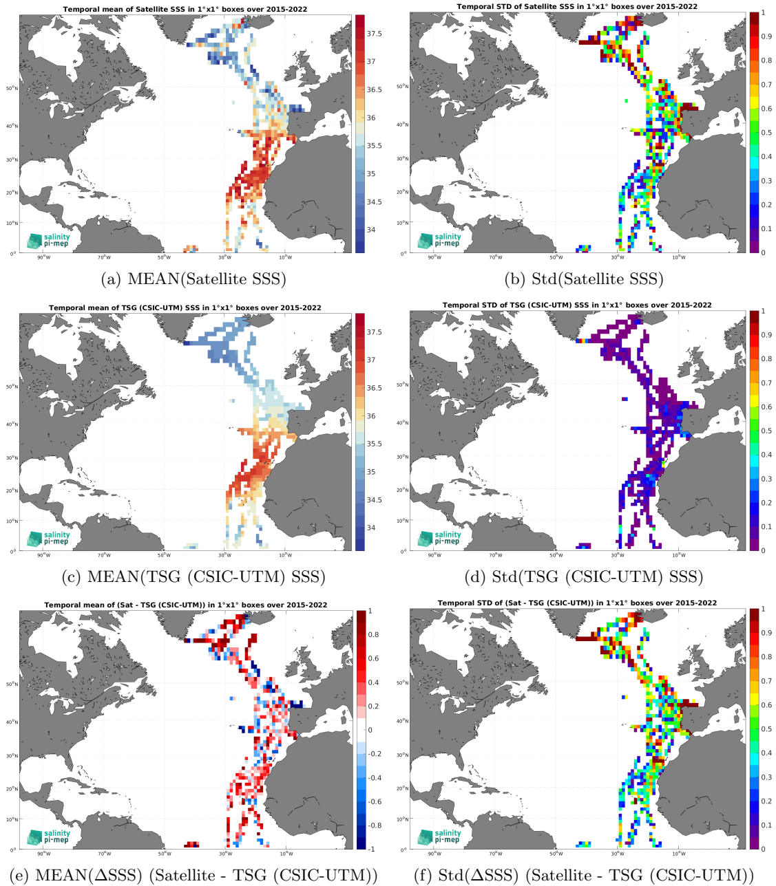
Figure 6: Temporal mean (left) and Std (right) of SSS from SMAP SSS L2 v5.0 (JPL) (top), TSG (CSIC-UTM) (middle), and of \Delta SSS (Satellite - TSG (CSIC-UTM)). Only match-up pairs are used to generate these maps.
