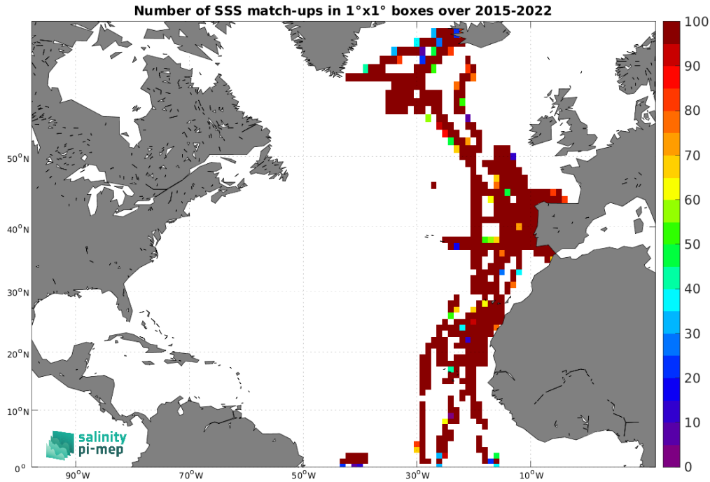
Figure 4: Number of SSS match-ups between TSG (CSIC-UTM) SSS and the SMAP SSS L2 v5.0 (JPL) SSS product for the North Atlantic Ocean Pi-MEP region over 1^\circ \times 1^\circ boxes and for the full satellite product period.
