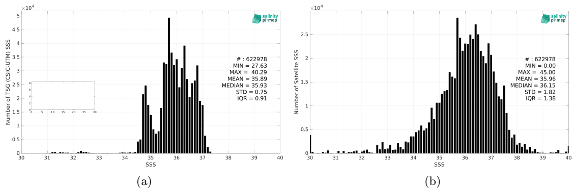
Figure 2: Histograms of SSS from TSG (CSIC-UTM) (a) and SMAP SSS L2 v5.0 (JPL) (b) considering all match-up pairs per bins of 0.1 over the North Atlantic Ocean Pi-MEP region and for the full satellite product period.
