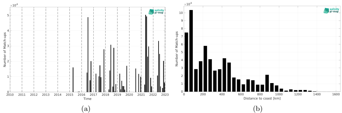
Figure 1: Number of match-ups between TSG (CSIC-UTM) and SMAP SSS L2 v5.0 (JPL) SSS as a function of time (a) and as function of the distance to coast (b) over the North Atlantic Ocean Pi-MEP region and for the full satellite product period.
