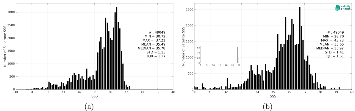
Figure 3: Histograms of SSS from Saildrone (a) and SMAP SSS L2 v5.0 (JPL) (b) considering all match-up pairs per bins of 0.1 over the North Atlantic Ocean Pi-MEP region and for the full satellite product period.
