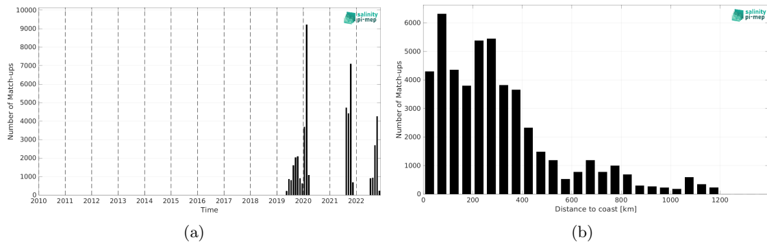
Figure 2: Number of match-ups between Saildrone and SMAP SSS L2 v5.0 (JPL) SSS as a function of time (a) and as function of the distance to coast (b) over the North Atlantic Ocean Pi-MEP region and for the full satellite product period.
