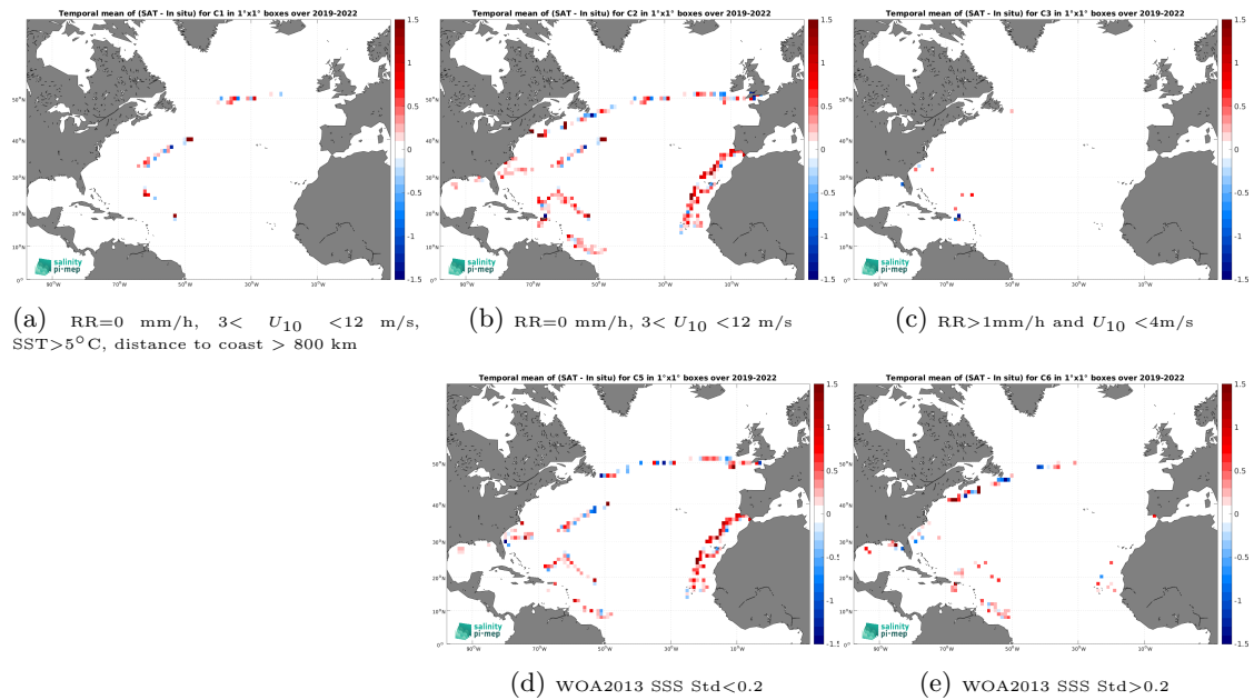
Figure 12: Temporal mean gridded over spatial boxes of size 1^\circ \times 1^\circ of \Delta\text{SSS} (SMAP SSS L2 v5.0 (JPL) - Saildrone) for 5 different subdatasets corresponding to:RR=0 mm/h, 3 < U_{10} < 12 m/s, SST > 5^\circ\text{C} , distance to coast > 800 km (a), RR=0 mm/h, 3 < U_{10} < 12 m/s (b), RR > 1 mm/h and U_{10} < 4 m/s (c), WOA2013 SSS Std < 0.2 (d), WOA2013 SSS Std > 0.2 (e).
