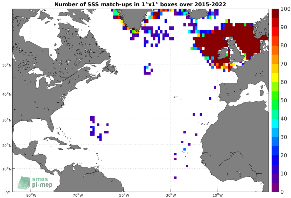
Figure 4: Number of SSS match-ups between ICES SSS and the SMAP SSS L2 v5.0 (JPL) SSS product for the North Atlantic Ocean Pi-MEP region over 1^\circ \times 1^\circ boxes and for the full satellite product period.
