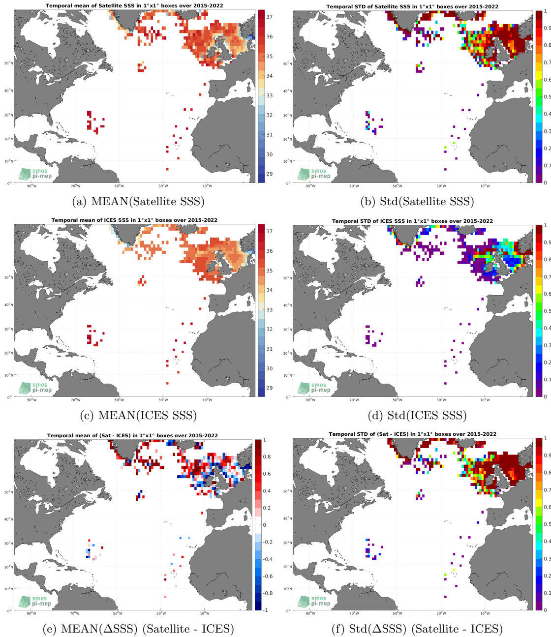
Figure 6: Temporal mean (left) and Std (right) of SSS from SMAP SSS L2 v5.0 (JPL) (top), ICES (middle), and of \Delta SSS (Satellite - ICES). Only match-up pairs are used to generate these maps.
