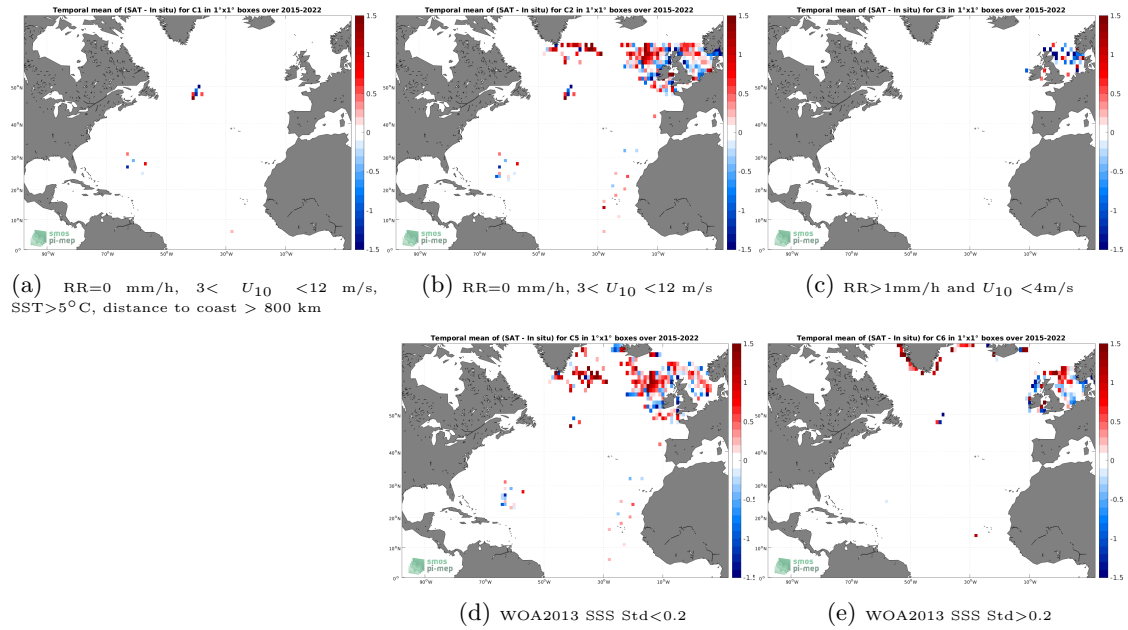
Figure 12: Temporal mean gridded over spatial boxes of size 1^\circ \times 1^\circ of \Delta SSS (SMAP SSS L2 v5.0 (JPL) - ICES) for 5 different subdatasets corresponding to:RR=0 mm/h, 3 < U_{10} < 12 m/s, SST >5^\circ C, distance to coast > 800 km (a), RR=0 mm/h, 3 < U_{10} < 12 m/s (b), RR >1 mm/h and U_{10} < 4 m/s (c), WOA2013 SSS Std <0.2 (d), WOA2013 SSS Std >0.2 (e).
