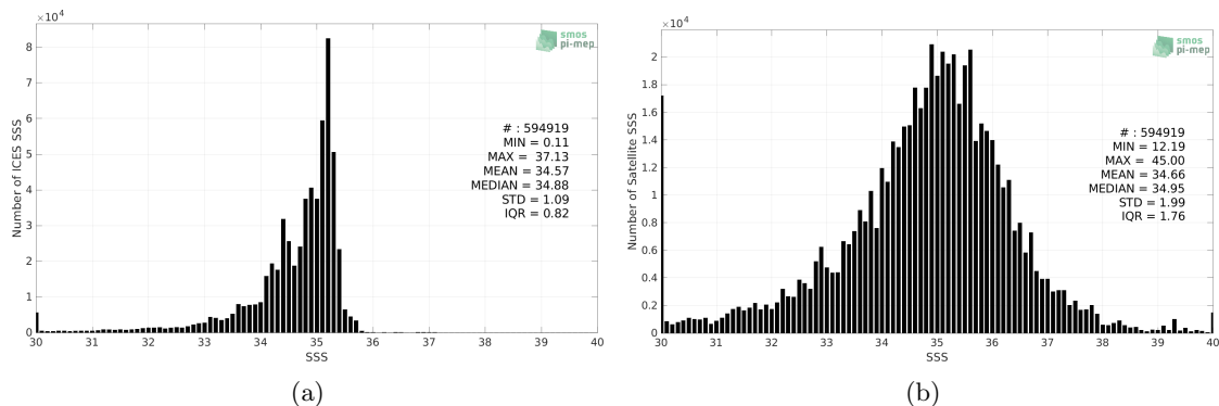
Figure 2: Histograms of SSS from ICES (a) and SMAP SSS L2 v5.0 (JPL) (b) considering all match-up pairs per bins of 0.1 over the North Atlantic Ocean Pi-MEP region and for the full satellite product period.
