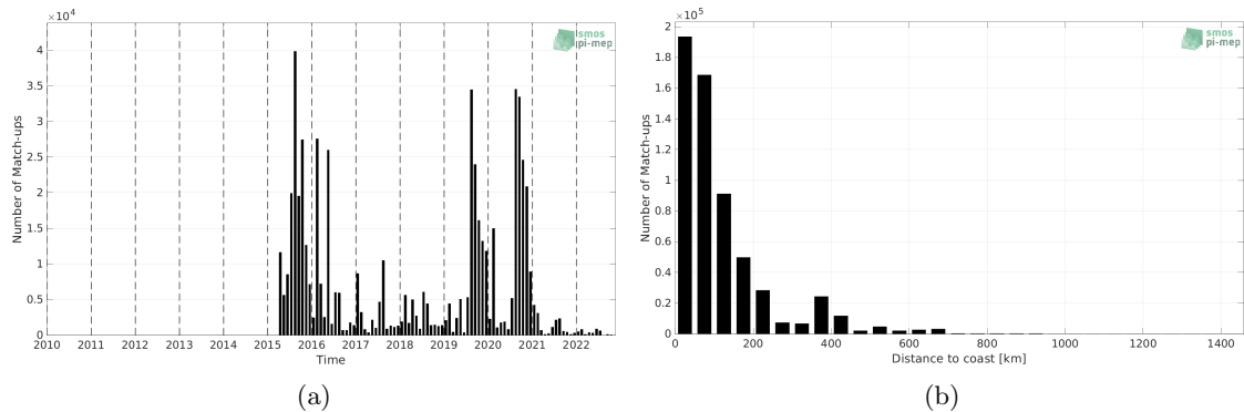
Figure 1: Number of match-ups between ICES and SMAP SSS L2 v5.0 (JPL) SSS as a function of time (a) and as function of the distance to coast (b) over the North Atlantic Ocean Pi-MEP region and for the full satellite product period.
