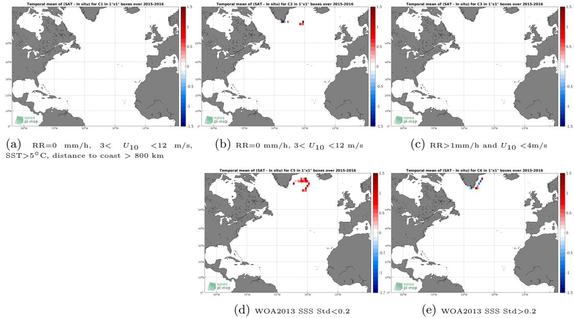
Figure 11: Temporal mean gridded over spatial boxes of size 1^{\circ}\times 1^{\circ} of \Delta\text{SSS} (SMAP SSS L2 v5.0 (JPL) - Surface drifters) for 5 different subdatasets corresponding to:RR=0 mm/h, 3 < U_{10} < 12 m/s, SST >5^{\circ}\text{C} , distance to coast > 800 km (a), RR=0 mm/h, 3 < U_{10} < 12 m/s (b), RR >1 mm/h and U_{10} < 4 m/s (c), WOA2013 SSS Std <0.2 (d), WOA2013 SSS Std >0.2 (e).
