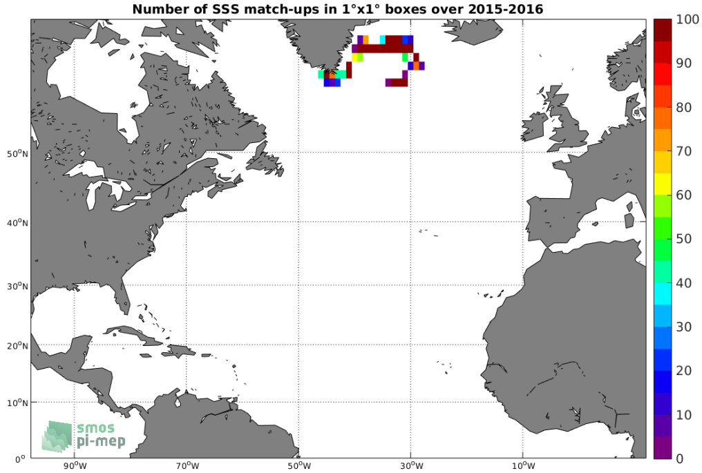
Figure 3: Number of SSS match-ups between Surface drifters SSS and the SMAP SSS L2 v5.0 (JPL) SSS product for the North Atlantic Ocean Pi-MEP region over 1°x1° boxes and for the full satellite product period.
