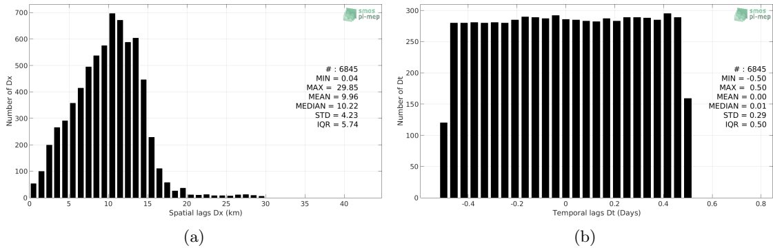
Figure 4: Histograms of the spatial (a) and temporal (b) lags between the time of the Surface drifters measurements and the date of the corresponding SMAP SSS L2 v5.0 (JPL) SSS product.
