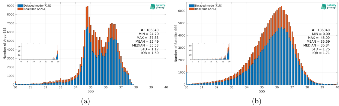
Figure 3: Histograms of SSS from Argo (a) and SMAP SSS L2 v5.0 (JPL) (b) considering all match-up pairs per bins of 0.1 over the North Atlantic Ocean Pi-MEP region and for the full satellite product period.
