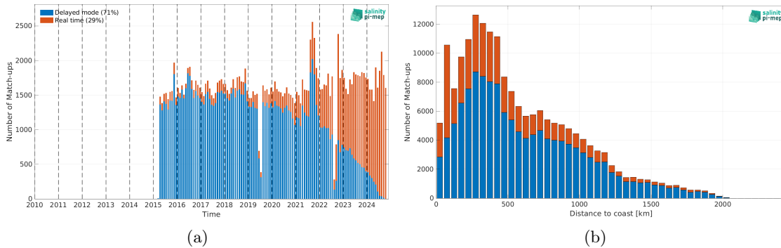
Figure 2: Number of match-ups between Argo and SMAP SSS L2 v5.0 (JPL) SSS as a function of time (a) and as function of the distance to coast (b) over the North Atlantic Ocean Pi-MEP region and for the full satellite product period.
