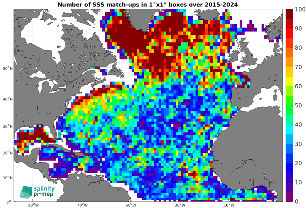
Figure 5: Number of SSS match-ups between Argo SSS and the SMAP SSS L2 v5.0 (JPL) SSS product for the North Atlantic Ocean Pi-MEP region over 1^\circ \times 1^\circ boxes and for the full satellite product period.
