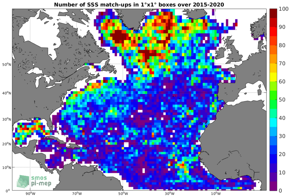
Figure 4: Number of SSS match-ups between Argo SSS and the SMAP SSS L2 v5.0 (JPL) SSS product for the North Atlantic Ocean Pi-MEP region over 1°x1° boxes and for the full satellite product period.
