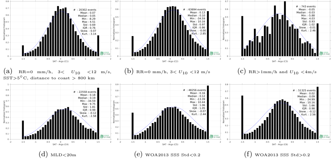
Figure 13: Normalized histogram of \Delta SSS (SMAP SSS L2 v5.0 (JPL) - Argo) for 6 different subdatasets corresponding to: RR=0 mm/h, 3 < U_{10} < 12 m/s, SST>5°C, distance to coast > 800 km (a), RR=0 mm/h, 3 < U_{10} < 12 m/s (b), RR>1mm/h and U_{10} < 4 m/s (c), MLD<20m (d), WOA2013 SSS Std<0.2 (e), WOA2013 SSS Std>0.2 (f).
