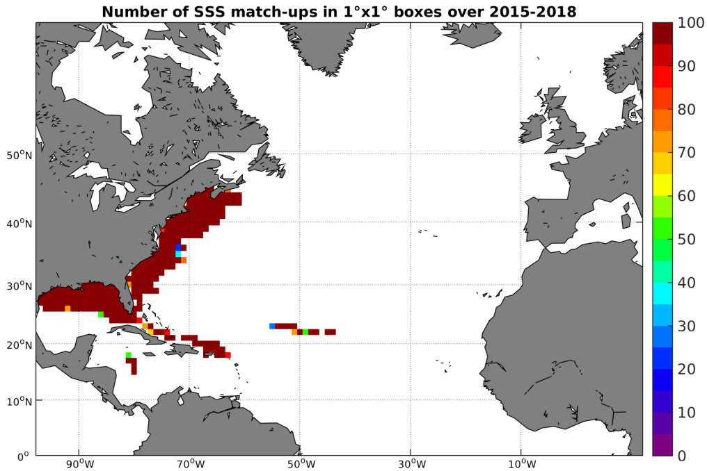
Figure 4: Number of SSS match-ups between TSG-SAMOS SSS and the SMAP-L2-JPL-V4 SSS product for the North Atlantic Ocean Pi-MEP region over 1^\circ \times 1^\circ boxes and for the full satellite product period.
