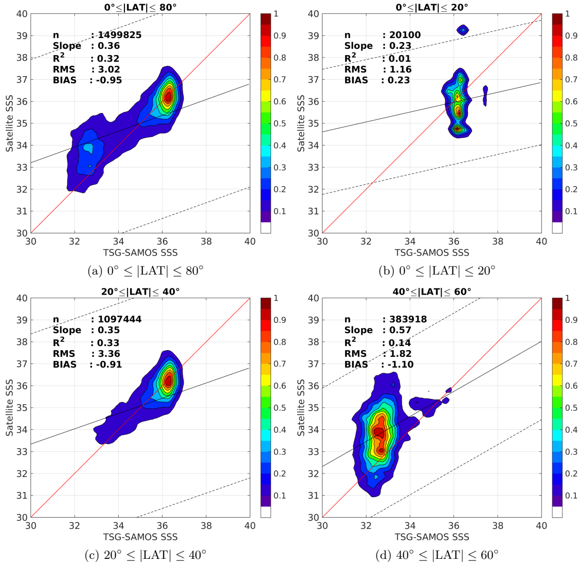
Figure 9: Contour maps of the concentration of SMAP-L2-JPL-V4 SSS (y-axis) versus TSG-SAMOS SSS (x-axis) at match-up pairs for different latitude bands. For each plot, the red line shows x=y . The black thin and dashed lines indicate a linear fit through the data cloud and the \pm 95\% confidence levels, respectively. The number match-up pairs n , the slope and R^2 coefficient of the linear fit, the root mean square (RMS) and the mean bias between satellite and in situ data are indicated for each latitude band in each plots.
