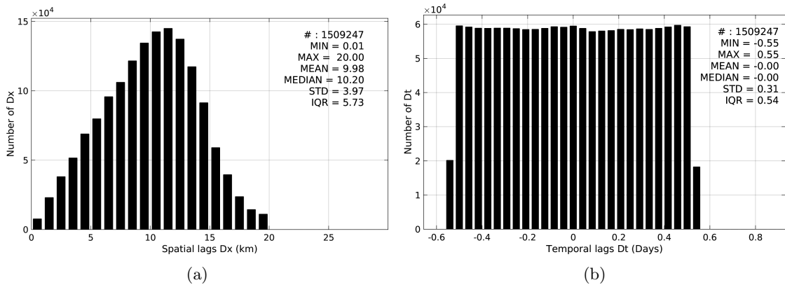
Figure 5: Histograms of the spatial (a) and temporal (b) lags between the time of the TSG-SAMOS measurements and the date of the corresponding SMAP-L2-JPL-V4 SSS product.
