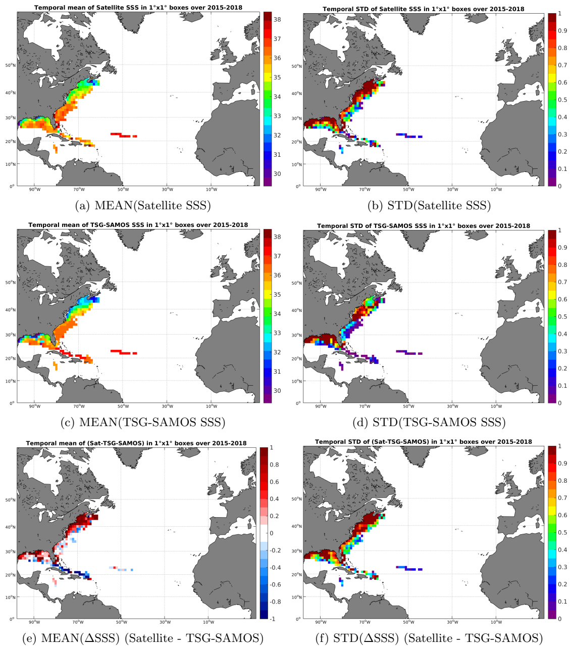
Figure 6: Temporal mean (left) and STD (right) of SSS from SMAP-L2-JPL-V4 (top), TSG-SAMOS (middle), and of \Delta SSS (Satellite - TSG-SAMOS). Only match-up pairs are used to generate these maps.
