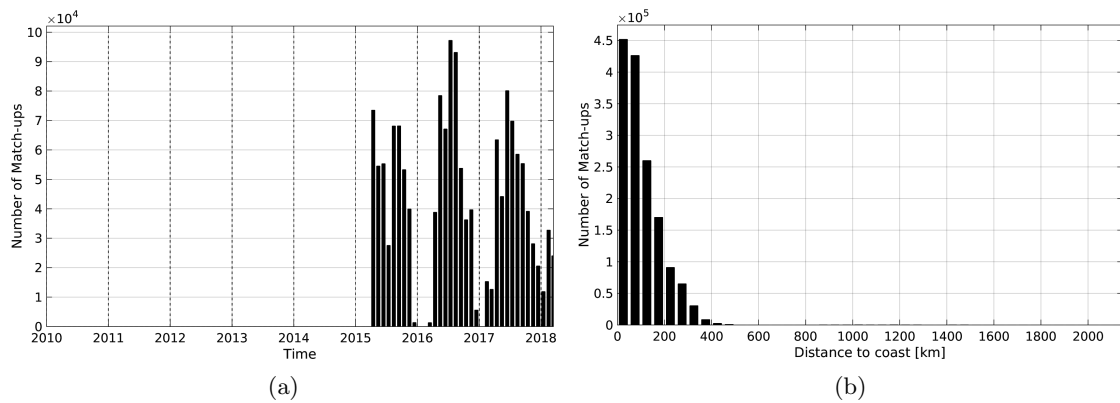
Figure 1: Number of match-ups between TSG-SAMOS and SMAP-L2-JPL-V4 SSS as a function of time (a) and as function of the distance to coast (b) over the North Atlantic Ocean Pi-MEP region and for the full satellite product period.
