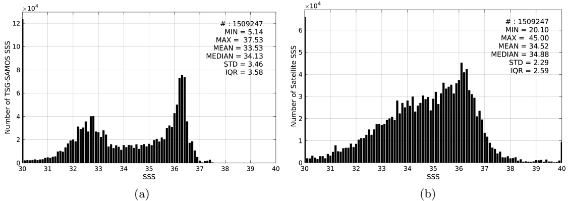
Figure 2: Histograms of SSS from TSG-SAMOS (a) and SMAP-L2-JPL-V4 (b) considering all match-up pairs per bins of 0.1 over the North Atlantic Ocean Pi-MEP region and for the full satellite product period.
