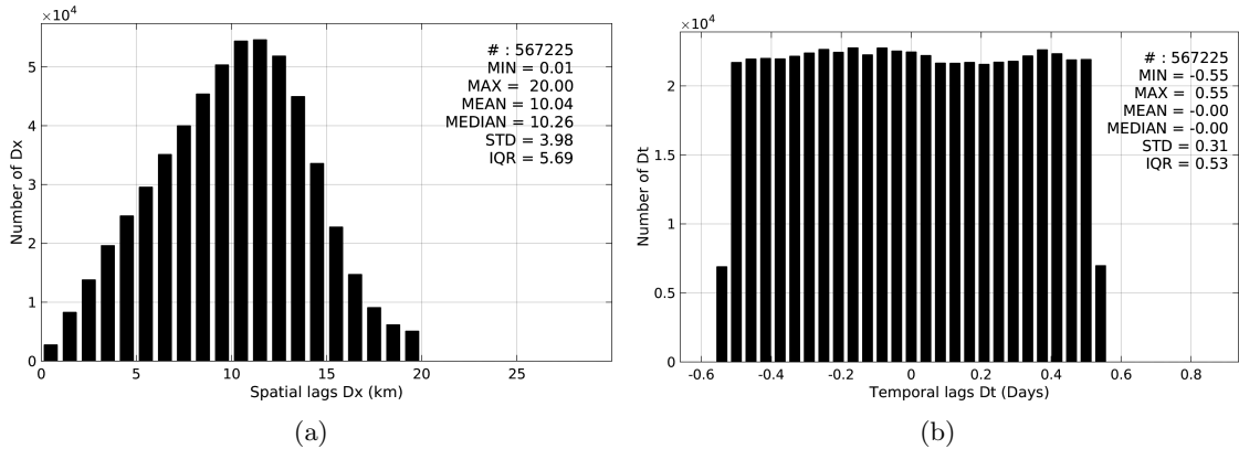
Figure 5: Histograms of the spatial (a) and temporal (b) lags between the time of the TSG-LEGOS-DM measurements and the date of the corresponding SMAP-L2-JPL-V4 SSS product.
