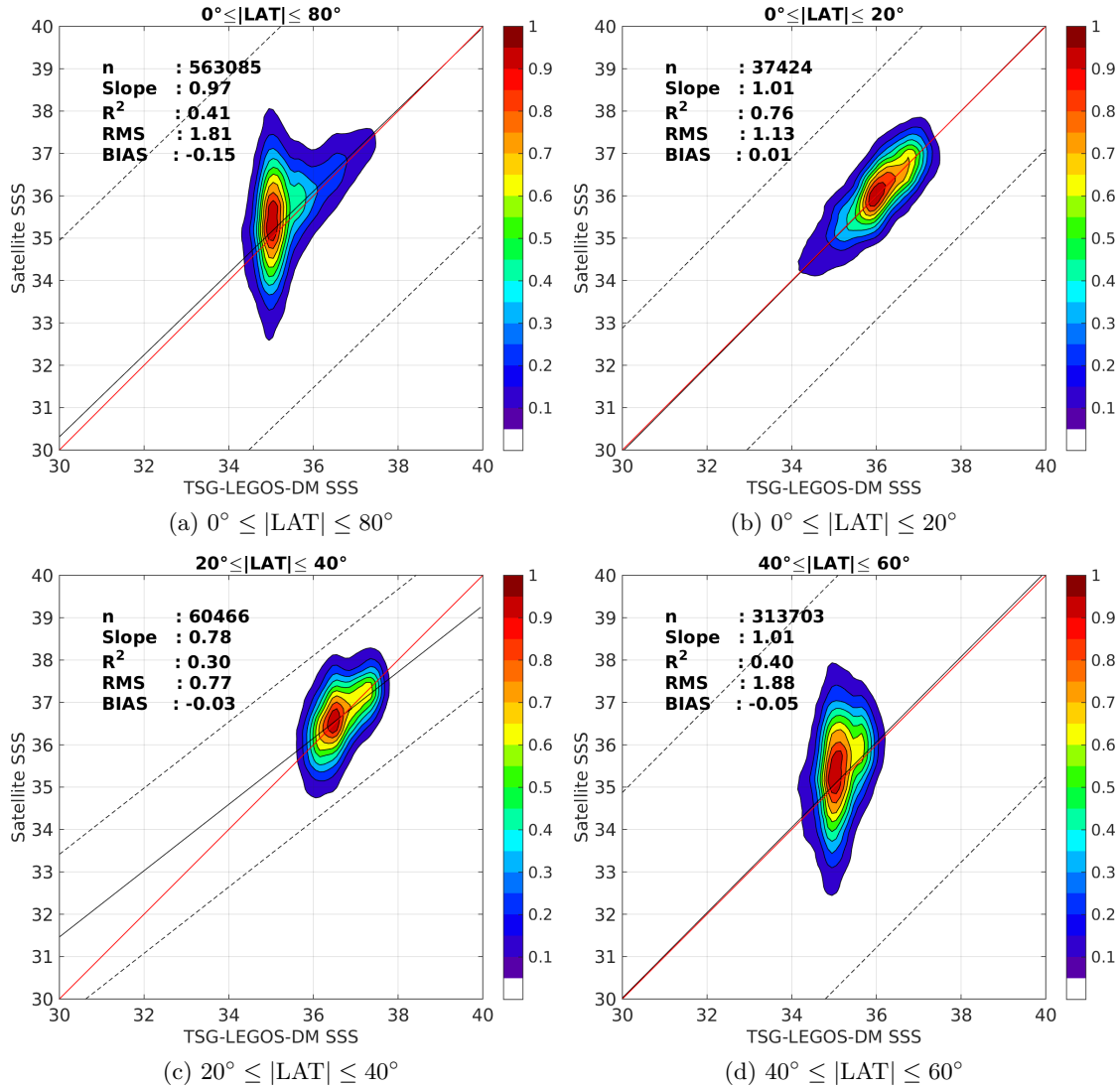
Figure 9: Contour maps of the concentration of SMAP-L2-JPL-V4 SSS (y-axis) versus TSG-LEGOS-DM SSS (x-axis) at match-up pairs for different latitude bands. For each plot, the red line shows x=y . The black thin and dashed lines indicate a linear fit through the data cloud and the \pm 95\% confidence levels, respectively. The number match-up pairs n , the slope and R^2 coefficient of the linear fit, the root mean square (RMS) and the mean bias between satellite and in situ data are indicated for each latitude band in each plots.
