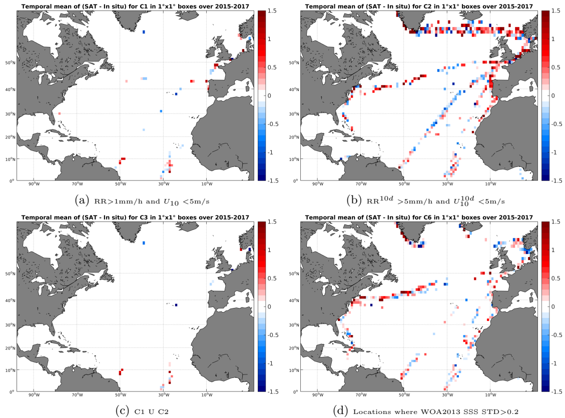
Figure 12: Temporal mean gridded over spatial boxes of size 1^\circ \times 1^\circ of \Delta SSS (SMAP-L2-JPL-V4 - TSG-LEGOS-DM) for 4 different subdatasets corresponding to:RR > 1mm/h and U_{10} < 5 m/s (a), RR 10d > 5mm/h and U_{10}^{10d} < 5 m/s (b), C1 U C2 (c),Locations where WOA2013 SSS STD > 0.2 (d).
