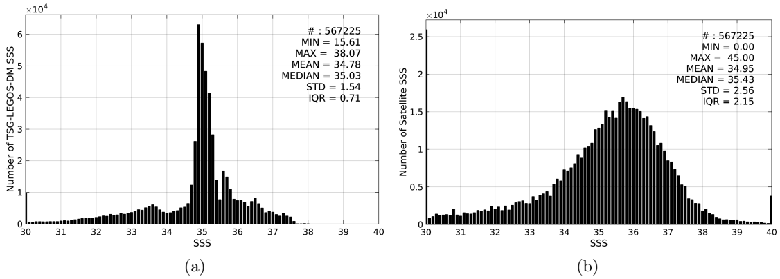
Figure 2: Histograms of SSS from TSG-LEGOS-DM (a) and SMAP-L2-JPL-V4 (b) considering all match-up pairs per bins of 0.1 over the North Atlantic Ocean Pi-MEP region and for the full satellite product period.
