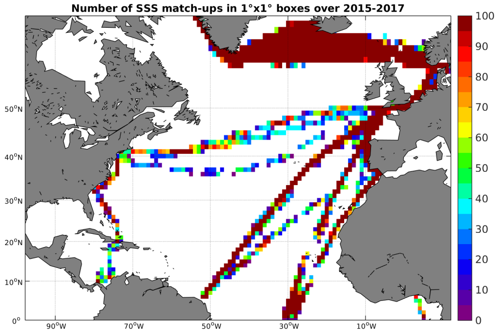
Figure 4: Number of SSS match-ups between TSG-LEGOS-DM SSS and the SMAP-L2-JPL-V4 SSS product for the North Atlantic Ocean Pi-MEP region over 1^\circ \times 1^\circ boxes and for the full satellite product period.
