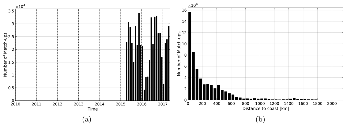
Figure 1: Number of match-ups between TSG-LEGOS-DM and SMAP-L2-JPL-V4 SSS as a function of time (a) and as function of the distance to coast (b) over the North Atlantic Ocean Pi-MEP region and for the full satellite product period.
