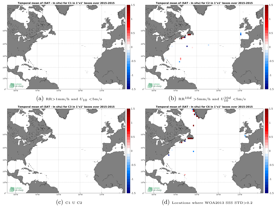
Figure 12: Temporal mean gridded over spatial boxes of size 1^\circ \times 1^\circ of \Delta SSS (SMAP-L2-JPL-V4 - TSG-GOSUD-Sailing-ship) for 4 different subdatasets corresponding to: RR > 1\text{mm/h} and U_{10} < 5\text{m/s} (a), RR^{10d} > 5\text{mm/h} and U_{10}^{10d} < 5\text{m/s} (b), C1 U C2 (c), Locations where WOA2013 SSS STD > 0.2 (d).
