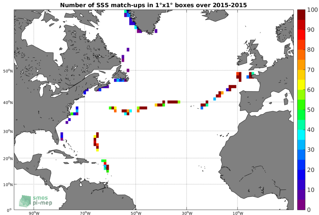
Figure 4: Number of SSS match-ups between TSG-GOSUD-Sailing-ship SSS and the SMAP-L2-JPL-V4 SSS product for the North Atlantic Ocean Pi-MEP region over 1°x1° boxes and for the full satellite product period.
