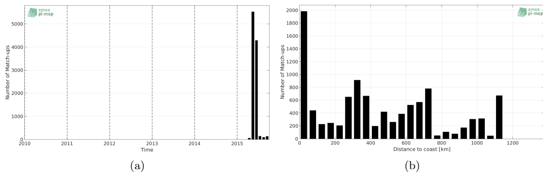
Figure 1: Number of match-ups between TSG-GOSUD-Sailing-ship and SMAP-L2-JPL-V4 SSS as a function of time (a) and as function of the distance to coast (b) over the North Atlantic Ocean Pi-MEP region and for the full satellite product period.
