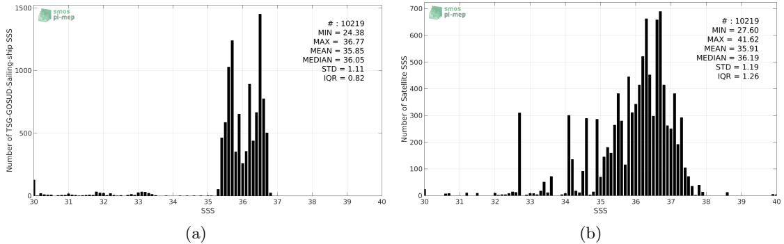
Figure 2: Histograms of SSS from TSG-GOSUD-Sailing-ship (a) and SMAP-L2-JPL-V4 (b) considering all match-up pairs per bins of 0.1 over the North Atlantic Ocean Pi-MEP region and for the full satellite product period.
