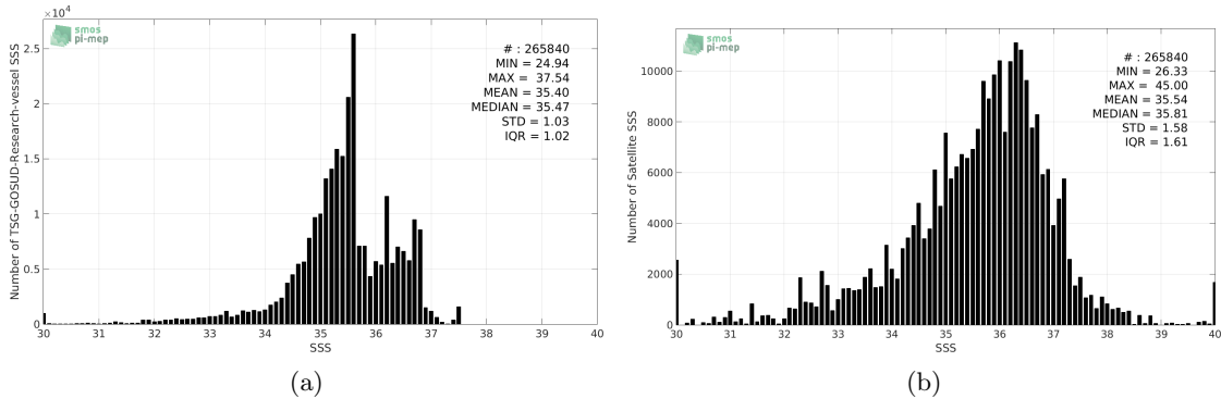
Figure 2: Histograms of SSS from TSG-GOSUD-Research-vessel (a) and SMAP-L2-JPL-V4 (b) considering all match-up pairs per bins of 0.1 over the North Atlantic Ocean Pi-MEP region and for the full satellite product period.
