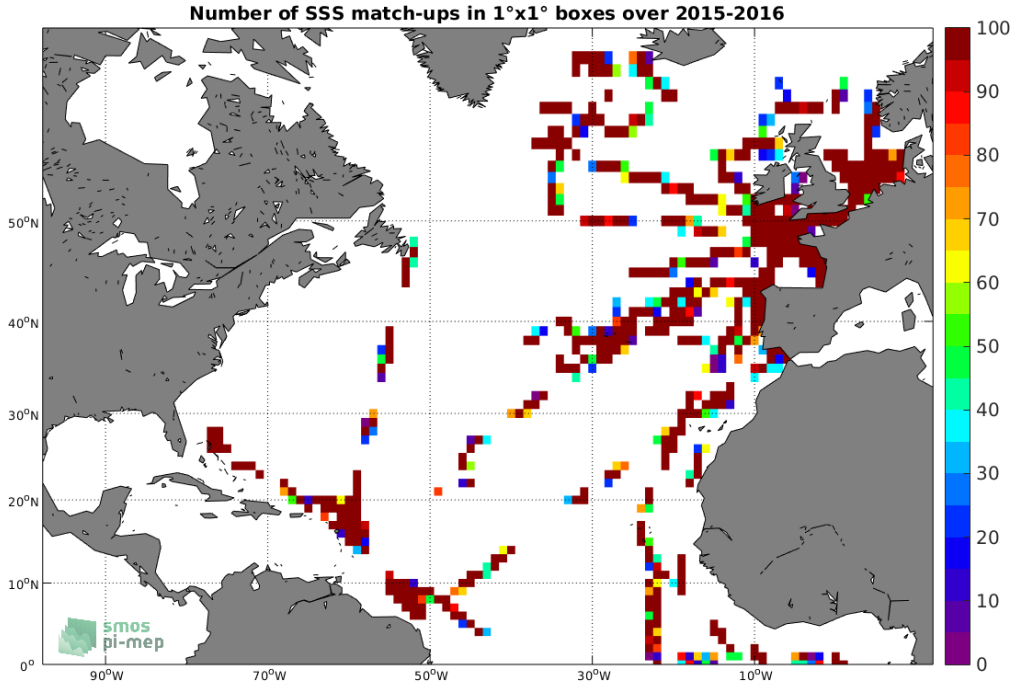
Figure 4: Number of SSS match-ups between TSG-GOSUD-Research-vessel SSS and the SMAP-L2-JPL-V4 SSS product for the North Atlantic Ocean Pi-MEP region over 1°x1° boxes and for the full satellite product period.
