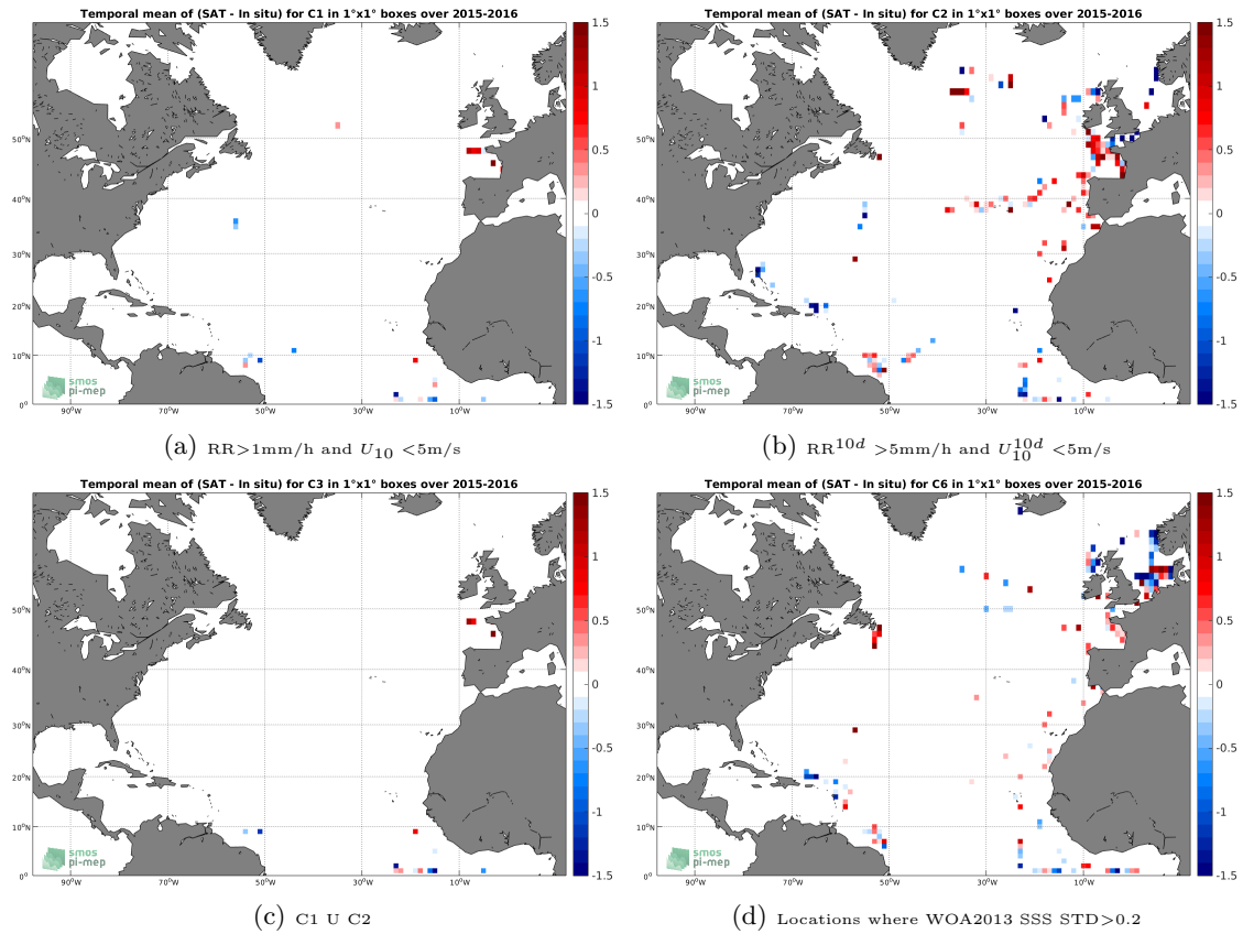
Figure 12: Temporal mean gridded over spatial boxes of size 1^\circ \times 1^\circ of \Delta SSS (SMAP-L2-JPL-V4 - TSG-GOSUD-Research-vessel) for 4 different subdatasets corresponding to: RR > 1\text{mm/h} and U_{10} < 5\text{m/s} (a), RR^{10d} > 5\text{mm/h} and U_{10}^{10d} < 5\text{m/s} (b), C1 U C2 (c), Locations where WOA2013 SSS STD > 0.2 (d).
