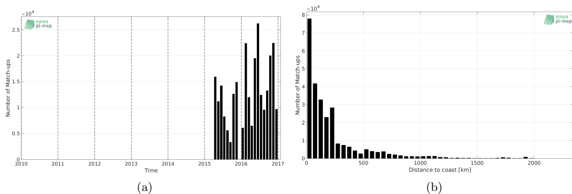
Figure 1: Number of match-ups between TSG-GOSUD-Research-vessel and SMAP-L2-JPL-V4 SSS as a function of time (a) and as function of the distance to coast (b) over the North Atlantic Ocean Pi-MEP region and for the full satellite product period.
