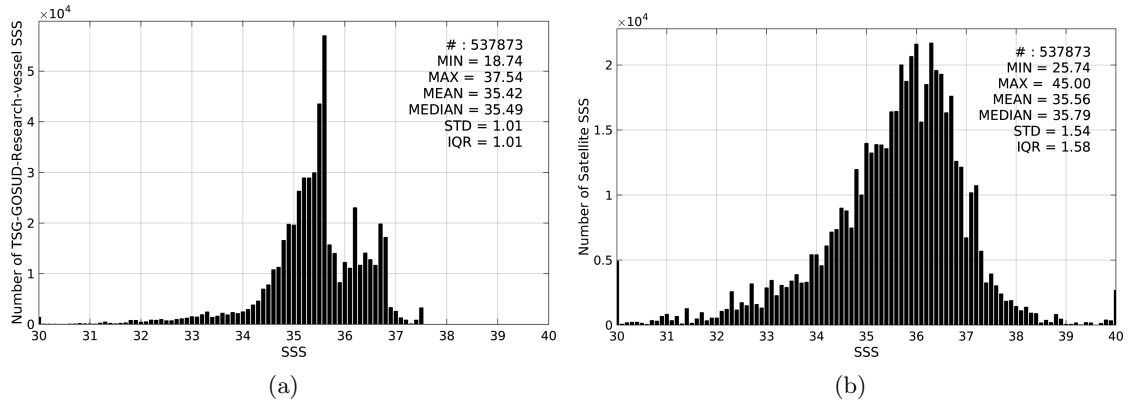
Figure 2: Histograms of SSS from TSG-GOSUD-Research-vessel (a) and SMAP-L2-JPL-V4 (b) considering all match-up pairs per bins of 0.1 over the North Atlantic Ocean Pi-MEP region and for the full satellite product period.
