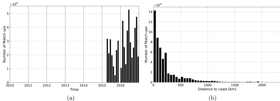
Figure 1: Number of match-ups between TSG-GOSUD-Research-vessel and SMAP-L2-JPL-V4 SSS as a function of time (a) and as function of the distance to coast (b) over the North Atlantic Ocean Pi-MEP region and for the full satellite product period.
