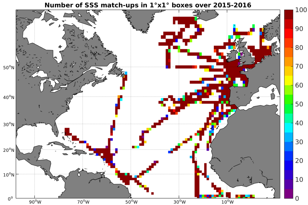
Figure 4: Number of SSS match-ups between TSG-GOSUD-Research-vessel SSS and the SMAP-L2-JPL-V4 SSS product for the North Atlantic Ocean Pi-MEP region over 1^\circ \times 1^\circ boxes and for the full satellite product period.
