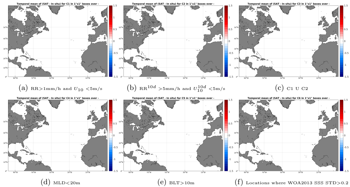
Figure 12: Temporal mean gridded over spatial boxes of size 1^\circ \times 1^\circ of \Delta SSS (SMAP-L2-JPL-V4 - Sea mammals) for 6 different subdatasets corresponding to:RR>1mm/h and U_{10} < 5m/s (a), RR^{10d} > 5mm/h and U_{10}^{10d} < 5m/s (b), C1 U C2 (c),MLD<20m (d),BLT>10m (e),Locations where WOA2013 SSS STD>0.2 (f).
