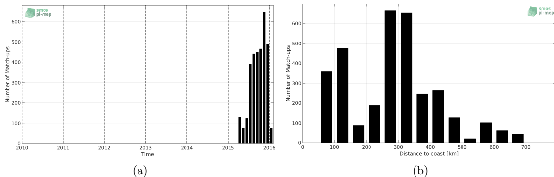
Figure 1: Number of match-ups between Surface drifters and SMAP-L2-JPL-V4 SSS as a function of time (a) and as function of the distance to coast (b) over the North Atlantic Ocean Pi-MEP region and for the full satellite product period.
