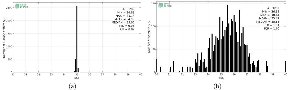
Figure 2: Histograms of SSS from Surface drifters (a) and SMAP-L2-JPL-V4 (b) considering all match-up pairs per bins of 0.1 over the North Atlantic Ocean Pi-MEP region and for the full satellite product period.
