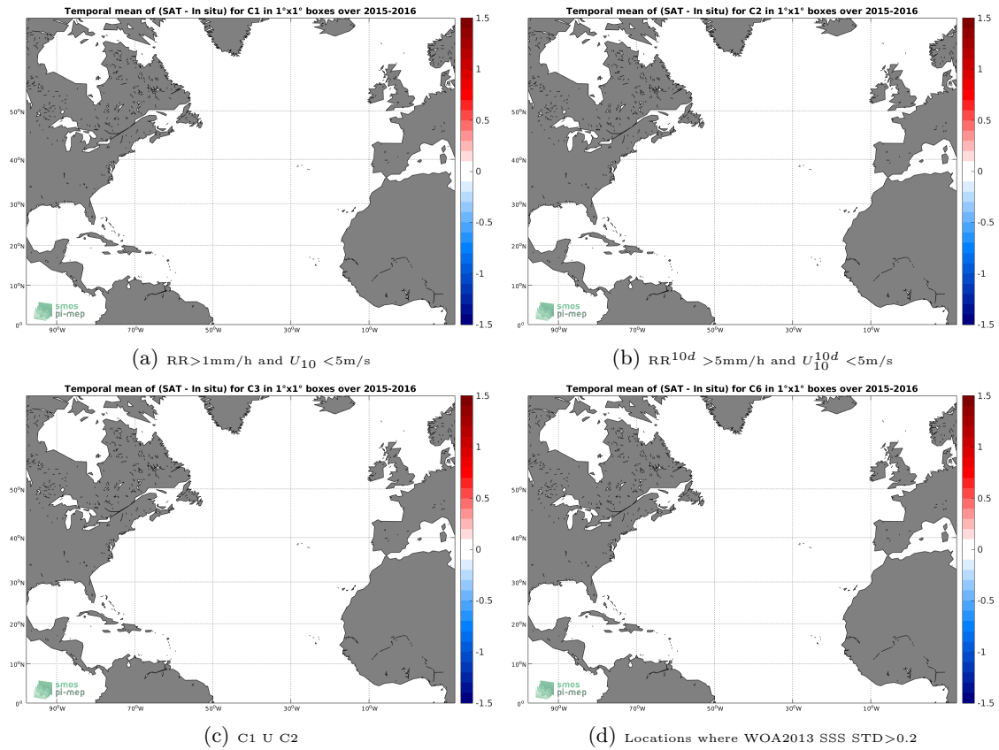
Figure 11: Temporal mean gridded over spatial boxes of size 1^\circ \times 1^\circ of \Delta SSS (SMAP-L2-JPL-V4 - Surface drifters) for 4 different subdatasets corresponding to: RR > 1\text{mm/h} and U_{10} < 5\text{m/s} (a), RR^{10d} > 5\text{mm/h} and U_{10}^{10d} < 5\text{m/s} (b), C1 U C2 (c), Locations where WOA2013 SSS STD > 0.2 (d).
