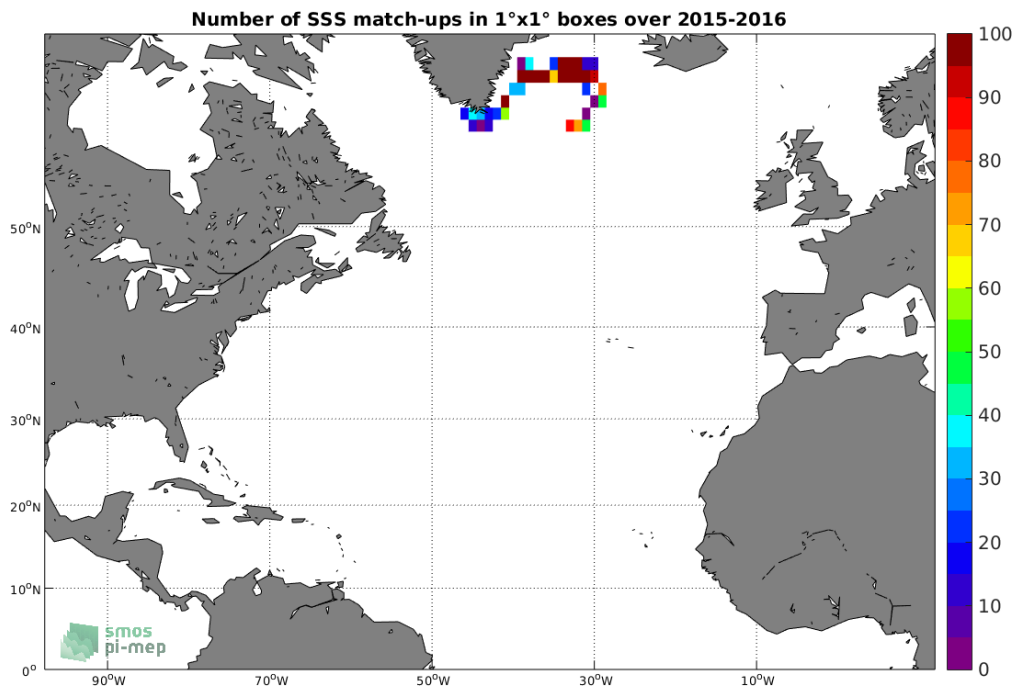
Figure 3: Number of SSS match-ups between Surface drifters SSS and the SMAP-L2-JPL-V4 SSS product for the North Atlantic Ocean Pi-MEP region over 1°x1° boxes and for the full satellite product period.
