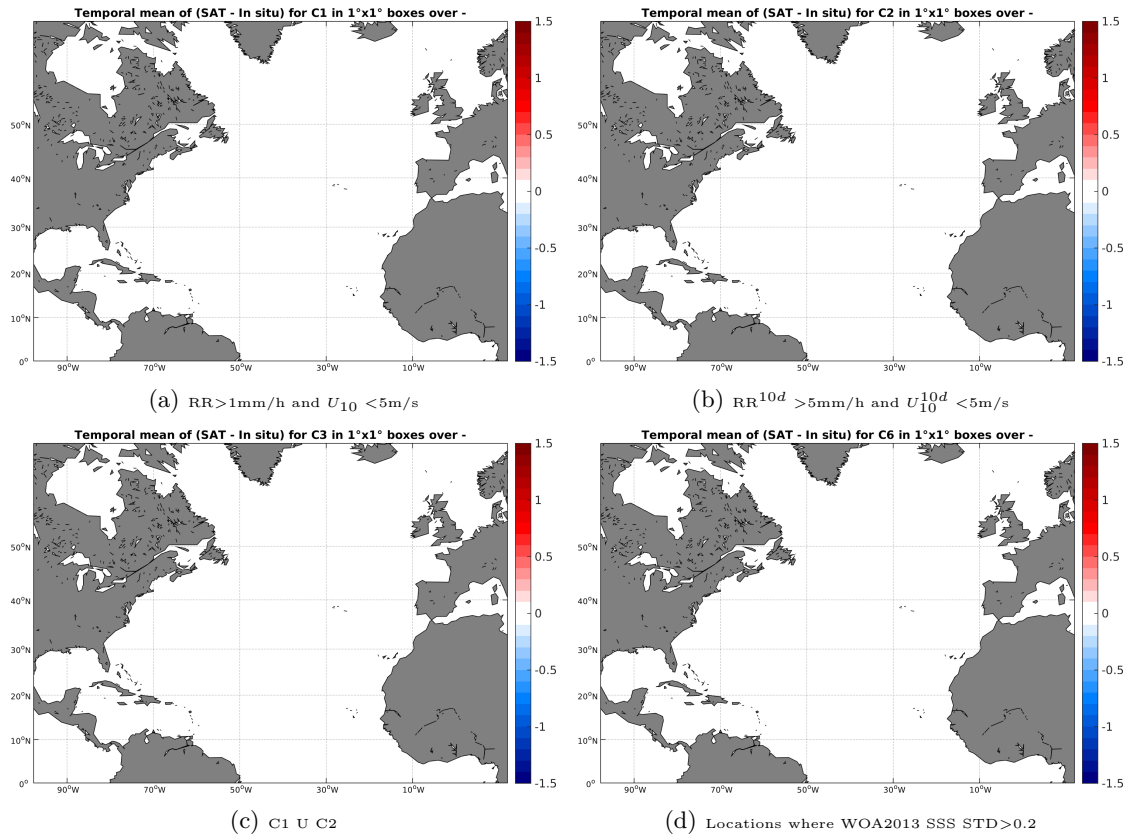
Figure 11: Temporal mean gridded over spatial boxes of size 1^\circ \times 1^\circ of \Delta SSS (SMAP-L2-JPL-V4 - Surface drifters) for 4 different subdatasets corresponding to: RR > 1mm/h and U_{10} < 5 m/s (a), RR^{10d} > 5 mm/h and U_{10}^{10d} < 5 m/s (b), C1 U C2 (c), Locations where WOA2013 SSS STD > 0.2 (d).
