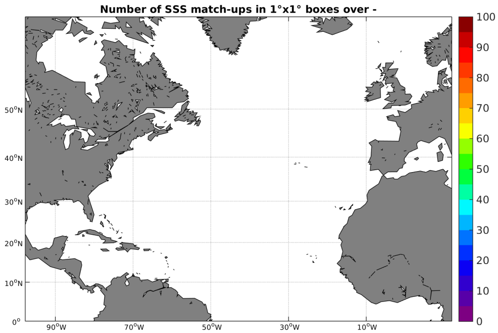
Figure 3: Number of SSS match-ups between Surface drifters SSS and the SMAP-L2-JPL-V4 SSS product for the North Atlantic Ocean Pi-MEP region over 1^\circ \times 1^\circ boxes and for the full satellite product period.
