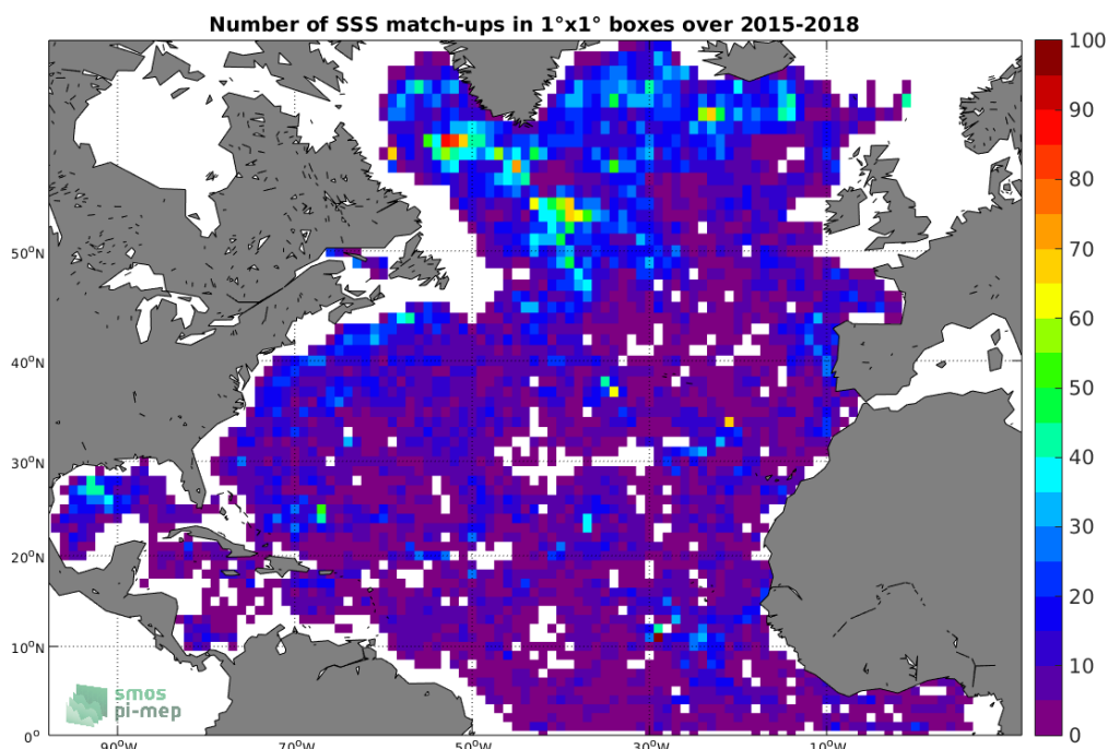
Figure 4: Number of SSS match-ups between Argo SSS and the SMAP-L2-JPL-V4 SSS product for the North Atlantic Ocean Pi-MEP region over 1°x1° boxes and for the full satellite product period.
