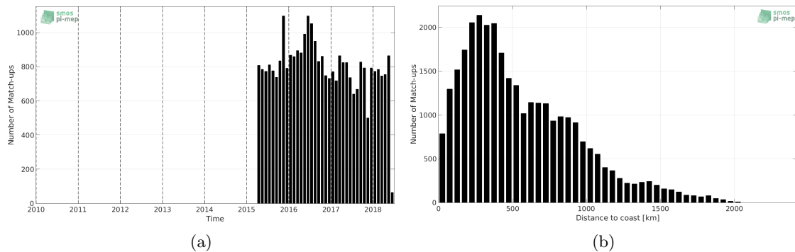
Figure 1: Number of match-ups between Argo and SMAP-L2-JPL-V4 SSS as a function of time (a) and as function of the distance to coast (b) over the North Atlantic Ocean Pi-MEP region and for the full satellite product period.
