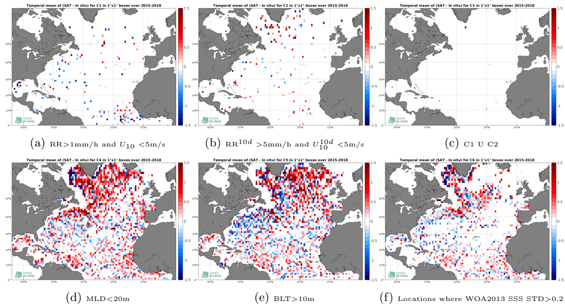
Figure 12: Temporal mean gridded over spatial boxes of size 1^\circ \times 1^\circ of \Delta\text{SSS} (SMAP-L2-JPL-V4 - Argo) for 6 different subdatasets corresponding to: RR > 1\text{mm/h} and U_{10} < 5\text{m/s} (a), RR^{10d} > 5\text{mm/h} and U_{10}^{10d} < 5\text{m/s} (b), C1 U C2 (c), MLD < 20\text{m} (d), BLT > 10\text{m} (e), Locations where WOA2013 SSS STD > 0.2 (f).
