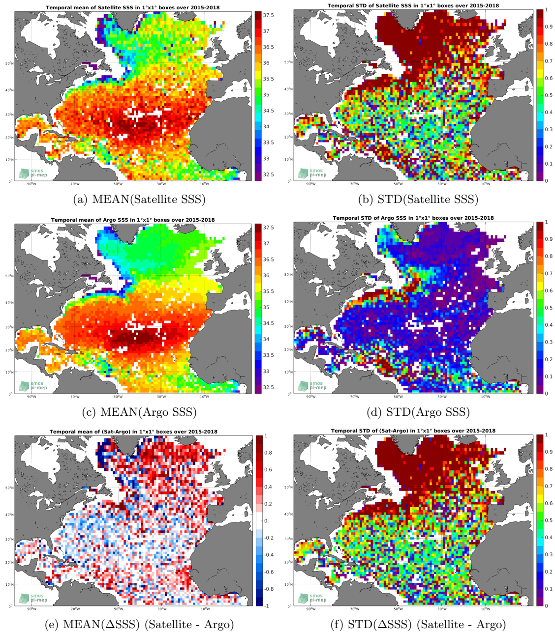
Figure 6: Temporal mean (left) and STD (right) of SSS from SMAP-L2-JPL-V4 (top), Argo (middle), and of \Delta SSS (Satellite - Argo). Only match-up pairs are used to generate these maps.
