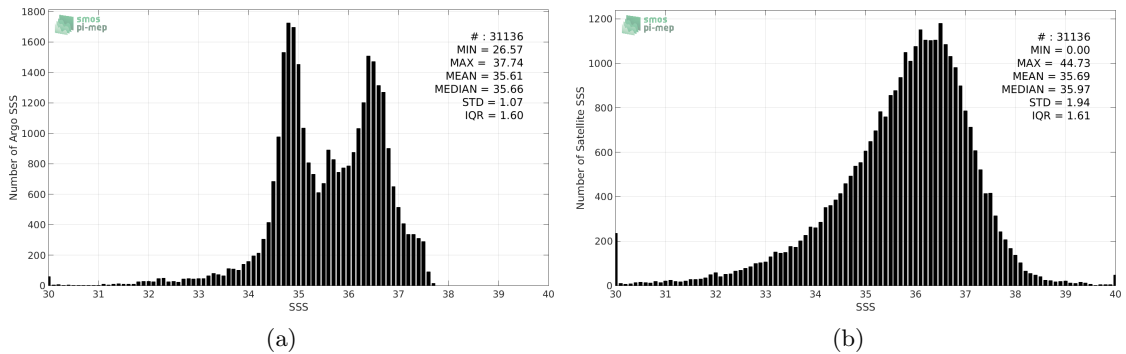
Figure 2: Histograms of SSS from Argo (a) and SMAP-L2-JPL-V4 (b) considering all match-up pairs per bins of 0.1 over the North Atlantic Ocean Pi-MEP region and for the full satellite product period.
