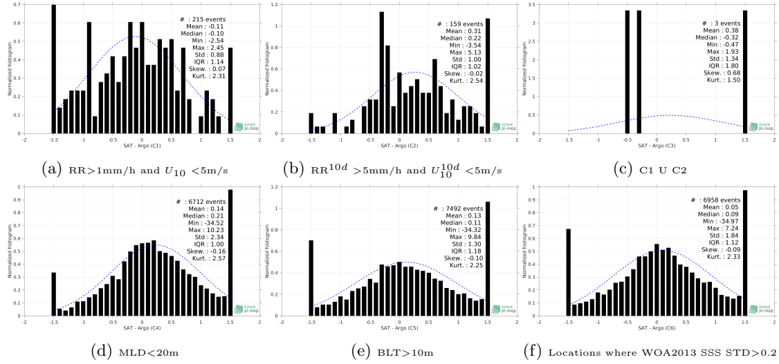
Figure 13: Normalized histogram of \Delta SSS (SMAP-L2-JPL-V4 - Argo) for 6 different subdatasets corresponding to: RR > 1\text{mm/h} and U_{10} < 5\text{m/s} (a), RR^{10d} > 5\text{mm/h} and U_{10}^{10d} < 5\text{m/s} (b), C1 U C2 (c), MLD < 20\text{m} (d), BLT > 10\text{m} (e), Locations where WOA2013 SSS STD > 0.2 (f).
