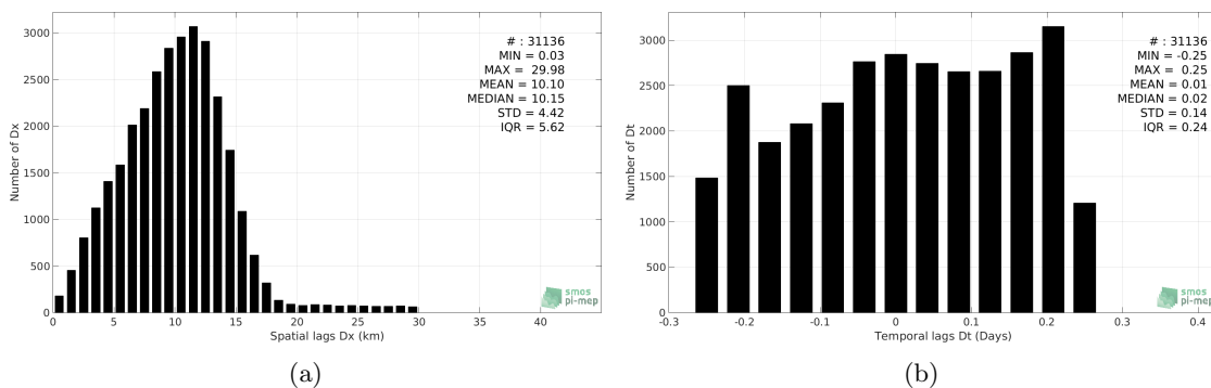
Figure 5: Histograms of the spatial (a) and temporal (b) lags between the time of the Argo measurements and the date of the corresponding SMAP-L2-JPL-V4 SSS product.
