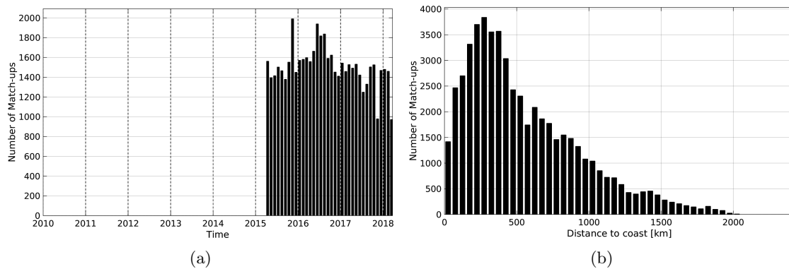
Figure 1: Number of match-ups between Argo and SMAP-L2-JPL-V4 SSS as a function of time (a) and as function of the distance to coast (b) over the North Atlantic Ocean Pi-MEP region and for the full satellite product period.
