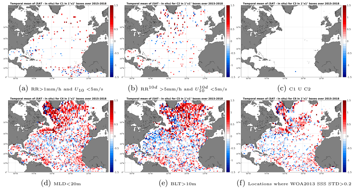
Figure 12: Temporal mean gridded over spatial boxes of size 1^\circ \times 1^\circ of \Delta\text{SSS} (SMAP-L2-JPL-V4 - Argo) for 6 different subdatasets corresponding to: RR > 1\text{mm/h} and U_{10} < 5\text{m/s} (a), RR^{10d} > 5\text{mm/h} and U_{10}^{10d} < 5\text{m/s} (b), C1 U C2 (c), MLD < 20\text{m} (d), BLT > 10\text{m} (e), Locations where WOA2013 SSS STD > 0.2 (f).
