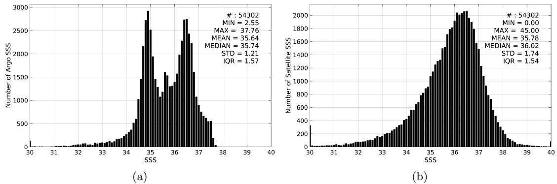
Figure 2: Histograms of SSS from Argo (a) and SMAP-L2-JPL-V4 (b) considering all match-up pairs per bins of 0.1 over the North Atlantic Ocean Pi-MEP region and for the full satellite product period.
