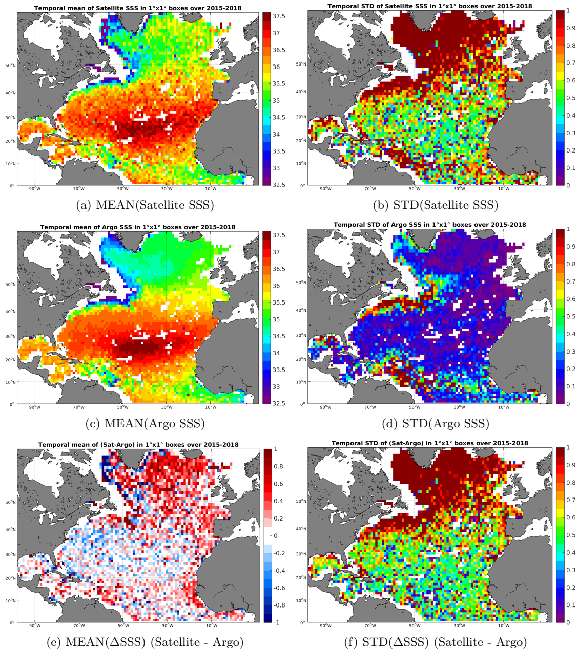
Figure 6: Temporal mean (left) and STD (right) of SSS from SMAP-L2-JPL-V4 (top), Argo (middle), and of \Delta SSS (Satellite - Argo). Only match-up pairs are used to generate these maps.
