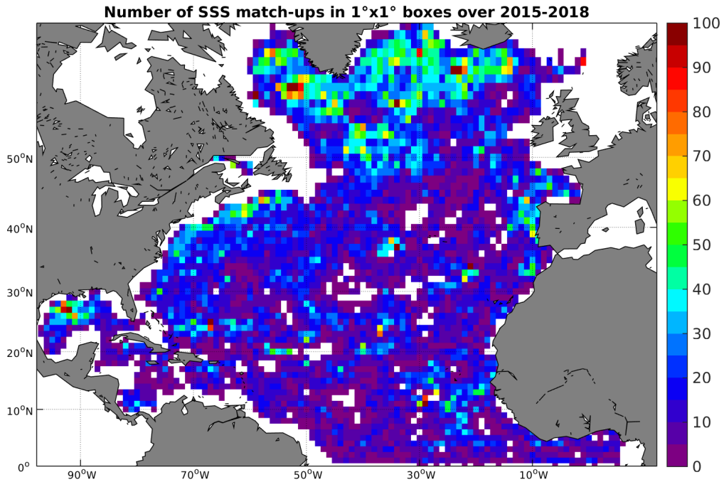
Figure 4: Number of SSS match-ups between Argo SSS and the SMAP-L2-JPL-V4 SSS product for the North Atlantic Ocean Pi-MEP region over 1^\circ \times 1^\circ boxes and for the full satellite product period.
