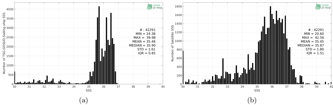
Figure 2: Histograms of SSS from TSG-GOSUD-Sailing-ship (a) and SMAP-L2-JPL-V4.3 (b) considering all match-up pairs per bins of 0.1 over the North Atlantic Ocean Pi-MEP region and for the full satellite product period.
