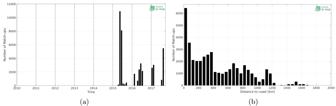
Figure 1: Number of match-ups between TSG-GOSUD-Sailing-ship and SMAP-L2-JPL-V4.3 SSS as a function of time (a) and as function of the distance to coast (b) over the North Atlantic Ocean Pi-MEP region and for the full satellite product period.
