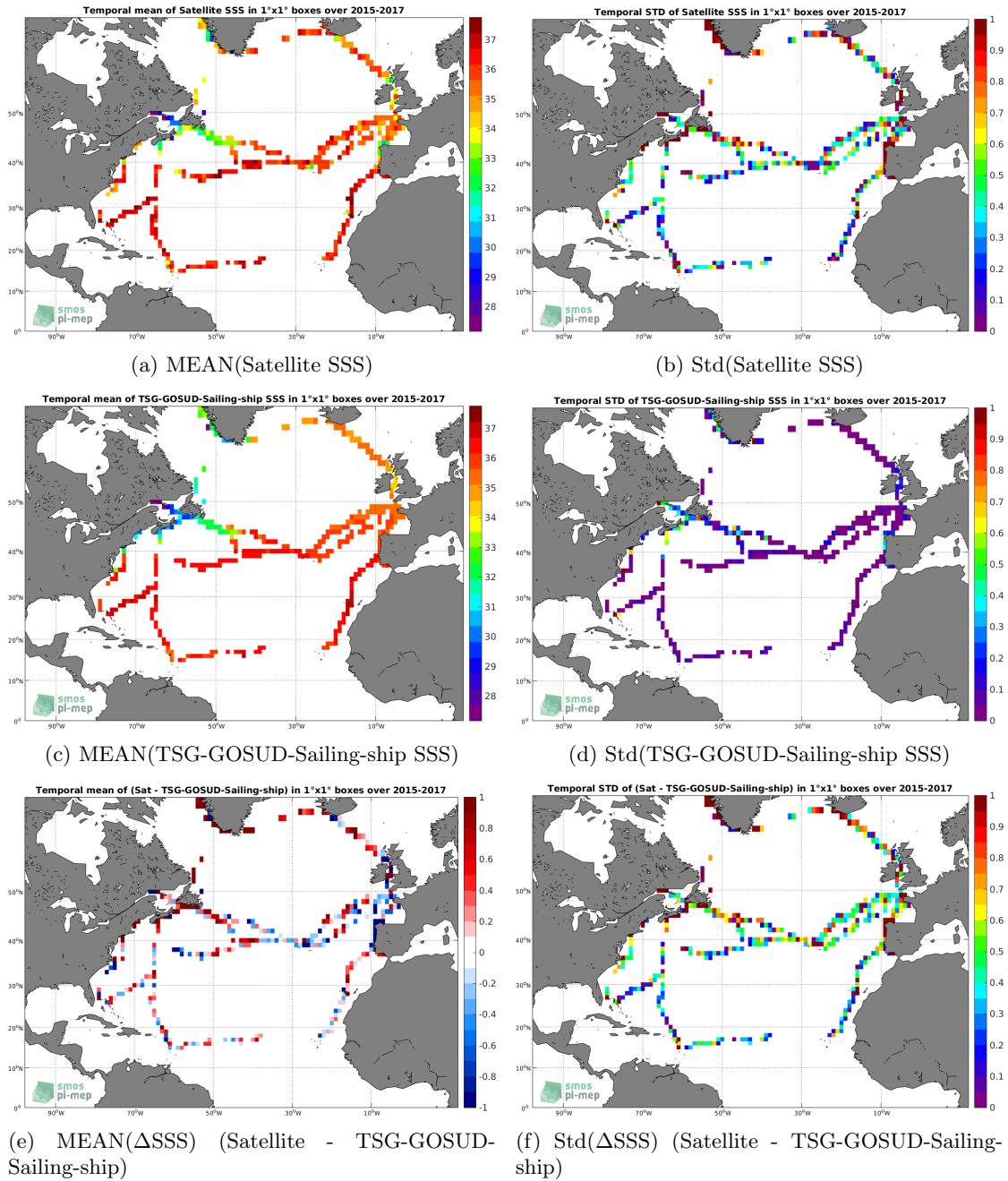
Figure 6: Temporal mean (left) and Std (right) of SSS from SMAP-L2-JPL-V4.3 (top), TSG-GOSUD-Sailing-ship (middle), and of \Delta SSS (Satellite - TSG-GOSUD-Sailing-ship). Only match-up pairs are used to generate these maps.
