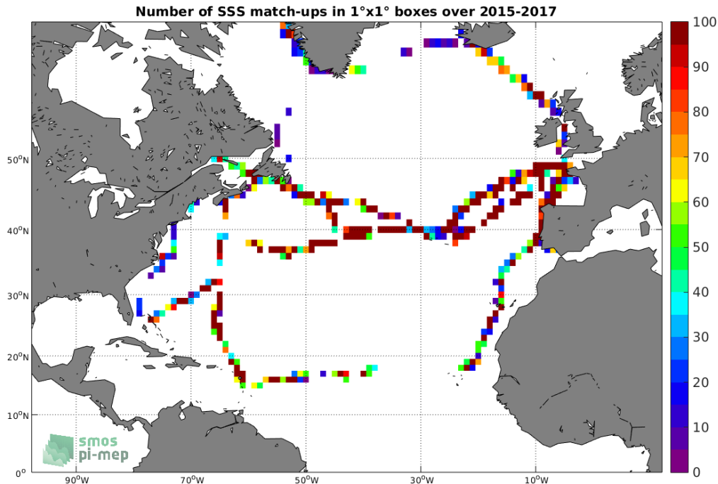
Figure 4: Number of SSS match-ups between TSG-GOSUD-Sailing-ship SSS and the SMAP-L2-JPL-V4.3 SSS product for the North Atlantic Ocean Pi-MEP region over 1°x1° boxes and for the full satellite product period.
