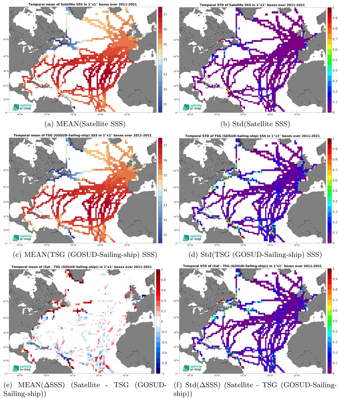
Figure 7: Temporal mean (left) and Std (right) of SSS from ISAS v7 - Monthly (Ifremer-LOPS-CMEMS) (top), TSG (GOSUD-Sailing-ship) (middle), and of \Delta SSS (Satellite - TSG (GOSUD-Sailing-ship)). Only match-up pairs are used to generate these maps.
