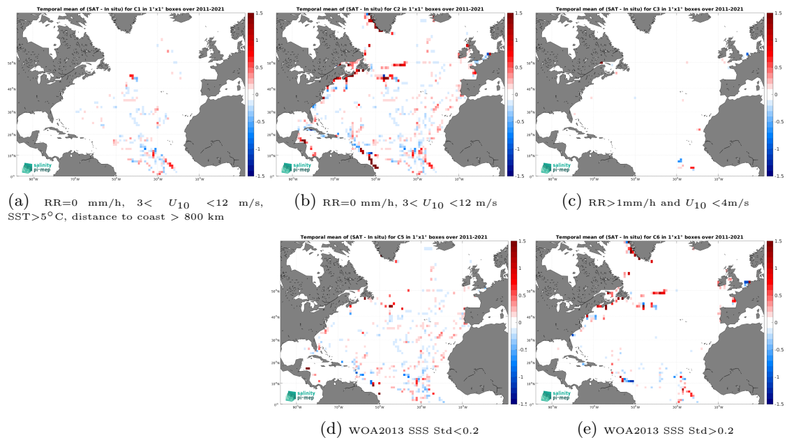
Figure 14: Temporal mean gridded over spatial boxes of size 1^\circ \times 1^\circ of \Delta\text{SSS} (ISAS v7 - Monthly (Ifremer-LOPS-CMEMS) - TSG (GOSUD-Sailing-ship)) for 5 different subdatasets corresponding to:RR=0 mm/h, 3 < U_{10} < 12 m/s, SST>5°C, distance to coast > 800 km (a), RR=0 mm/h, 3 < U_{10} < 12 m/s (b), RR>1mm/h and U_{10} < 4 m/s (c), WOA2013 SSS Std<0.2 (d), WOA2013 SSS Std>0.2 (e).
