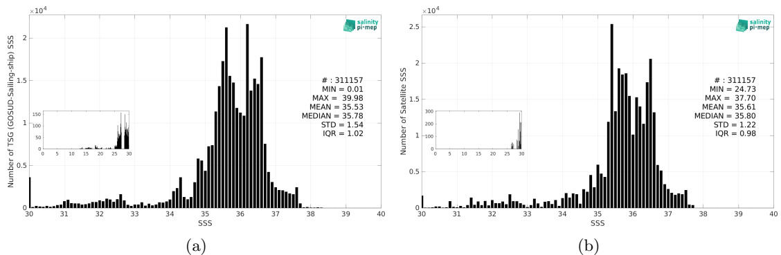
Figure 3: Histograms of SSS from TSG (GOSUD-Sailing-ship) (a) and ISAS v7 - Monthly (Ifremer-LOPS-CMEMS) (b) considering all match-up pairs per bins of 0.1 over the North Atlantic Ocean Pi-MEP region and for the full satellite product period.
