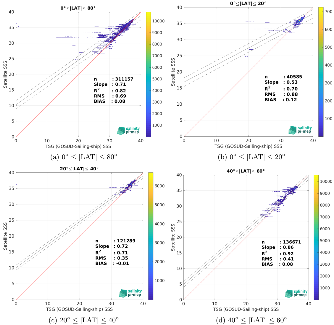
Figure 10: Contour maps of the concentration of ISAS v7 - Monthly (Ifremer-LOPS-CMEMS) SSS (y-axis) versus TSG (GOSUD-Sailing-ship) SSS (x-axis) at match-up pairs for different latitude bands. For each plot, the red line shows x=y . The black thin and dashed lines indicate a linear fit through the data cloud and the \pm 95\% confidence levels, respectively. The number match-up pairs n , the slope and R^2 coefficient of the linear fit, the root mean square (RMS) and the mean bias between satellite and in situ data are indicated for each latitude band in each plots.
