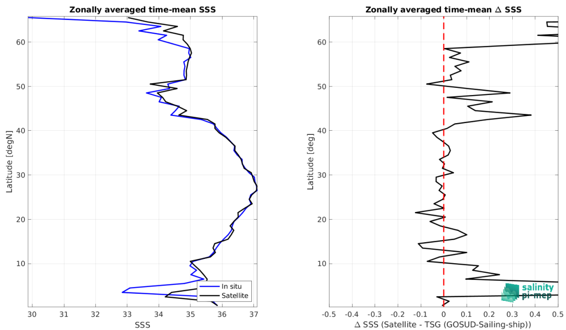
Figure 9: Left panel: Zonal mean SSS from ISAS v7 - Monthly (Ifremer-LOPS-CMEMS) satellite product (black) and from TSG (GOSUD-Sailing-ship) (blue). Right panel: Zonal mean of \Delta SSS (Satellite - TSG (GOSUD-Sailing-ship)) for all the collected Pi-MEP match-up pairs estimated over the full satellite product period.
