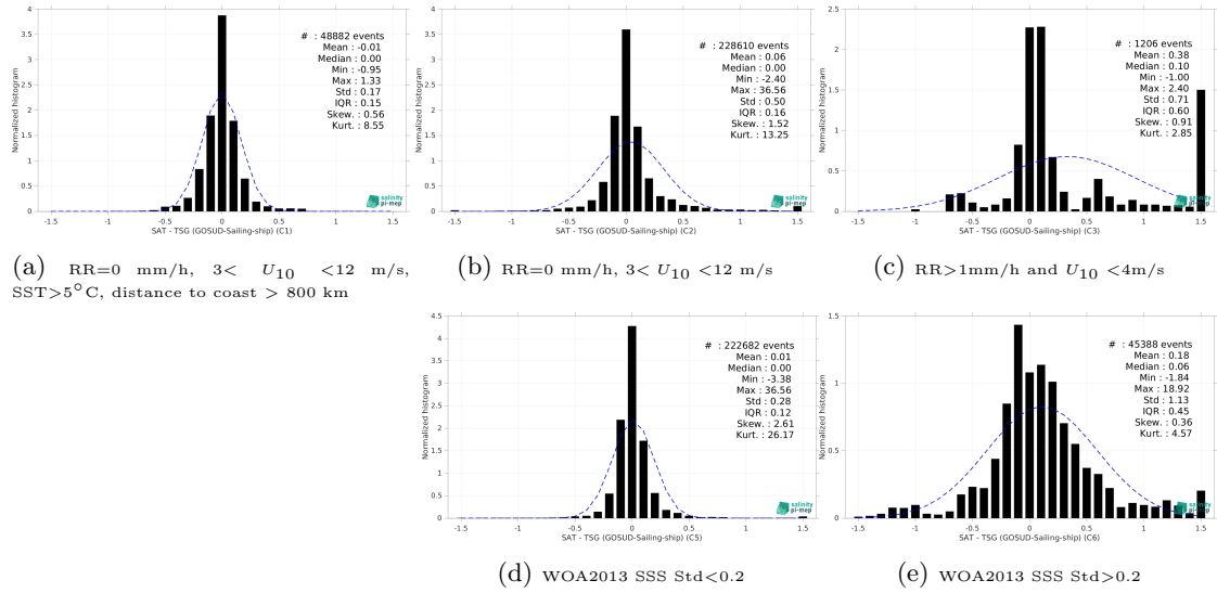
Figure 15: Normalized histogram of \Delta SSS (ISAS v7 - Monthly (Ifremer-LOPS-CMEMS) - TSG (GOSUD-Sailing-ship)) for 5 different subdatasets corresponding to: RR=0 mm/h, 3 < U_{10} < 12 m/s, SST>5°C, distance to coast > 800 km (a), RR=0 mm/h, 3 < U_{10} < 12 m/s (b), RR>1mm/h and U_{10} < 4 m/s (c), WOA2013 SSS Std<0.2 (d), WOA2013 SSS Std>0.2 (e).
