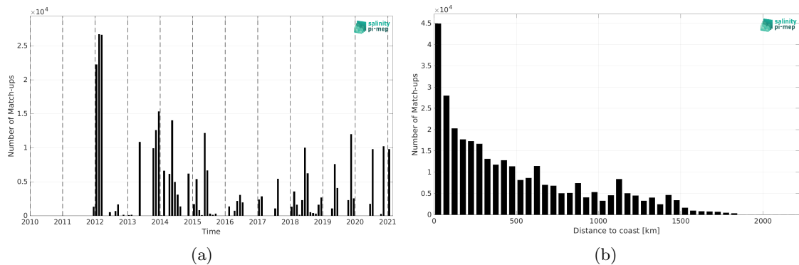
Figure 2: Number of match-ups between TSG (GOSUD-Sailing-ship) and ISAS v7 - Monthly (Ifremer-LOPS-CMEMS) SSS as a function of time (a) and as function of the distance to coast (b) over the North Atlantic Ocean Pi-MEP region and for the full satellite product period.
