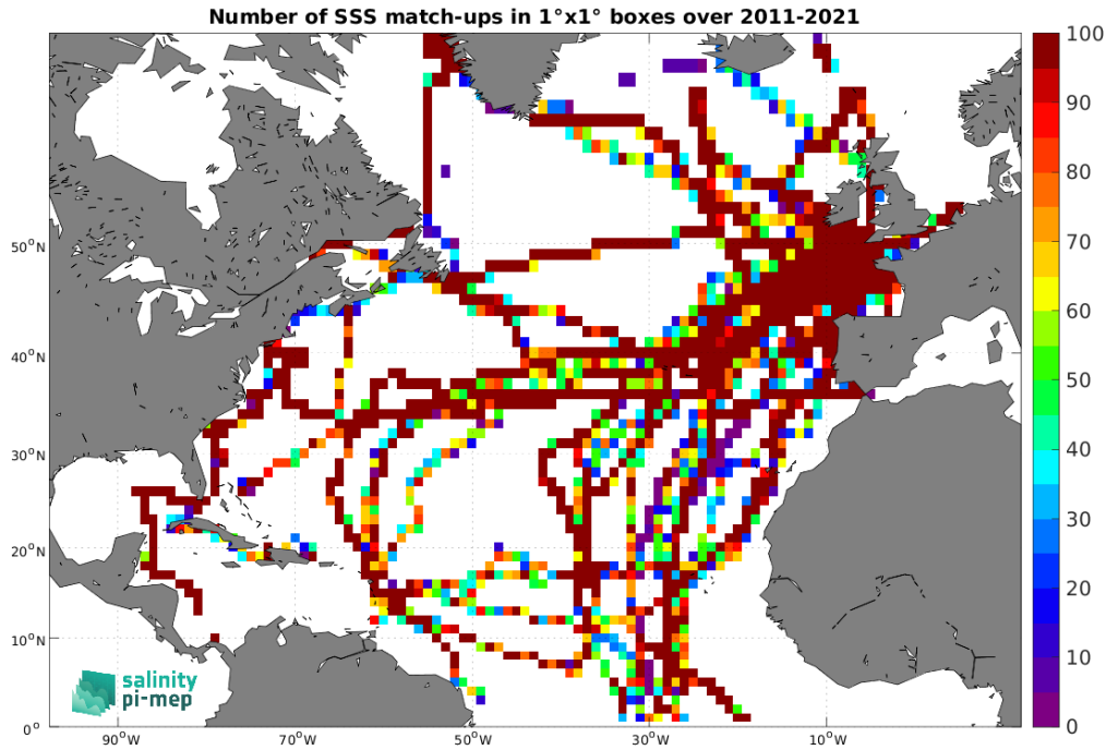
Figure 5: Number of SSS match-ups between TSG (GOSUD-Sailing-ship) SSS and the ISAS v7 - Monthly (Ifremer-LOPS-CMEMS) SSS product for the North Atlantic Ocean Pi-MEP region over 1^\circ \times 1^\circ boxes and for the full satellite product period.
