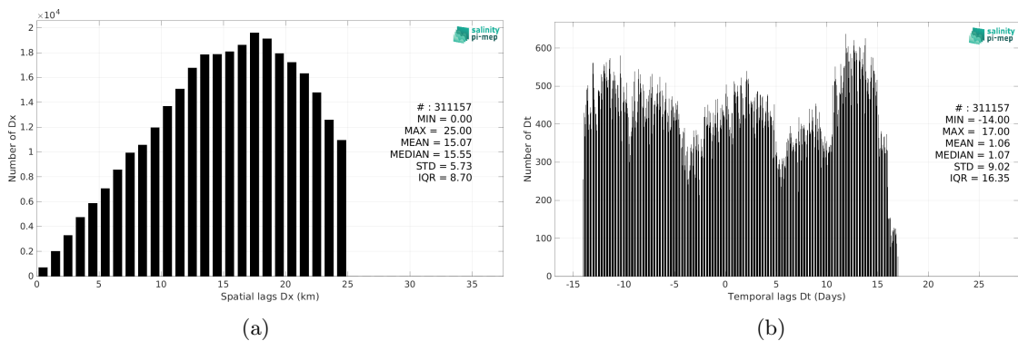
Figure 6: Histograms of the spatial (a) and temporal (b) lags between the location/time of the TSG (GOSUD-Sailing-ship) measurement and the date of the corresponding ISAS v7 - Monthly (Ifremer-LOPS-CMEMS) SSS pixel.
